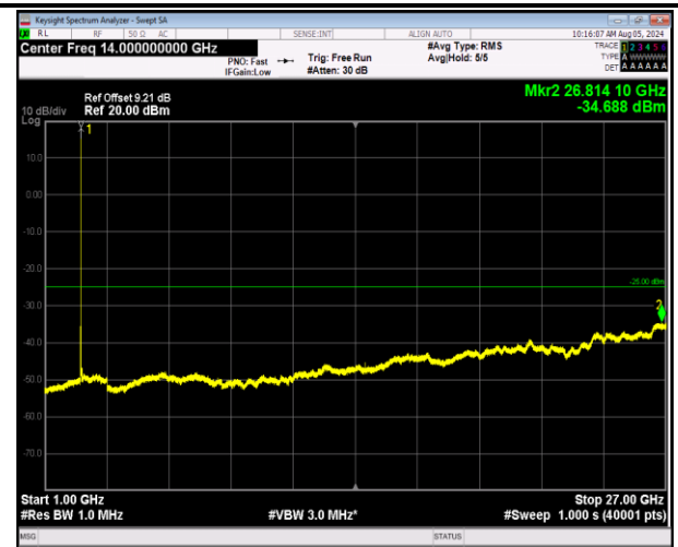
7-7-20MHz-20MHz-64QAM-64QAM-20850-21048-1RB#99- ORB#0-1000~27000MHz-PASS
