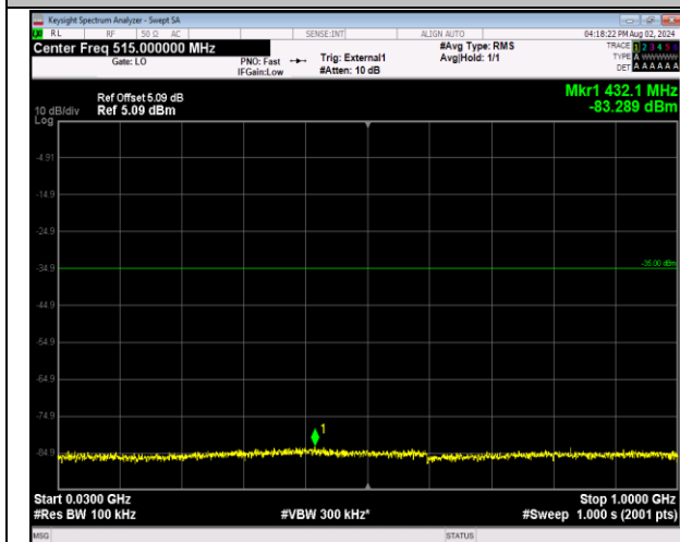
41-41-5MHz-20MHz-64QAM-64QAM-39683-39800-25RB #0-100RB#0-30~1000MHz-PASS
