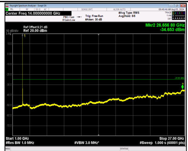
7-7-20MHz-10MHz-64QAM-64QAM-21051-21195-1RB#0-0 RB#0-1000~27000MHz-PASS
