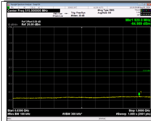
7-7-20MHz-20MHz-64QAM-64QAM-21001-21199-100RB#0-100RB#0-30~1000MHz-PASS
