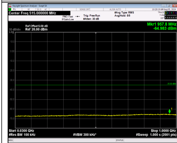
7-7-20MHz-20MHz-64QAM-64QAM-21152-21350-1RB#0-0RB#0-30~1000MHz-PASS
