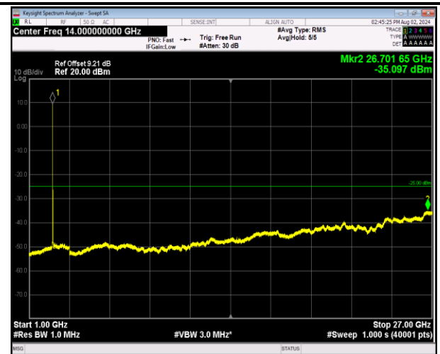
7-7-10MHz-20MHz-64QAM-64QAM-21006-21150-50RB#0- 100RB#0-1000~27000MHz-PASS
