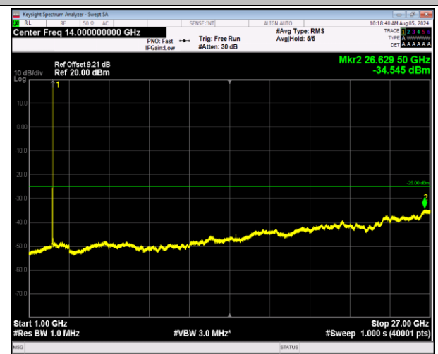
7-7-20MHz-20MHz-64QAM-64QAM-21001-21199-1RB#99- ORB#0-1000~27000MHz-PASS
