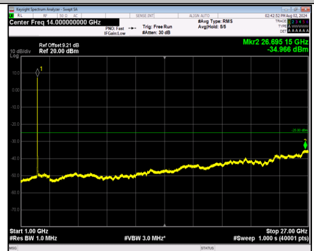
7-7-10MHz-20MHz-64QAM-64QAM-20805-20949-50RB#0- 100RB#0-1000~27000MHz-PASS
