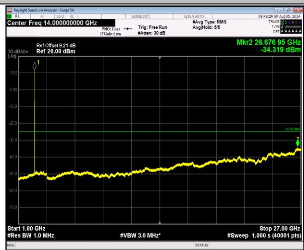
7-7-20MHz-10MHz-64QAM-64QAM-20850-20994-1RB#0-1 RB#49-1000~27000MHz-PASS
