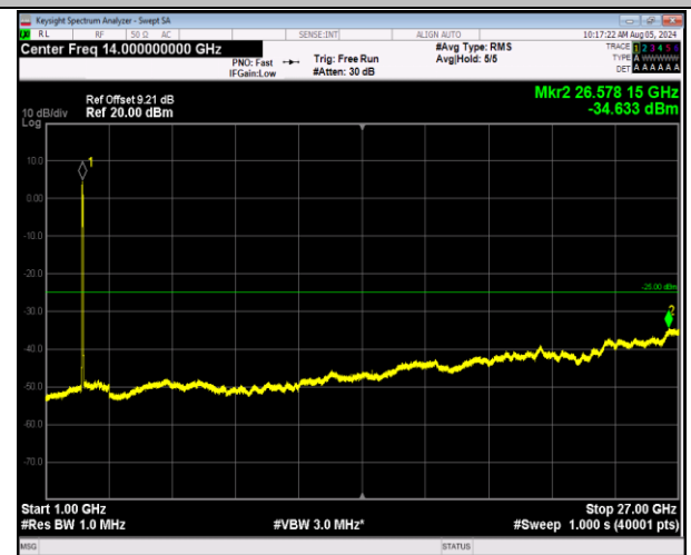
7-7-20MHz-20MHz-64QAM-64QAM-20850-21048-100RB#0 -100RB#0-1000~27000MHz-PASS
