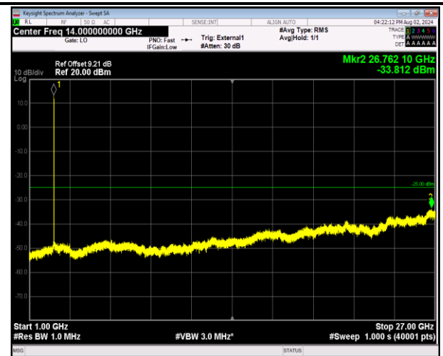
41-41-5MHz-20MHz-64QAM-64QAM-40528-40645-25RB#0 -100RB#0-1000~27000MHz-PASS
