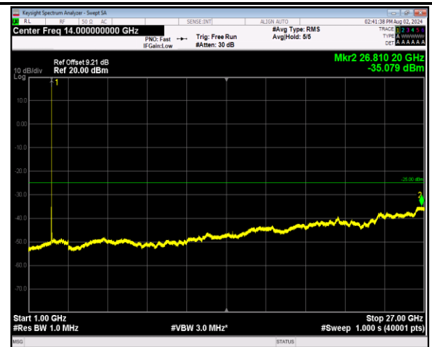
7-7-10MHz-20MHz-64QAM-64QAM-20805-20949-1RB#49- 0RB#0-1000~27000MHz-PASS
