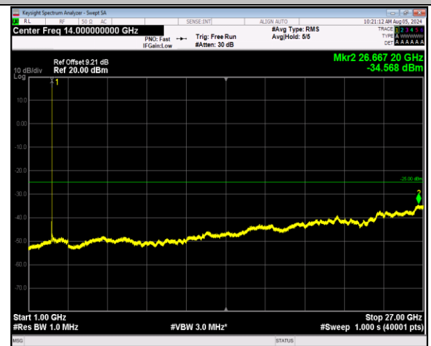
7-7-20MHz-20MHz-64QAM-64QAM-21152-21350-1RB#99-0RB#0-1000~27000MHz-PASS
