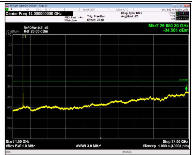
7-7-20MHz-20MHz-64QAM-64QAM-21001-21199-1RB#0-0 RB#0-1000~27000MHz-PASS
