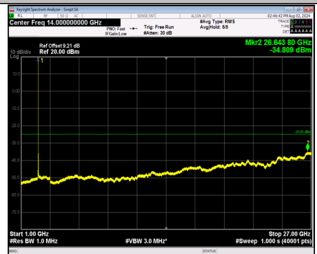
7-7-10MHz-20MHz-64QAM-64QAM-21206-21350-1RB#49- 9-0RB#0-1000~27000MHz-PASS
