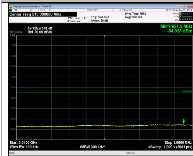
7-7-20MHz-10MHz-64QAM-64QAM-21251-21395-1RB#0 -0RB#0-30~1000MHz-PASS
