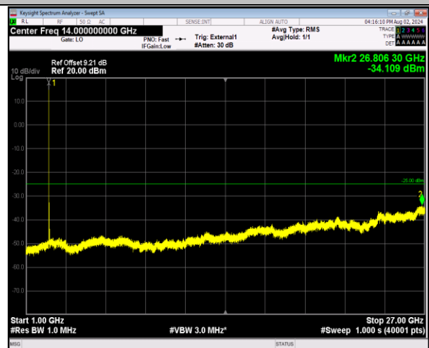
41-41-5MHz-20MHz-64QAM-64QAM-39683-39800-1RB#0- 0RB#0-1000~27000MHz-PASS
