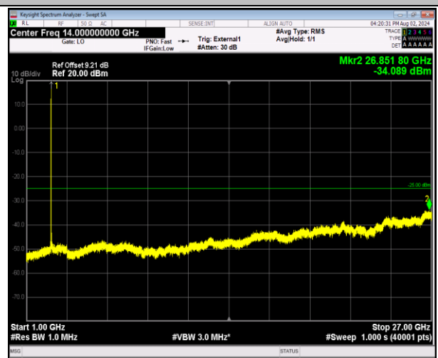
41-41-5MHz-20MHz-64QAM-64QAM-40528-40645-1RB#24 -0RB#0-1000~27000MHz-PASS
