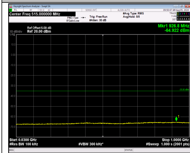
7-7-20MHz-10MHz-64QAM-64QAM-21051-21195-1RB#9 9-ORB#0-30~1000MHz-PASS
