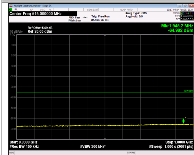
7-7-20MHz-20MHz-64QAM-64QAM-20850-21048-100RB #0-100RB#0-30~1000MHz-PASS
