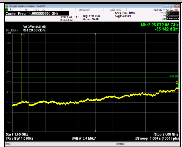
7-7-10MHz-20MHz-64QAM-64QAM-21006-21150-1RB#49- ORB#0-1000~27000MHz-PASS
