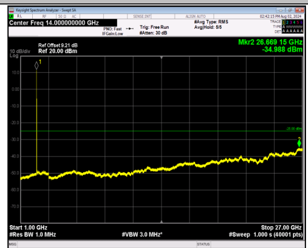
7-7-10MHz-20MHz-64QAM-64QAM-20805-20949-1RB#0-1 RB#99-1000~27000MHz-PASS
