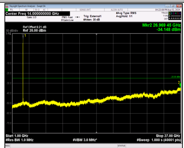
41-41-5MHz-20MHz-64QAM-64QAM-41373-41490-1RB#0- 0RB#0-1000~27000MHz-PASS
