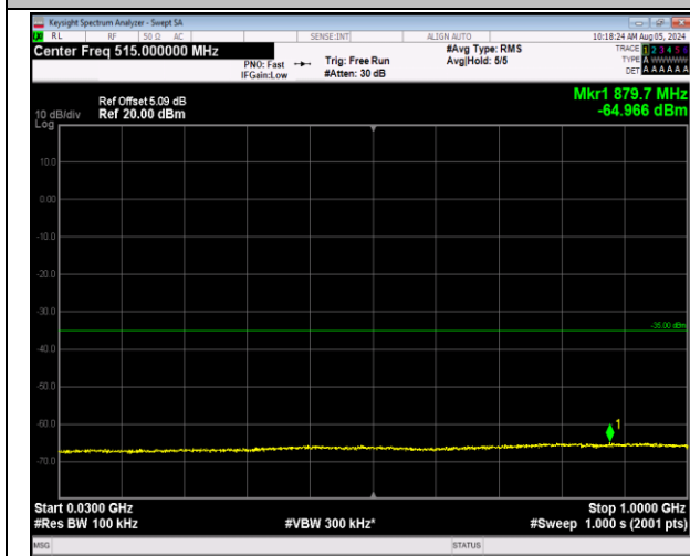
7-7-20MHz-20MHz-64QAM-64QAM-21001-21199-1RB#9 9-ORB#0-30~1000MHz-PASS
