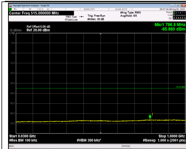
7-7-20MHz-10MHz-64QAM-64QAM-20850-20994-1RB#9 9-ORB#0-30~1000MHz-PASS
