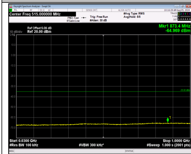
7-7-20MHz-20MHz-64QAM-64QAM-20850-21048-1RB#0 -1RB#99-30~1000MHz-PASS
