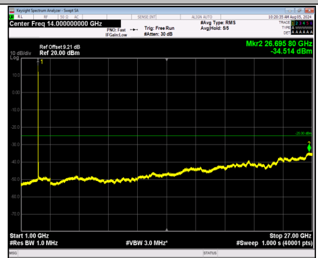
7-7-20MHz-20MHz-64QAM-64QAM-21152-21350-1RB#0-0RB#0-1000~27000MHz-PASS
