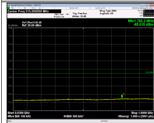
7-7-20MHz-10MHz-64QAM-64QAM-21251-21395-100RB #0-50RB#0-30~1000MHz-PASS
