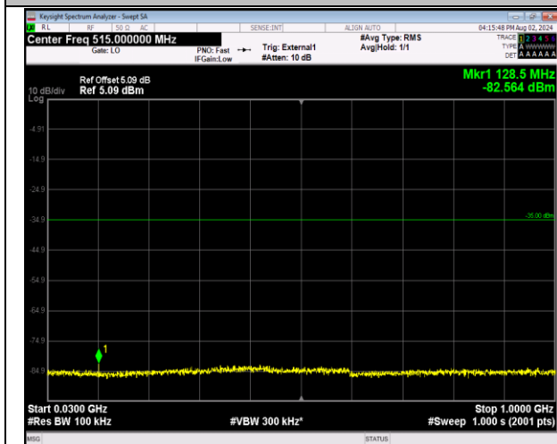
41-41-5MHz-20MHz-64QAM-64QAM-39683-39800-1RB# 0-0RB#0-30~1000MHz-PASS
