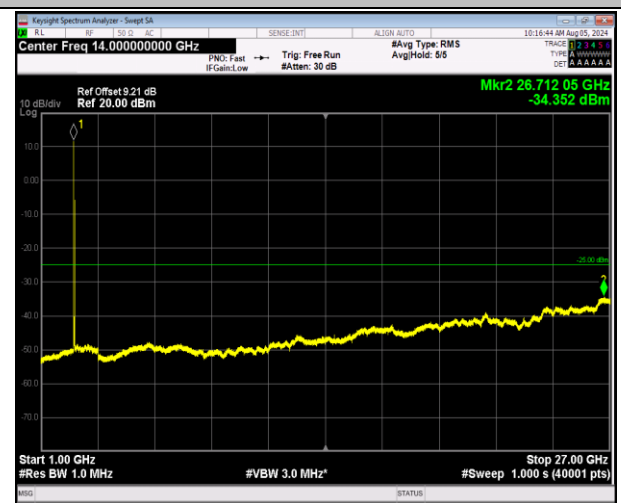
7-7-20MHz-20MHz-64QAM-64QAM-20850-21048-1RB#0-1 RB#99-1000~27000MHz-PASS
