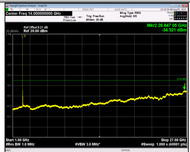
7-7-20MHz-20MHz-64QAM-64QAM-20850-21048-1RB#0-0 RB#0-1000~27000MHz-PASS
