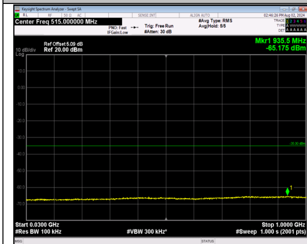
7-7-10MHz-20MHz-64QAM-64QAM-21206-21350-1RB#4 9-0RB#0-30~1000MHz-PASS
