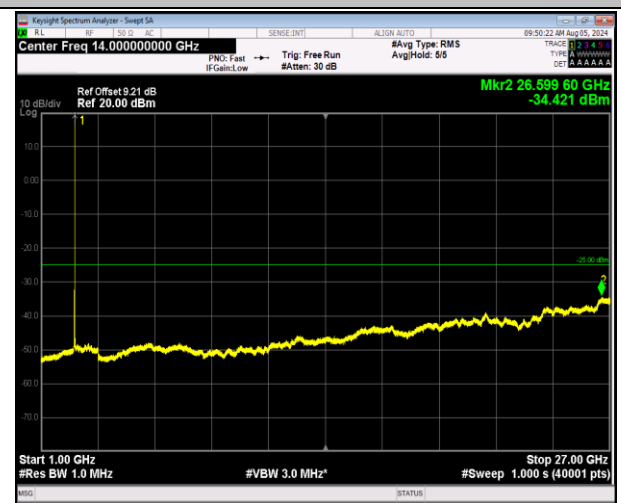
7-7-20MHz-10MHz-64QAM-64QAM-21051-21195-1RB#99- ORB#0-1000~27000MHz-PASS
