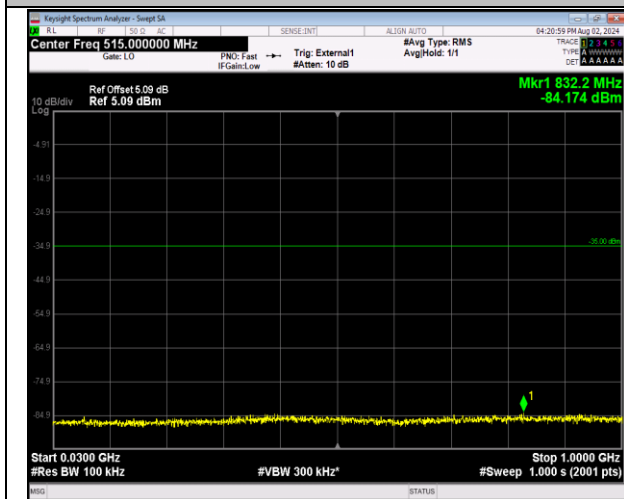
41-41-5MHz-20MHz-64QAM-64QAM-40528-40645-1RB# 0-1RB#99-30~1000MHz-PASS
