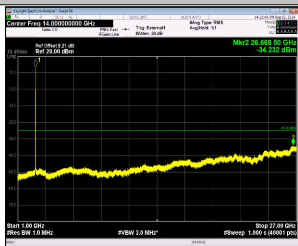
41-41-5MHz-20MHz-64QAM-64QAM-41373-41490-25RB#0 -100RB#0-1000~27000MHz-PASS
