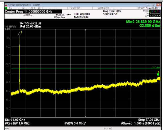
41-41-5MHz-20MHz-64QAM-64QAM-39683-39800-25RB#0 -100RB#0-1000~27000MHz-PASS
