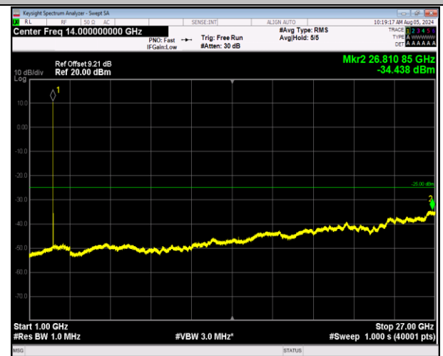
7-7-20MHz-20MHz-64QAM-64QAM-21001-21199-1RB#0-1 RB#99-1000~27000MHz-PASS
