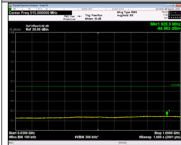
7-7-20MHz-20MHz-64QAM-64QAM-21001-21199-1RB#0 -1RB#99-30~1000MHz-PASS
