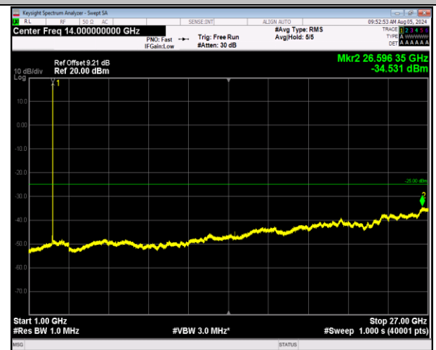
7-7-20MHz-10MHz-64QAM-64QAM-21251-21395-1RB#99- 0RB#0-1000~27000MHz-PASS
