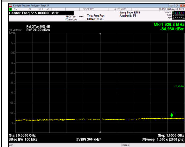
7-7-20MHz-20MHz-64QAM-64QAM-20850-21048-1RB#0 -0RB#0-30~1000MHz-PASS
