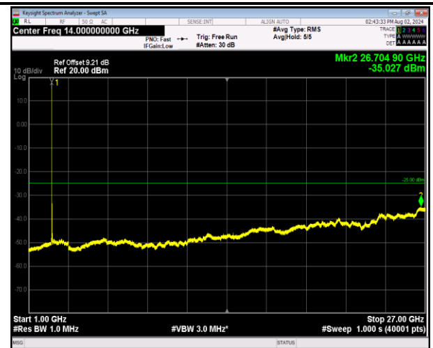
7-7-10MHz-20MHz-64QAM-64QAM-21006-21150-1RB#0-0 RB#0-1000~27000MHz-PASS
