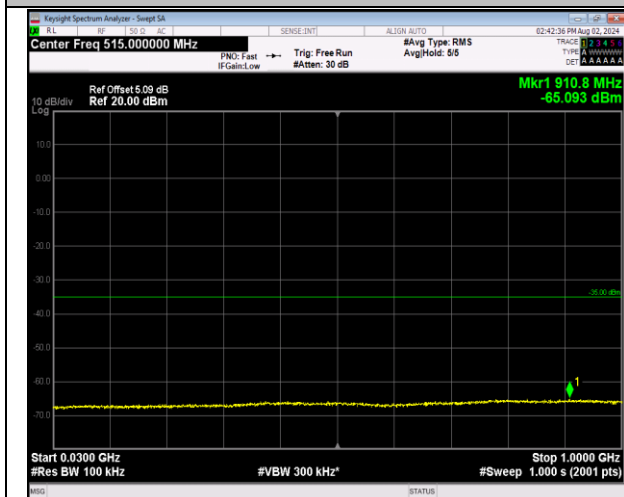
7-7-10MHz-20MHz-64QAM-64QAM-20805-20949-50RB# 0-100RB#0-30~1000MHz-PASS
