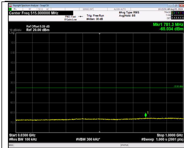
7-7-20MHz-20MHz-64QAM-64QAM-20850-21048-1RB#9 9-ORB#0-30~1000MHz-PASS
