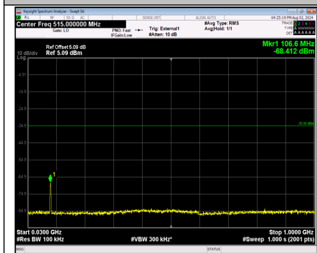
41-41-5MHz-20MHz-64QAM-64QAM-41373-41490-25RB #0-100RB#0-30~1000MHz-PASS
