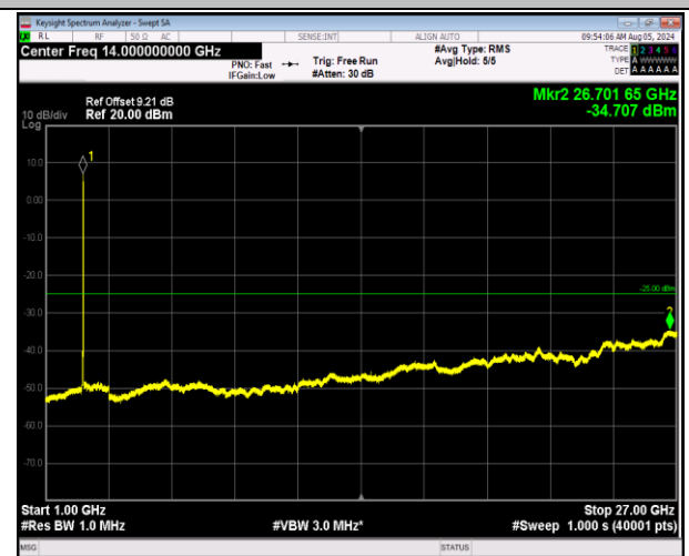
7-7-20MHz-10MHz-64QAM-64QAM-21251-21395-100RB#0 -50RB#0-1000~27000MHz-PASS
