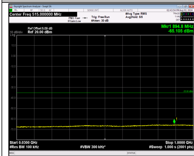
7-7-10MHz-20MHz-64QAM-64QAM-21006-21150-1RB#4 9-ORB#0-30~1000MHz-PASS
