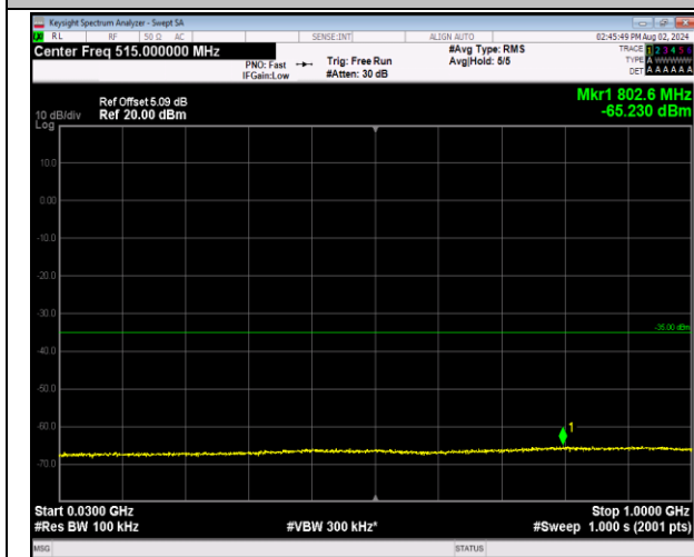
7-7-10MHz-20MHz-64QAM-64QAM-21206-21350-1RB#0 -0RB#0-30~1000MHz-PASS
