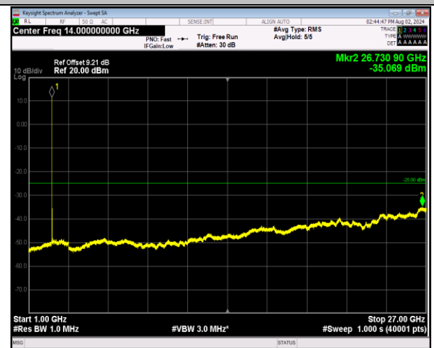
7-7-10MHz-20MHz-64QAM-64QAM-21006-21150-1RB#0-1 RB#99-1000~27000MHz-PASS
