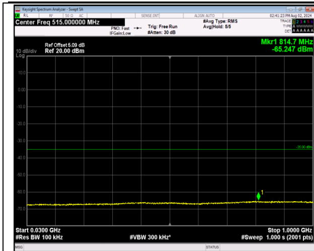
7-7-10MHz-20MHz-64QAM-64QAM-20805-20949-1RB#4 9-0RB#0-30~1000MHz-PASS
