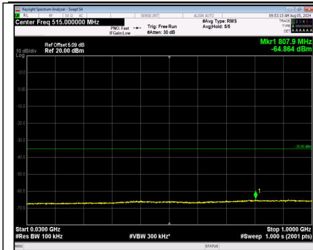
7-7-20MHz-10MHz-64QAM-64QAM-21251-21395-1RB#0 -1RB#49-30~1000MHz-PASS
