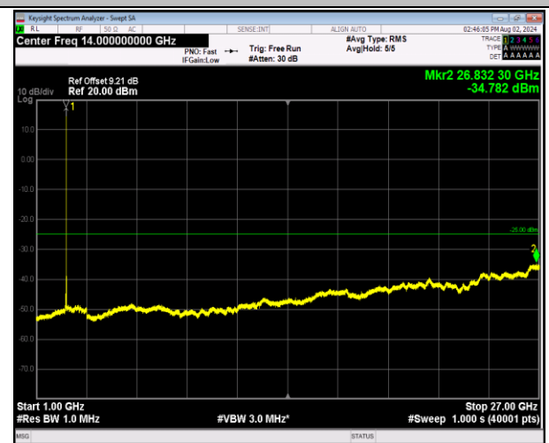
7-7-10MHz-20MHz-64QAM-64QAM-21206-21350-1RB#0-0 RB#0-1000~27000MHz-PASS
