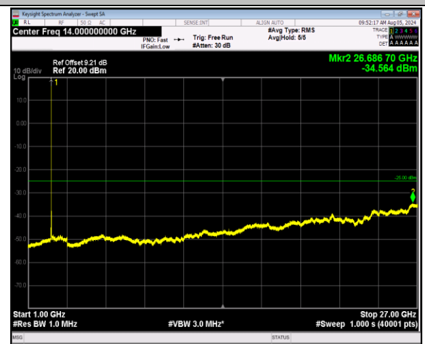
7-7-20MHz-10MHz-64QAM-64QAM-21251-21395-1RB#0-0 RB#0-1000~27000MHz-PASS
