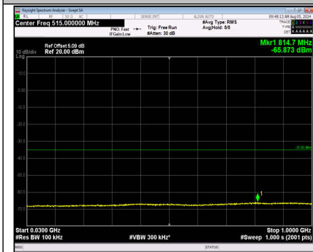
7-7-20MHz-10MHz-64QAM-64QAM-20850-20994-1RB#0 -1RB#49-30~1000MHz-PASS
