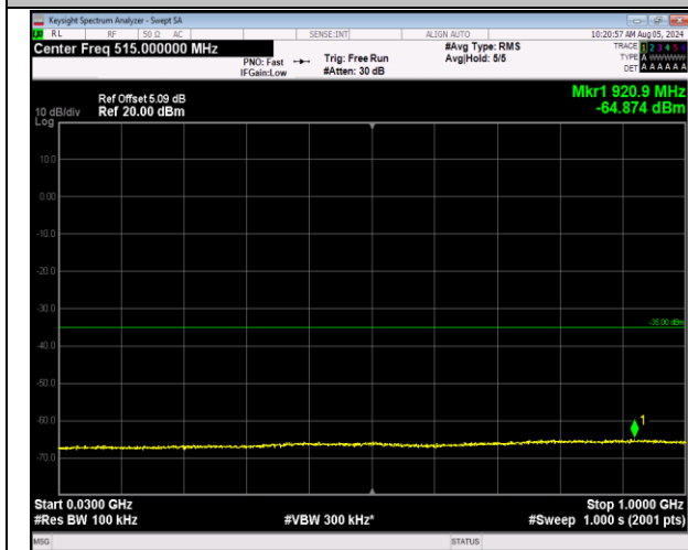
7-7-20MHz-20MHz-64QAM-64QAM-21152-21350-1RB#99-9-0RB#0-30~1000MHz-PASS
