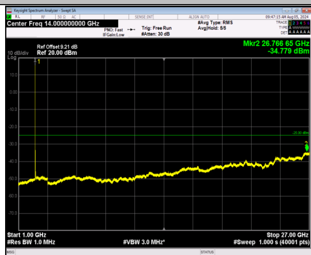
7-7-20MHz-10MHz-64QAM-64QAM-20850-20994-1RB#0-0 RB#0-1000~27000MHz-PASS
