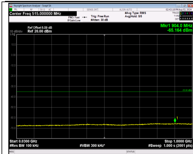
7-7-10MHz-20MHz-64QAM-64QAM-21006-21150-1RB#0 -ORB#0-30~1000MHz-PASS
