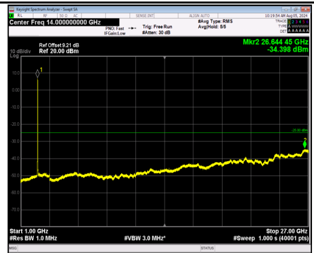
7-7-20MHz-20MHz-64QAM-64QAM-21001-21199-100RB#0-100RB#0-1000~27000MHz-PASS
