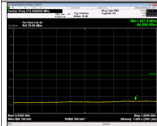
7-7-20MHz-10MHz-64QAM-64QAM-21251-21395-1RB#9 9-0RB#0-30~1000MHz-PASS
