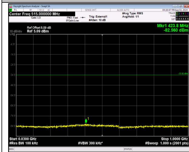
41-41-5MHz-20MHz-64QAM-64QAM-40528-40645-1RB# 24-0RB#0-30~1000MHz-PASS
