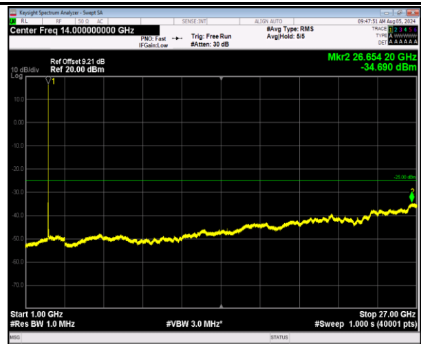
7-7-20MHz-10MHz-64QAM-64QAM-20850-20994-1RB#99- ORB#0-1000~27000MHz-PASS
