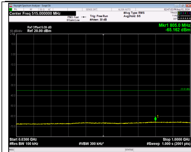
7-7-10MHz-20MHz-64QAM-64QAM-21206-21350-1RB#0 -1RB#99-30~1000MHz-PASS
