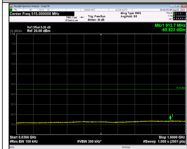
7-7-20MHz-10MHz-64QAM-64QAM-20850-20994-1RB#0 -0RB#0-30~1000MHz-PASS
