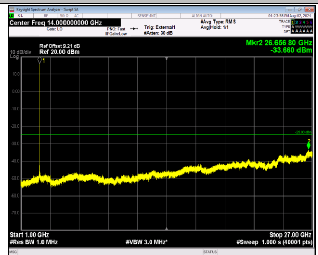
41-41-5MHz-20MHz-64QAM-64QAM-41373-41490-1RB#24 -0RB#0-1000~27000MHz-PASS
