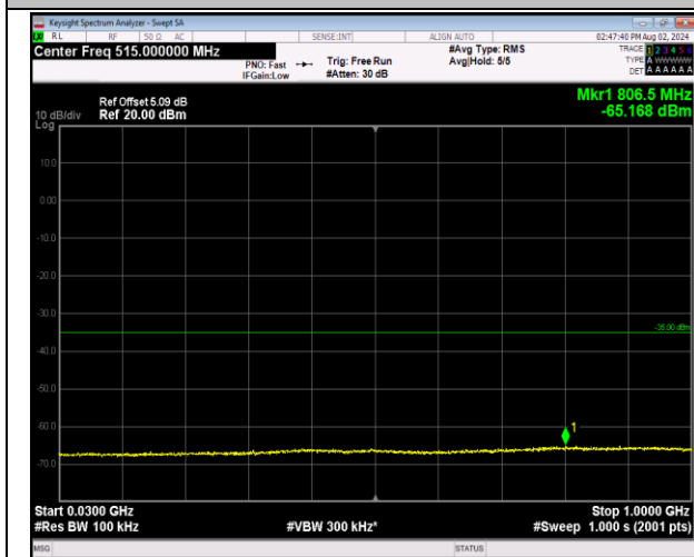
7-7-10MHz-20MHz-64QAM-64QAM-21206-21350-50RB# 0-100RB#0-30~1000MHz-PASS
