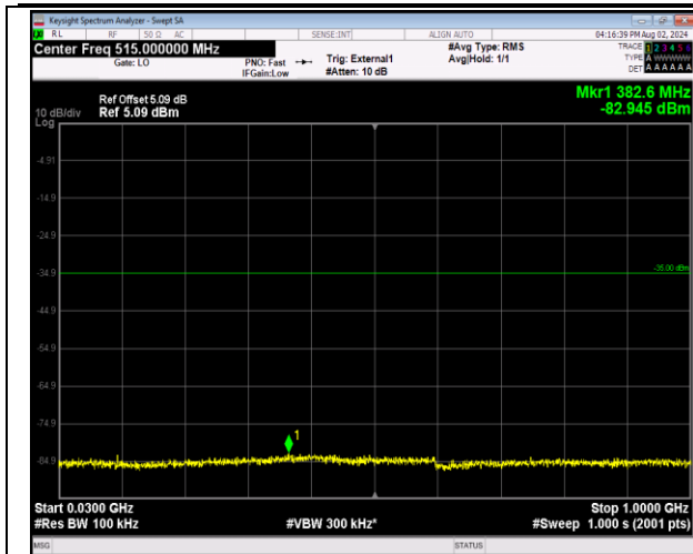
41-41-5MHz-20MHz-64QAM-64QAM-39683-39800-1RB# 24-0RB#0-30~1000MHz-PASS
