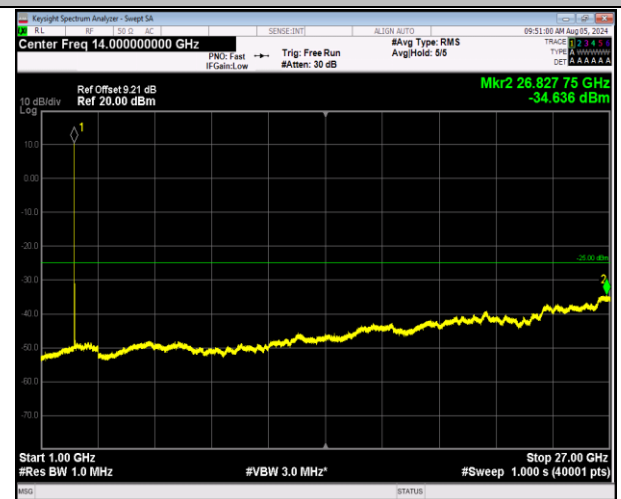
7-7-20MHz-10MHz-64QAM-64QAM-21051-21195-1RB#0-1 RB#49-1000~27000MHz-PASS
