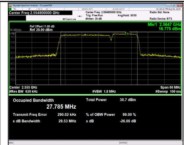
7-7-20MHz-10MHz-QPSK-QPSK-21251-21395-100RB#0-50RB#0-PASS
