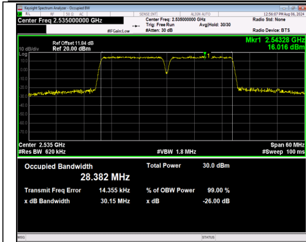
7-7-15MHz-15MHz-16QAM-16QAM-21025-21175-75RB#0 -75RB#0-PASS
