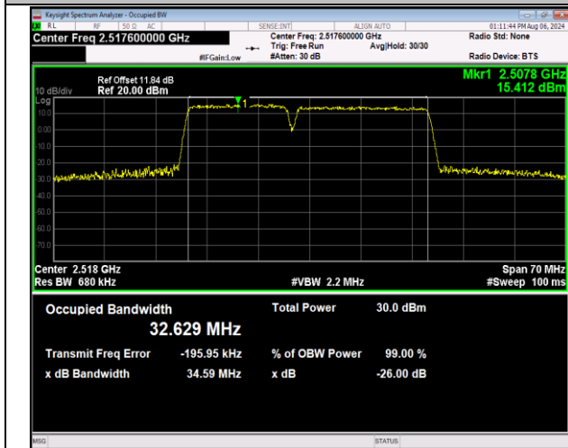
7-7-15MHz-20MHz-16QAM-16QAM-20828-20999-75RB#0 -100RB#0-PASS
