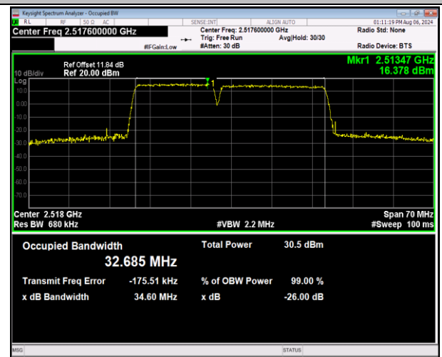
7-7-15MHz-20MHz-QPSK-QPSK-20828-20999-75RB#0-1 00RB#0-PASS
