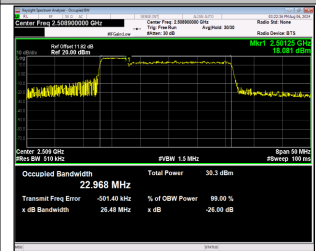
41-41-5MHz-20MHz-QPSK-QPSK-39683-39800-25RB#0-100RB#0-PASS
