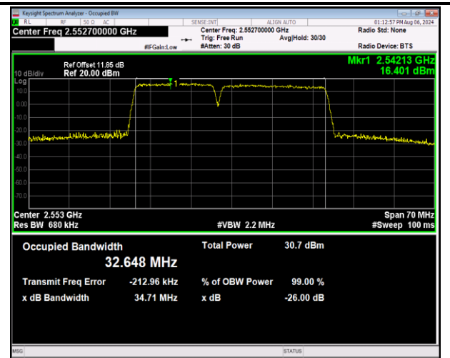
7-7-15MHz-20MHz-QPSK-QPSK-21179-21350-75RB#0-1 00RB#0-PASS
