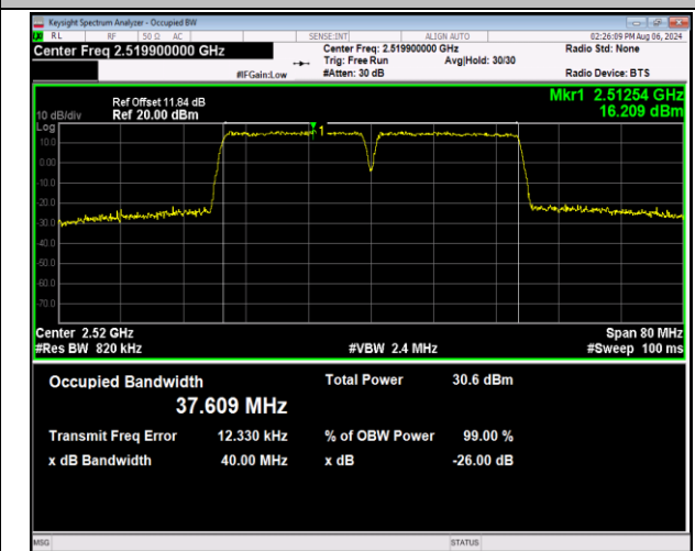
7-7-20MHz-20MHz-QPSK-QPSK-20850-21048-100RB#0-100RB#0-PASS
