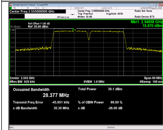
7-7-15MHz-15MHz-16QAM-16QAM-21225-21375-75RB#0 -75RB#0-PASS
