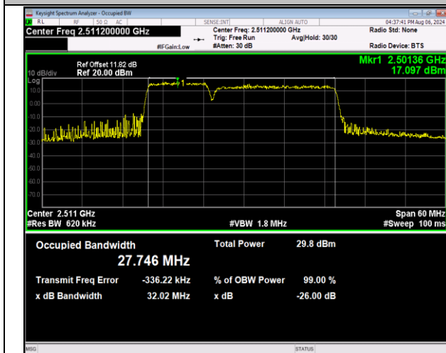
41-41-10MHz-20MHz-16QAM-16QAM-39705-39849-50RB #0-100RB#0-PASS
