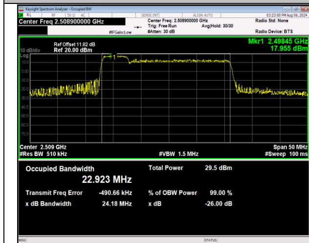
41-41-5MHz-20MHz-16QAM-16QAM-39683-39800-25RB#0-100RB#0-PASS
