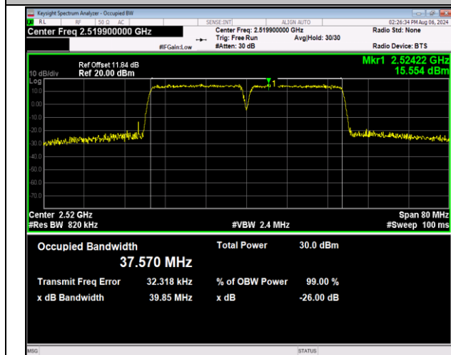
7-7-20MHz-20MHz-16QAM-16QAM-20850-21048-100RB#0-100RB#0-PASS
