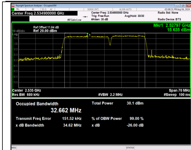
7-7-20MHz-15MHz-16QAM-16QAM-21026-21197-100RB#0-75RB#0-PASS
