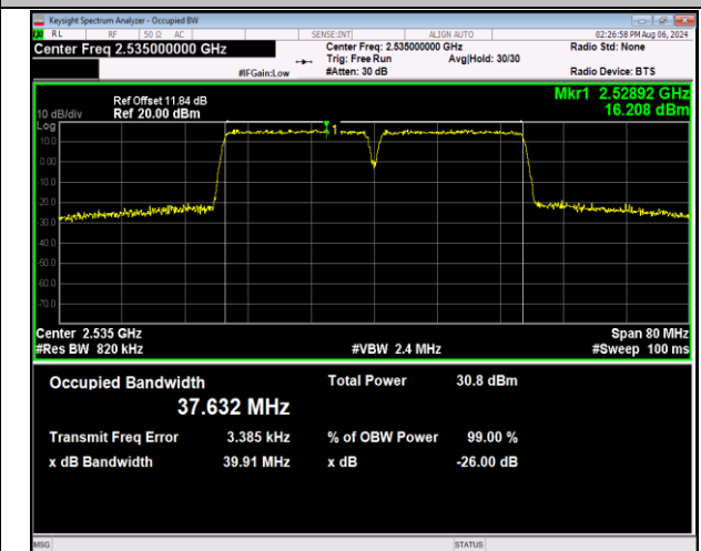
7-7-20MHz-20MHz-QPSK-QPSK-21001-21199-100RB#0-100RB#0-PASS
