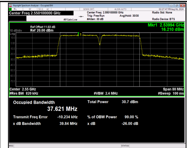
7-7-20MHz-20MHz-QPSK-QPSK-21152-21350-100RB#0-100RB#0-PASS
