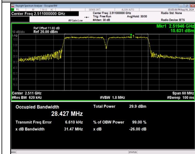
41-41-15MHz-15MHz-16QAM-16QAM-39725-39875-75RB #0-75RB#0-PASS
