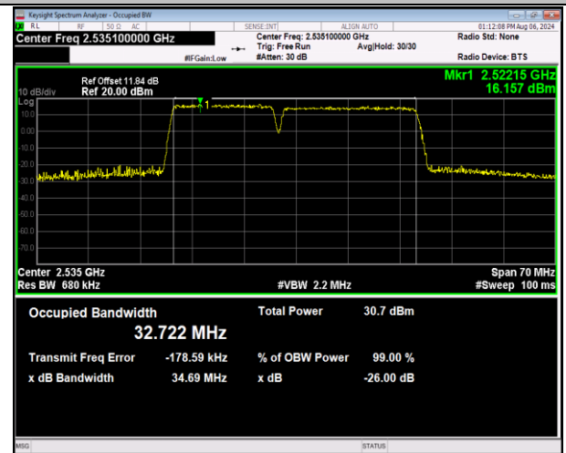
7-7-15MHz-20MHz-QPSK-QPSK-21003-21174-75RB#0-1 00RB#0-PASS
