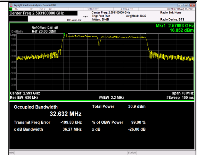
41-41-15MHz-20MHz-QPSK-QPSK-40523-40694-75RB#0 -100RB#0-PASS
