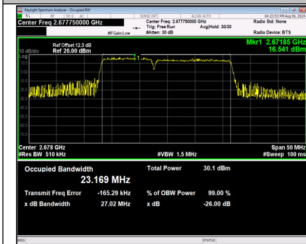
41-41-10MHz-15MHz-16QAM-16QAM-41395-41515-50RB #0-75RB#0-PASS
