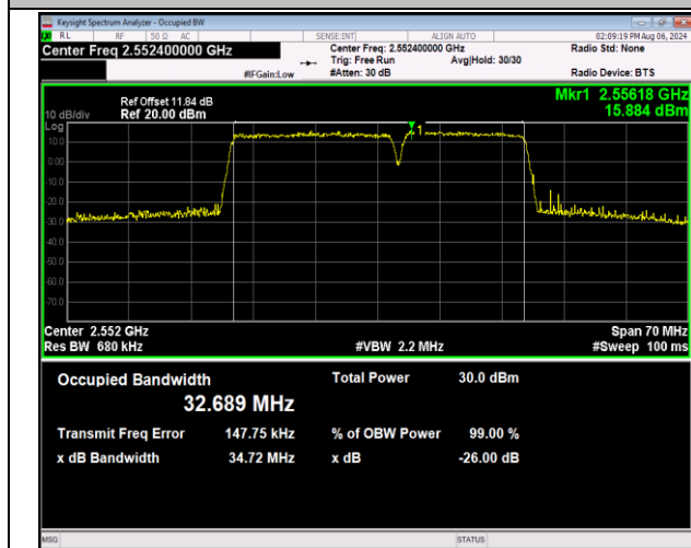
7-7-20MHz-15MHz-16QAM-16QAM-21201-21372-100RB#0-75RB#0-PASS
