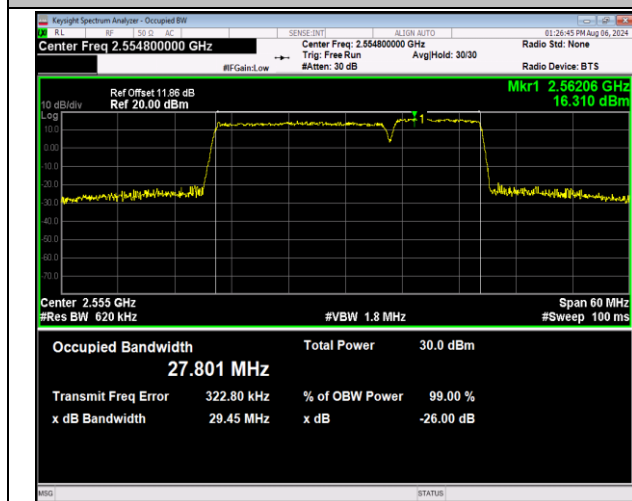
7-7-20MHz-10MHz-16QAM-16QAM-21251-21395-100RB#0-50RB#0-PASS
