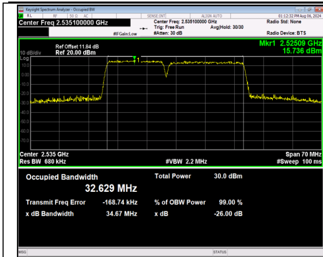
7-7-15MHz-20MHz-16QAM-16QAM-21003-21174-75RB#0 -100RB#0-PASS
