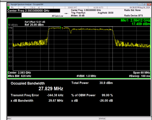
41-41-10MHz-20MHz-QPSK-QPSK-40526-40670-50RB#0 -100RB#0-PASS
