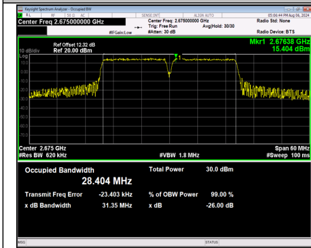
41-41-15MHz-15MHz-16QAM-16QAM-41365-41515-75RB #0-75RB#0-PASS
