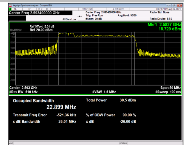
41-41-5MHz-20MHz-QPSK-QPSK-40528-40645-25RB#0-100RB#0-PASS
