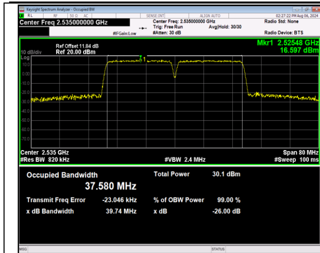
7-7-20MHz-20MHz-16QAM-16QAM-21001-21199-100RB#0-100RB#0-PASS
