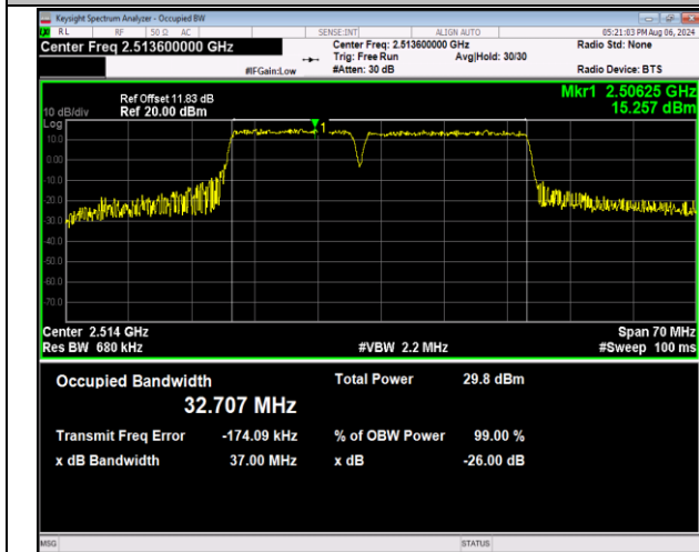
41-41-15MHz-20MHz-16QAM-16QAM-39728-39899-75RB #0-100RB#0-PASS
