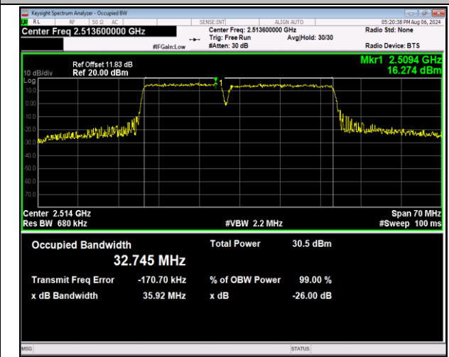
41-41-15MHz-20MHz-QPSK-QPSK-39728-39899-75RB#0 -100RB#0-PASS
