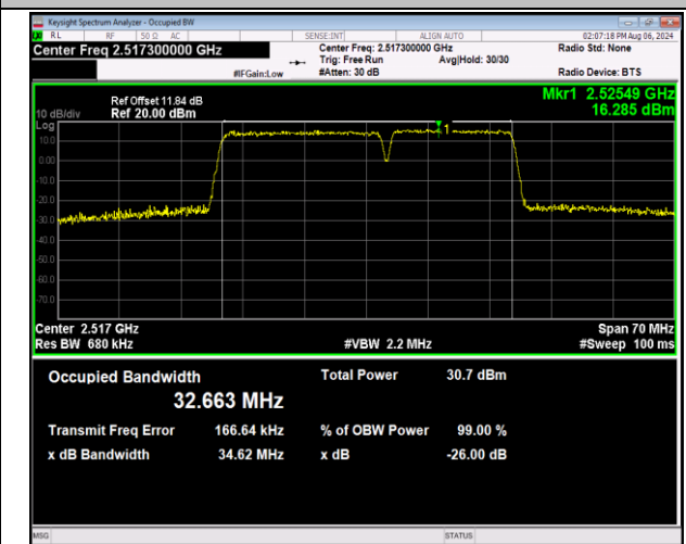
7-7-20MHz-15MHz-QPSK-QPSK-20850-21021-100RB#0-75RB#0-PASS
