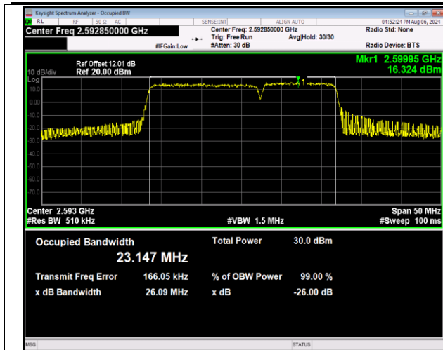
41-41-15MHz-10MHz-16QAM-16QAM-40571-40691-75RB #0-50RB#0-PASS
