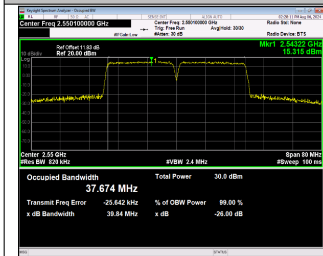
7-7-20MHz-20MHz-16QAM-16QAM-21152-21350-100RB#0-100RB#0-PASS
