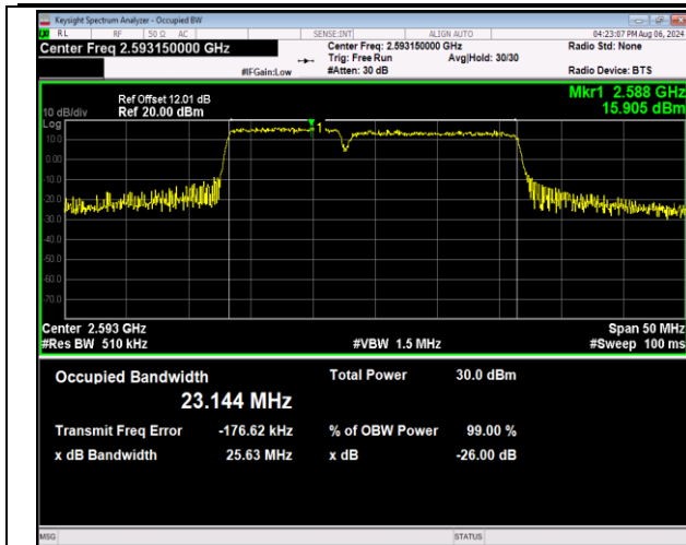
41-41-10MHz-15MHz-16QAM-16QAM-40549-40669-50RB #0-75RB#0-PASS
