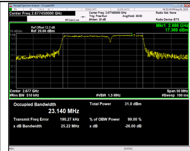
41-41-15MHz-10MHz-QPSK-QPSK-41417-41537-75RB#0 -50RB#0-PASS
