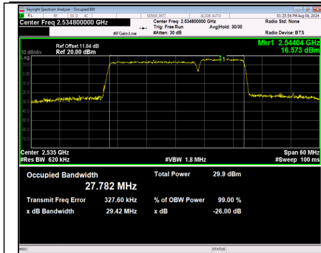
7-7-20MHz-10MHz-16QAM-16QAM-21051-21195-100RB#0-50RB#0-PASS
