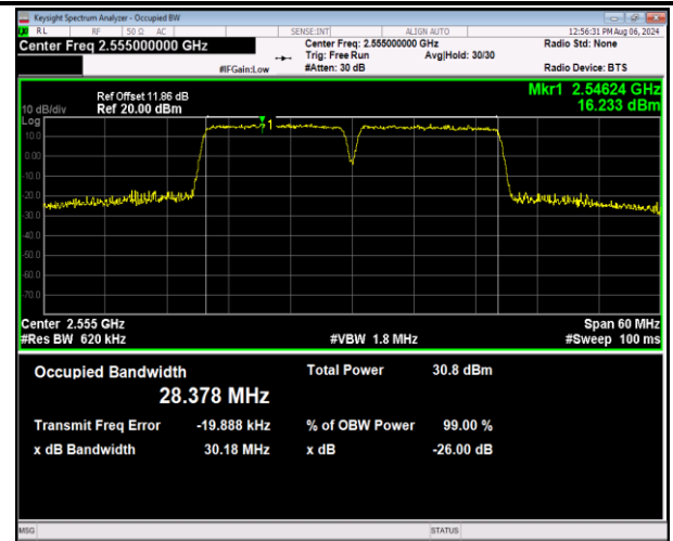
7-7-15MHz-15MHz-QPSK-QPSK-21225-21375-75RB#0-7 5RB#0-PASS
