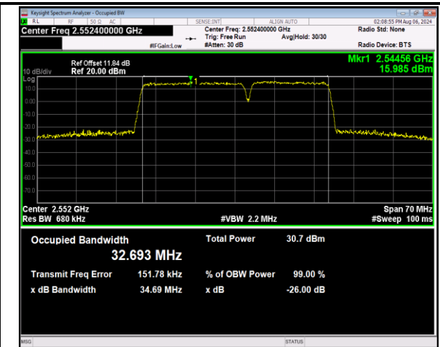
7-7-20MHz-15MHz-QPSK-QPSK-21201-21372-100RB#0-75RB#0-PASS
