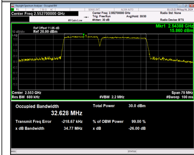
7-7-15MHz-20MHz-16QAM-16QAM-21179-21350-75RB#0 -100RB#0-PASS
