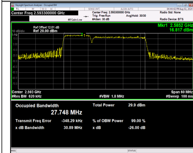
41-41-10MHz-20MHz-64QAM-64QAM-40526-40670-50RB #0-100RB#0-PASS
