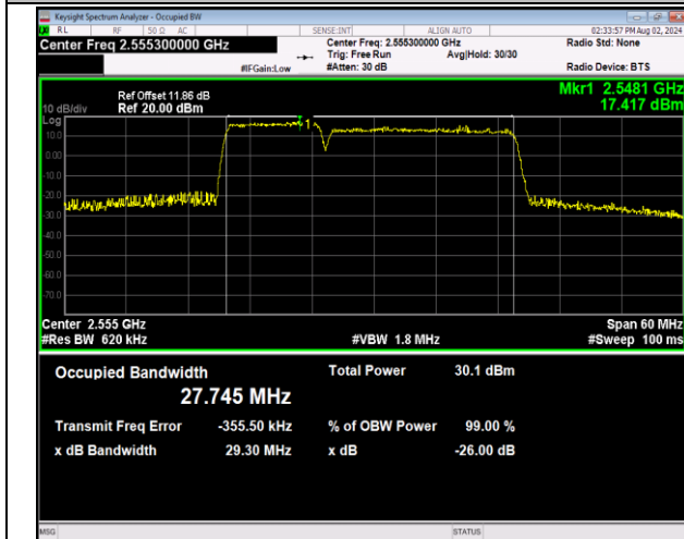
7-7-10MHz-20MHz-64QAM-64QAM-21206-21350-50RB#0 -100RB#0-PASS
