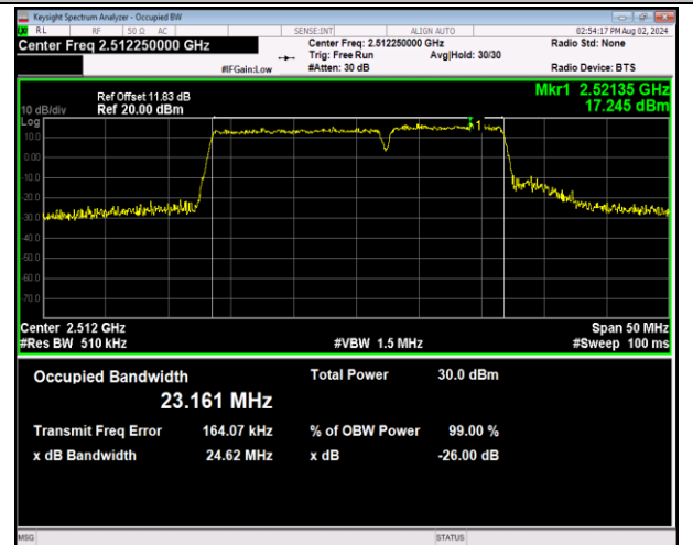
7-7-15MHz-10MHz-64QAM-64QAM-20825-20945-75RB#0 -50RB#0-PASS
