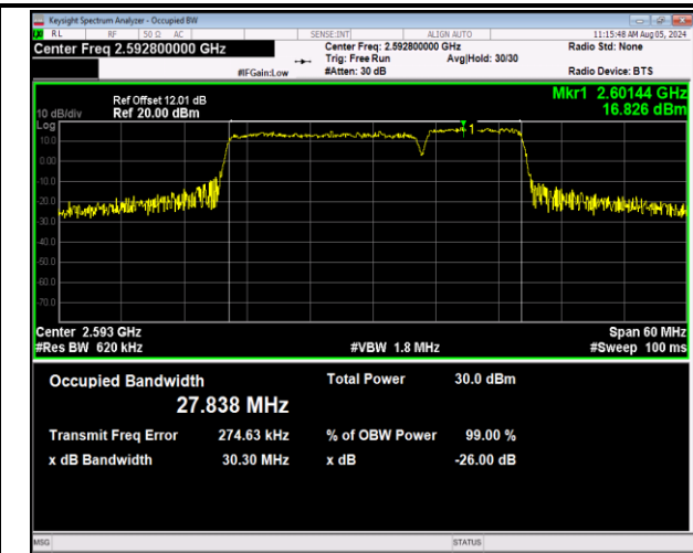
41-41-20MHz-10MHz-64QAM-64QAM-40571-40715-100R B#0-50RB#0-PASS
