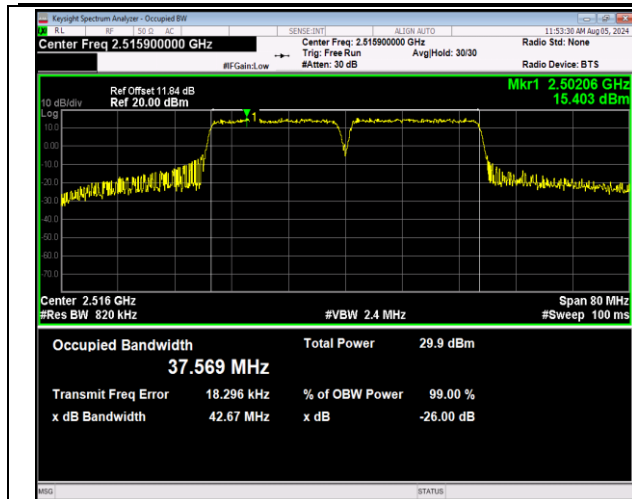
41-41-20MHz-20MHz-64QAM-64QAM-39750-39948-100R B#0-100RB#0-PASS
