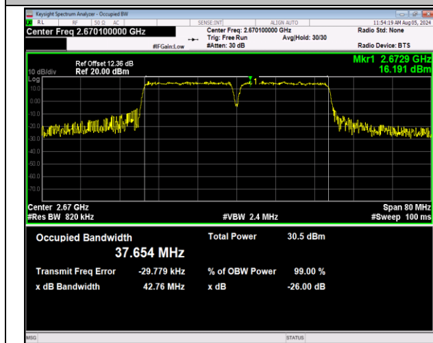
41-41-20MHz-20MHz-64QAM-64QAM-41292-41490-100R B#0-100RB#0-PASS
