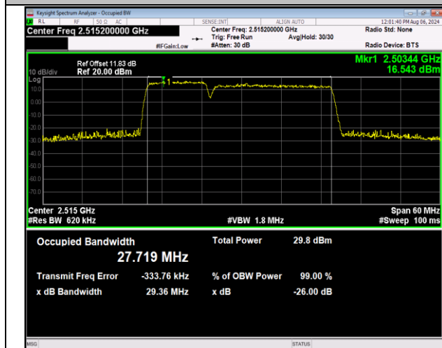
7-7-10MHz-20MHz-16QAM-16QAM-20805-20949-50RB#0 -100RB#0-PASS
