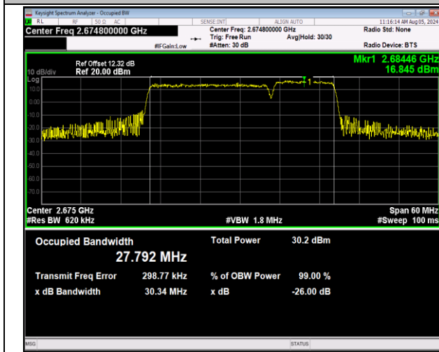
41-41-20MHz-10MHz-64QAM-64QAM-41391-41535-100R B#0-50RB#0-PASS
