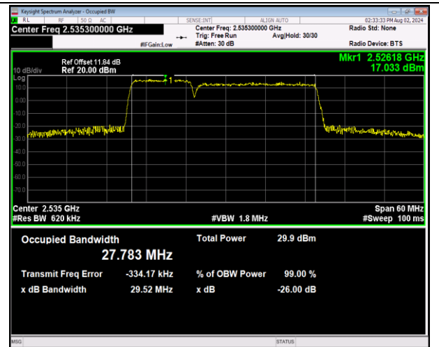
7-7-10MHz-20MHz-64QAM-64QAM-21006-21150-50RB#0 -100RB#0-PASS
