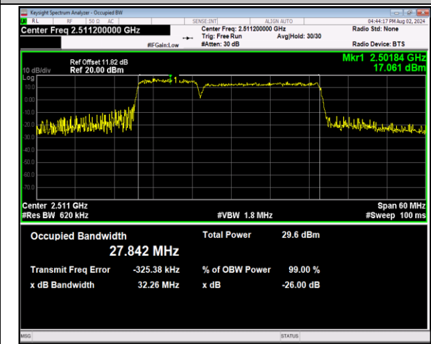
41-41-10MHz-20MHz-64QAM-64QAM-39705-39849-50RB #0-100RB#0-PASS
