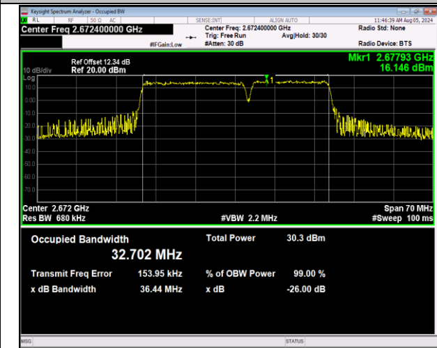
41-41-20MHz-15MHz-64QAM-64QAM-41341-41512-100R B#0-75RB#0-PASS
