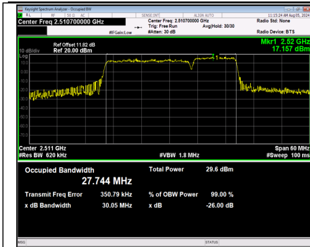
41-41-20MHz-10MHz-64QAM-64QAM-39750-39894-100R B#0-50RB#0-PASS
