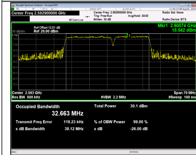
41-41-20MHz-15MHz-64QAM-64QAM-40546-40717-100R B#0-75RB#0-PASS
