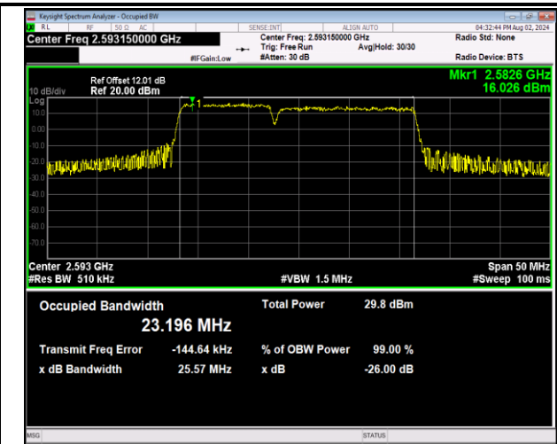
41-41-10MHz-15MHz-64QAM-64QAM-40549-40669-50RB #0-75RB#0-PASS
