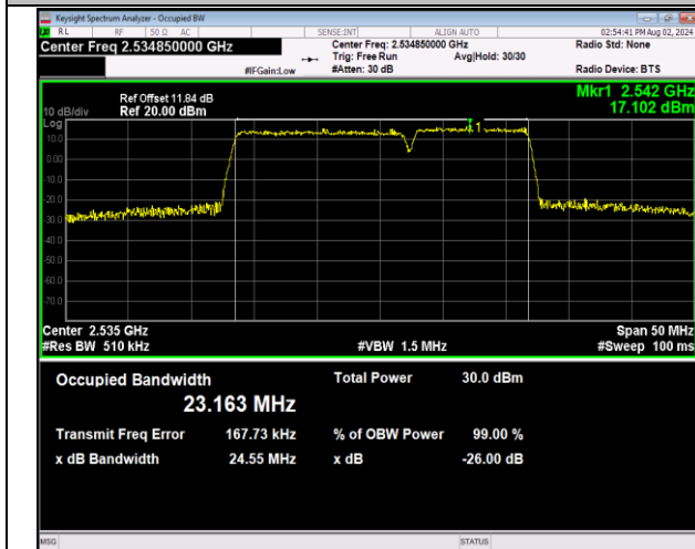
7-7-15MHz-10MHz-64QAM-64QAM-21051-21171-75RB#0
