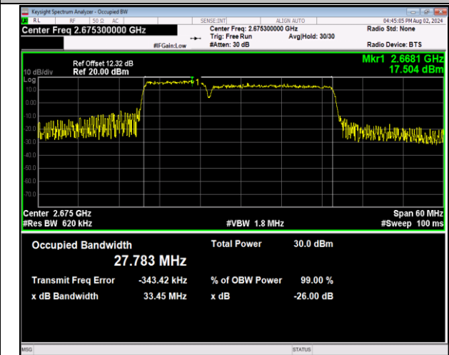
41-41-10MHz-20MHz-64QAM-64QAM-41346-41490-50RB #0-100RB#0-PASS
