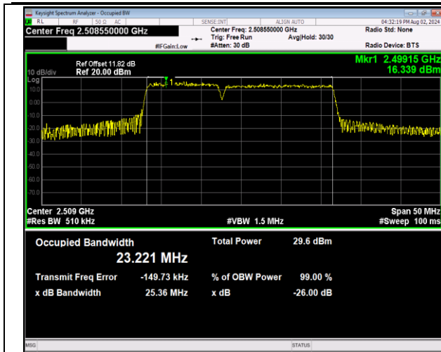
41-41-10MHz-15MHz-64QAM-64QAM-39703-39823-50RB #0-75RB#0-PASS
