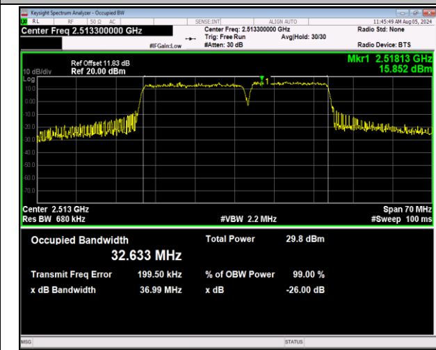
41-41-20MHz-15MHz-64QAM-64QAM-39750-39921-100R B#0-75RB#0-PASS
