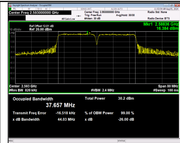
41-41-20MHz-20MHz-64QAM-64QAM-40521-40719-100R B#0-100RB#0-PASS
