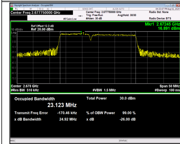
41-41-10MHz-15MHz-64QAM-64QAM-41395-41515-50RB #0-75RB#0-PASS
