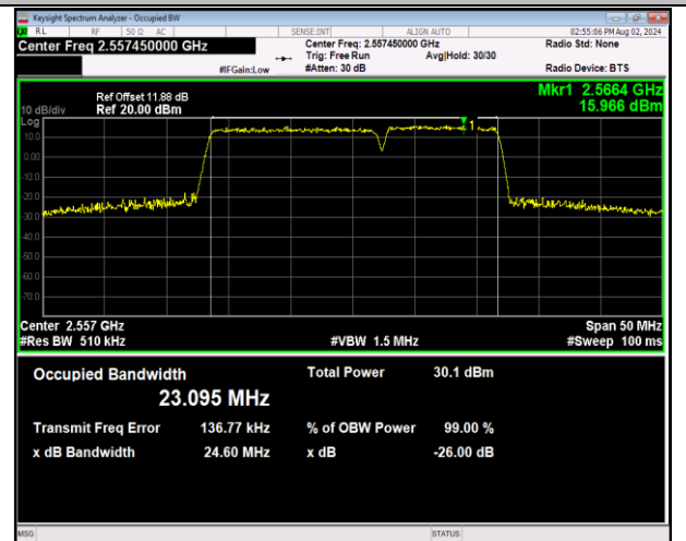
7-7-15MHz-10MHz-64QAM-64QAM-21277-21397-75RB#0
