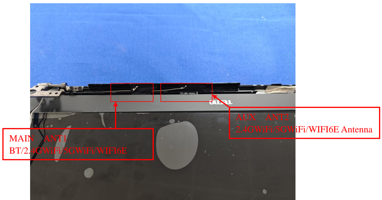
Internal photograph of EUT
