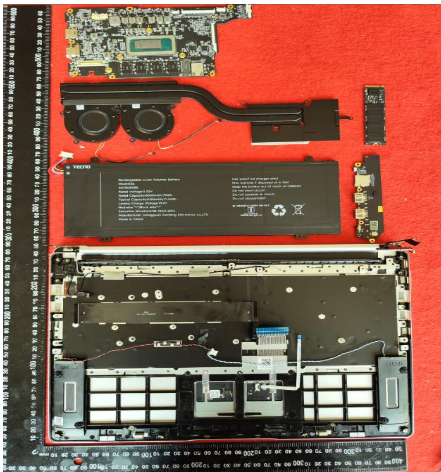
Internal photograph of EUT
