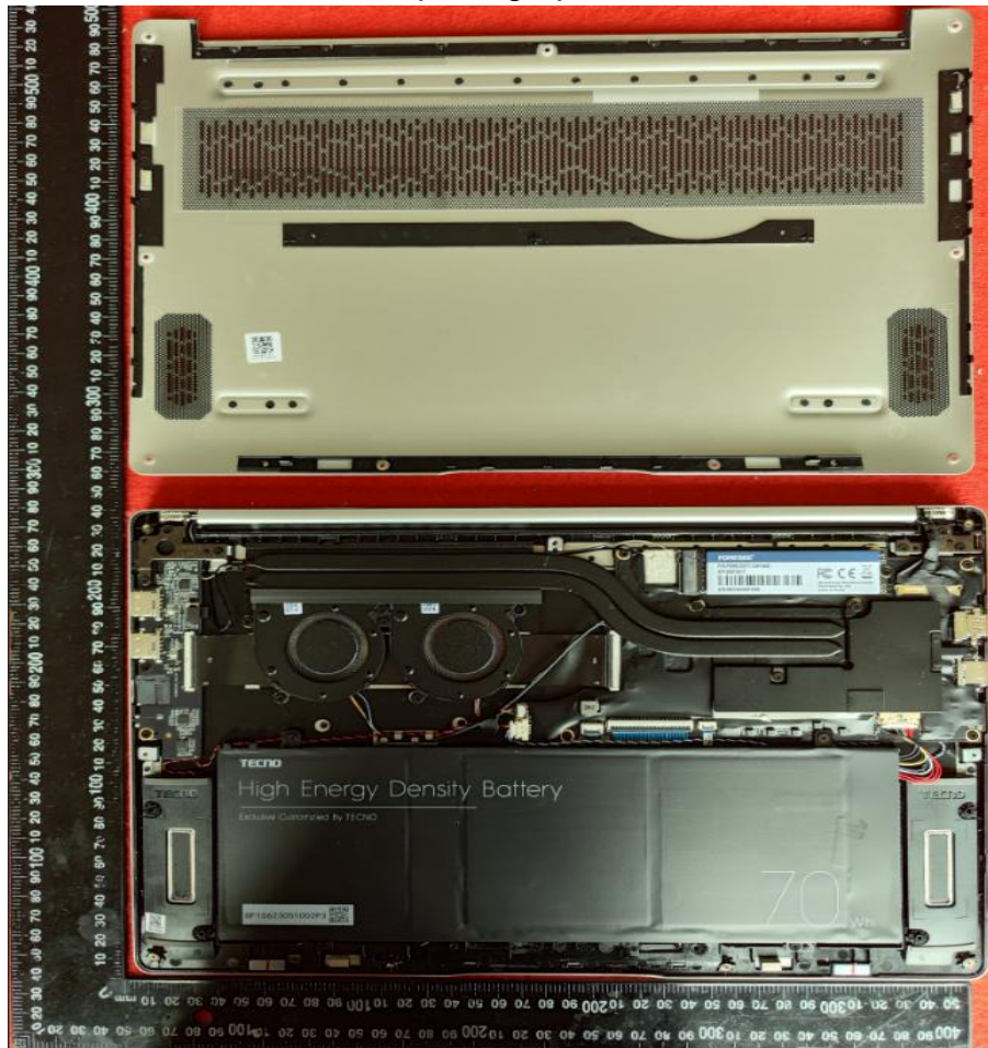
Internal photograph of EUT
