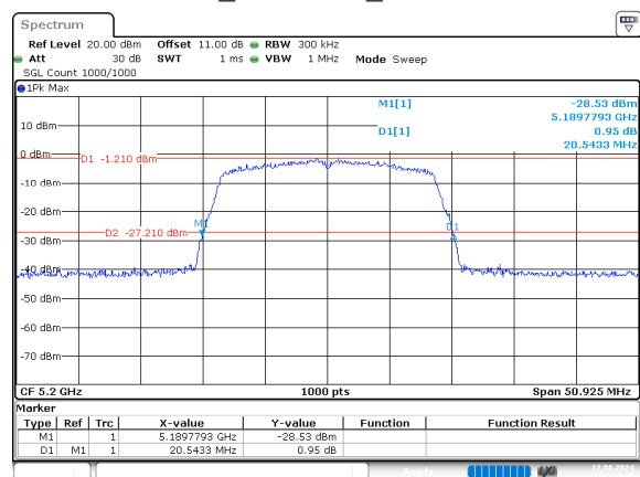
n20_5200MHz_Chain 0
