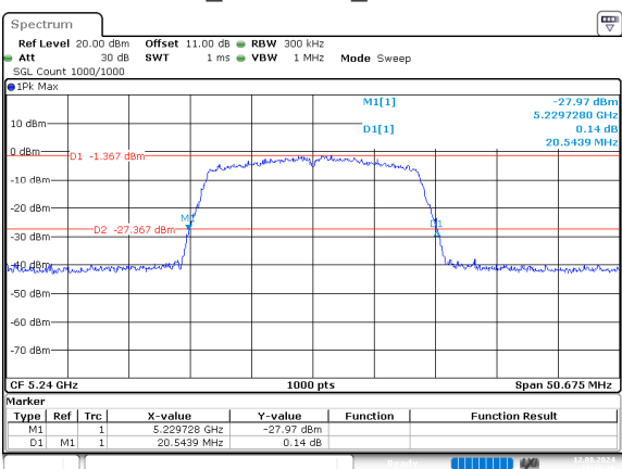
n20_5240MHz_Chain 0
