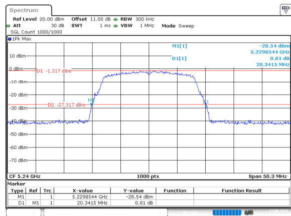
a_5240MHz_Chain 0
