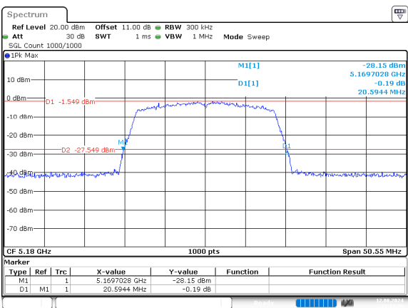
n20_5180MHz_Chain 0
