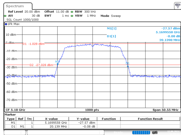
a_5180MHz_Chain 0
