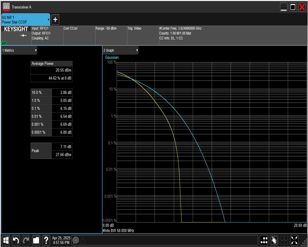
n78(3550-3700) SCS=30kHz DFT_QAM64 BW=50MHz Channel=645000 RB=128@0
