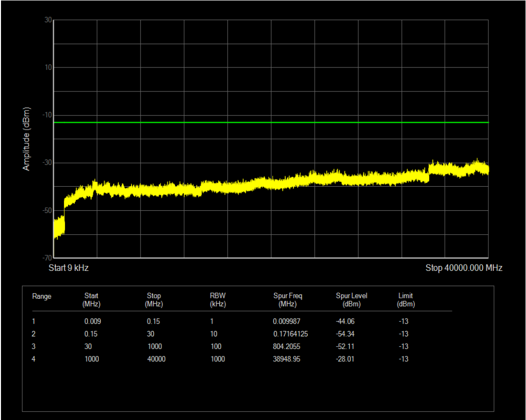
n77(3550-3700) SCS=30kHz CP_QPSK BW=10MHz Channel=646332 RB=1@0
