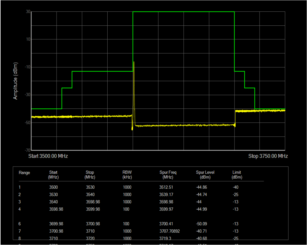
n77(3550-3700) SCS=30kHz CP_QPSK BW=100MHz Channel=643332 RB=1@272
