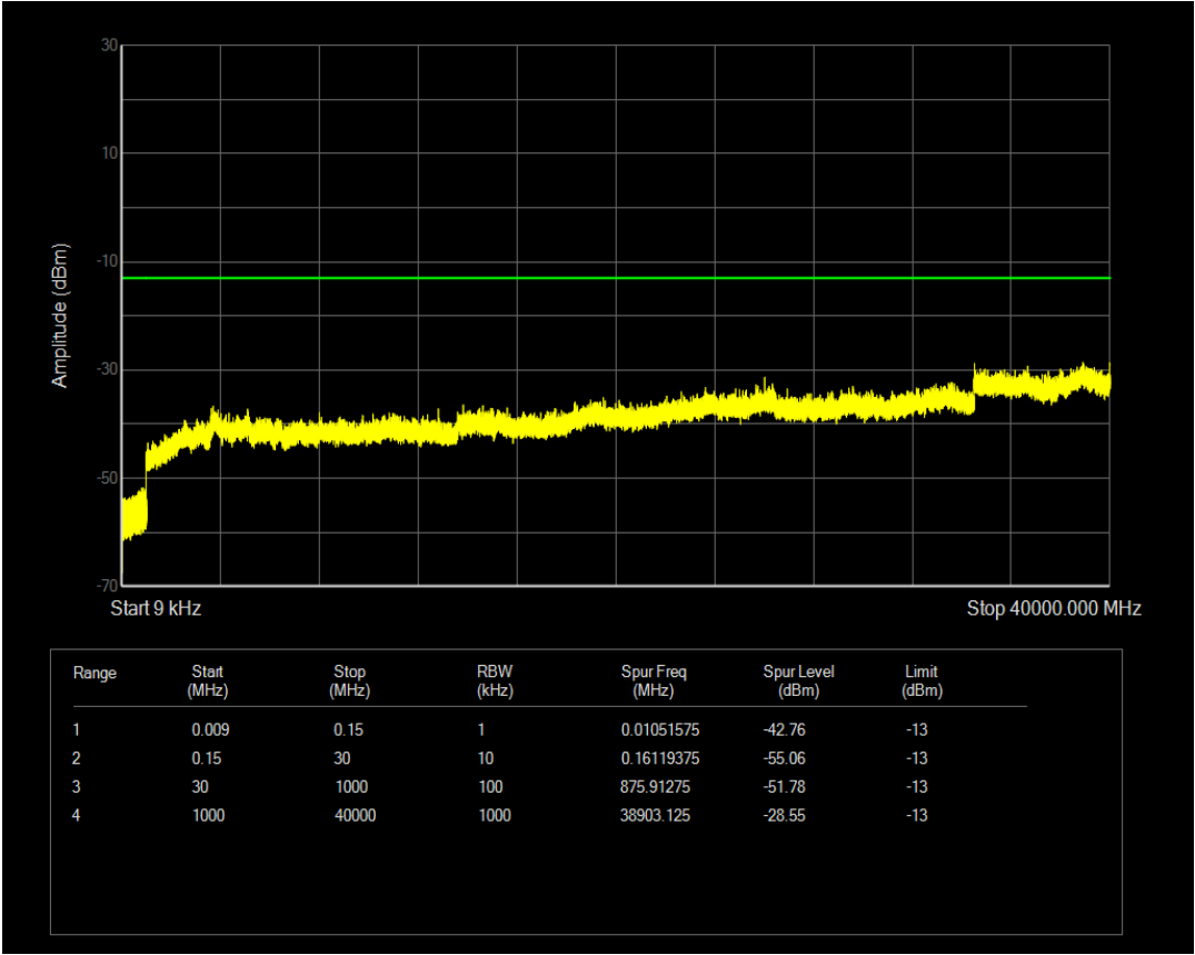
n77(3550-3700) SCS=30kHz CP_QPSK BW=10MHz Channel=646332 RB=1@23
