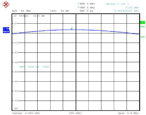
DH1_Low 3.35dBm
