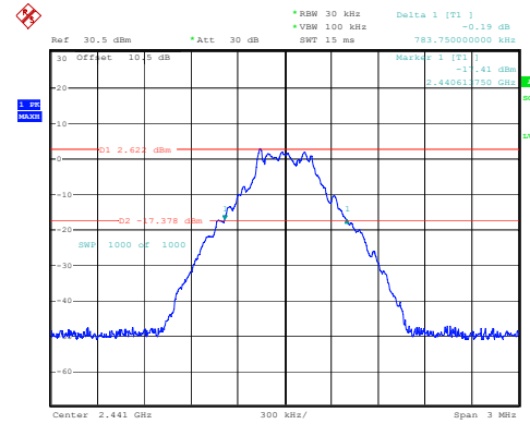
DH1_Middle 0.784MHz
