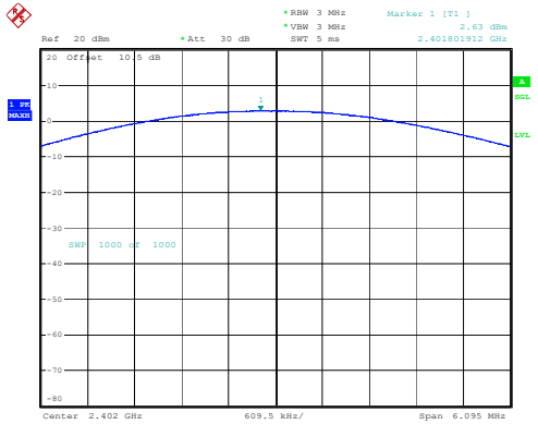
2DH1_Low 2.63dBm
