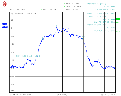
2DH1_High 1.133MHz
