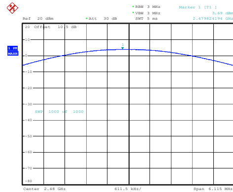
3DH1_High 3.69dBm
