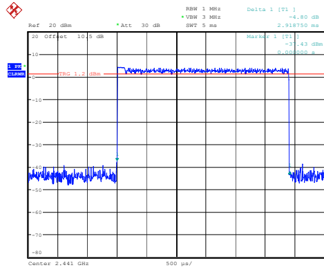
3DH5_Hopping 2.919ms
