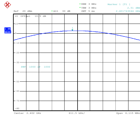
3DH1_Low 2.51dBm
