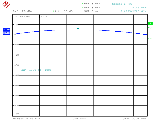
DH1_High 4.59dBm
