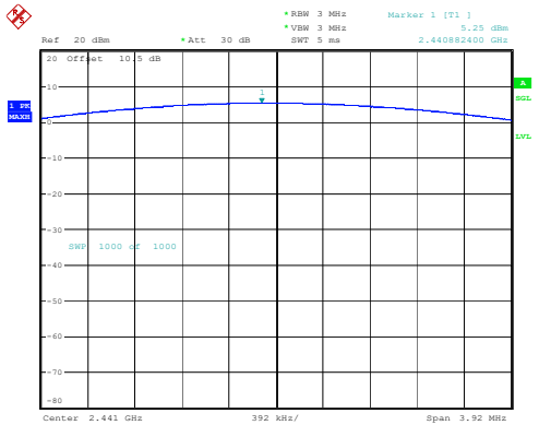
DH1_Middle 5.25dBm
