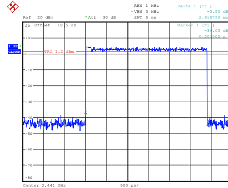
3DH5_Hopping 2.919ms
