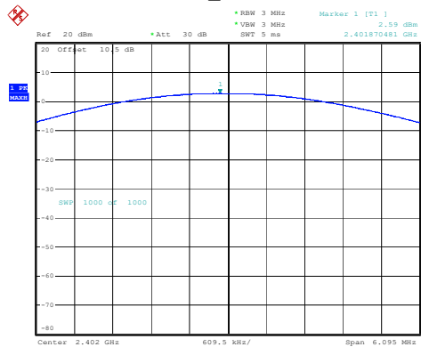
2DH1_Low 2.59dBm
