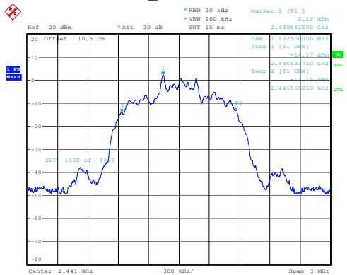
2DH1_Middle 1.133MHz
