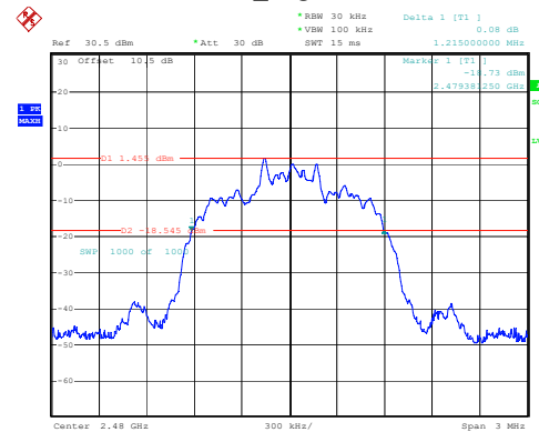
2DH1_High 1.215MHz
