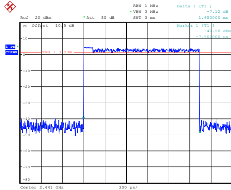
3DH3_Hopping 1.650ms
