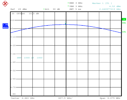
2DH1_Middle 4.52dBm
