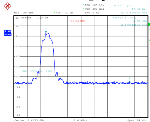
2DH1_High
