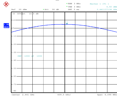
2DH1_Middle 4.50dBm
