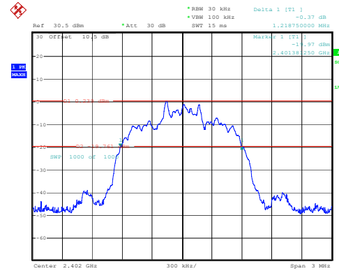
2DH1_Low 1.219MHz
