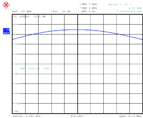
3DH1_Middle 4.42dBm
