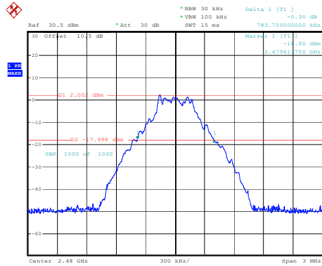
DH1_High 0.784MHz
