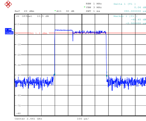
3DH1_Hopping 0.390ms
