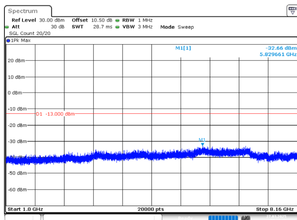
10MHz_Low_QPSK_1@0(1GHz~8.16GHz)
