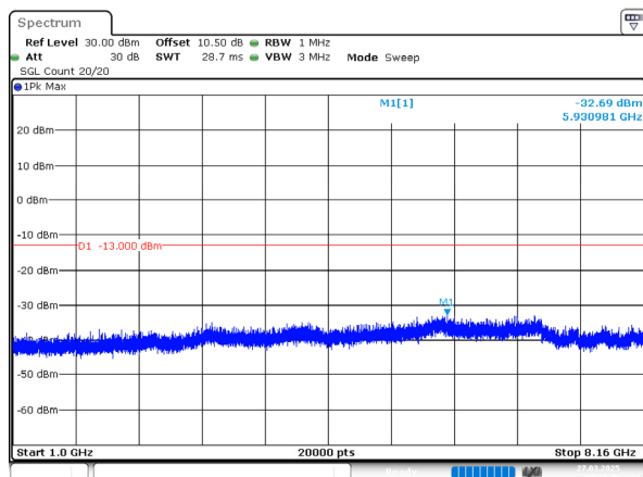
5MHz_High_QPSK_25@0(1GHz~8.16GHz)
