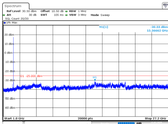
5MHz_Middle_QPSK_1@0(1GHz~27.2GHz)
