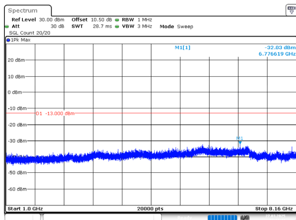
10MHz_Middle_QPSK_1@0(1GHz~8.16GHz)
