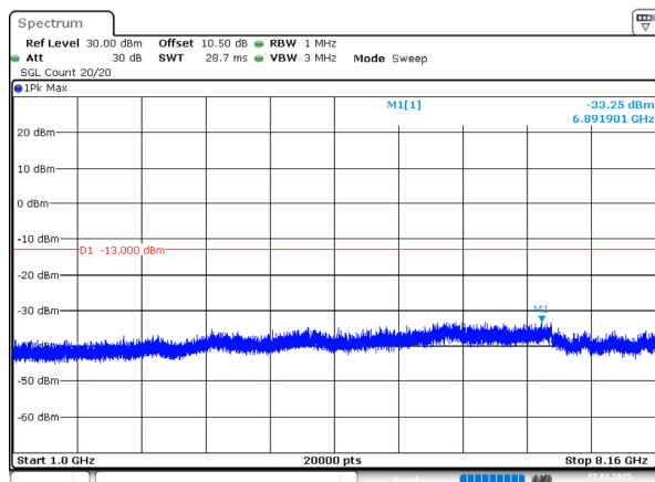
1.4MHz_Middle_QPSK_6@0(1GHz~8.16GHz)
