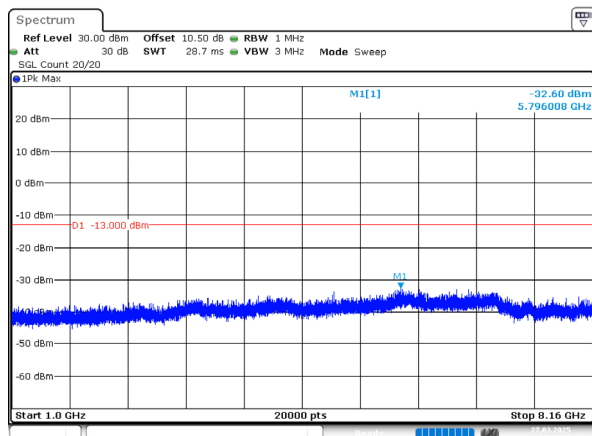
1.4MHz_High_QPSK_6@0(1GHz~8.16GHz)
