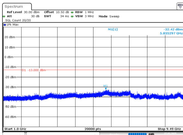
1.4MHz_Middle_QPSK_1@0(1GHz~9.49GHz)
