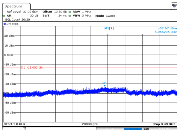
1.4MHz_Low_QPSK_6@0(1GHz~9.49GHz)
