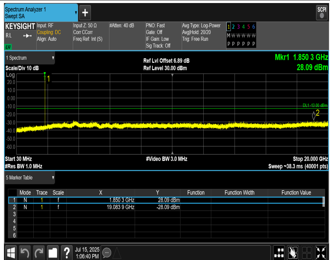
GSM1900 Channel=512
