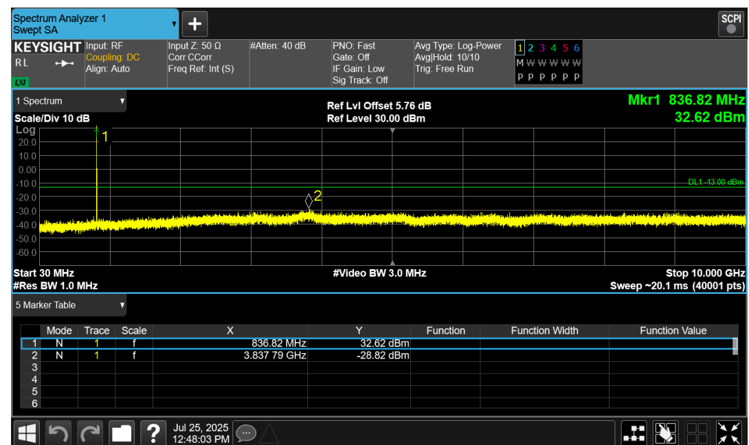
GSM850 Channel=190
