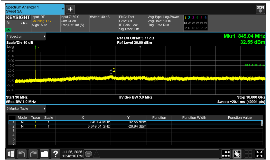
GSM850 Channel=251
