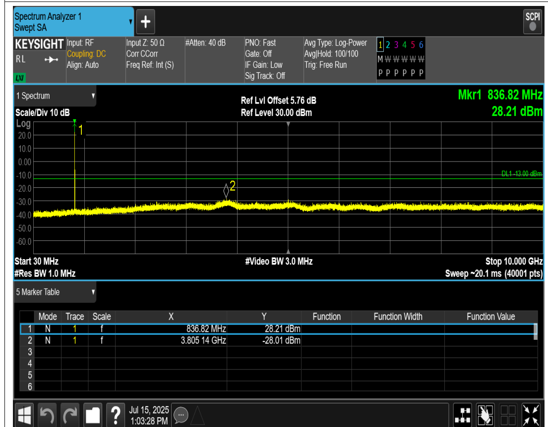
EGPRS850 Channel=190
