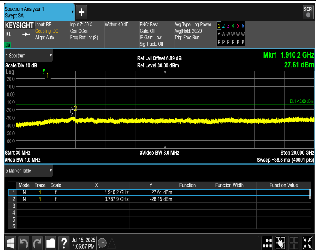
GSM1900 Channel=810
