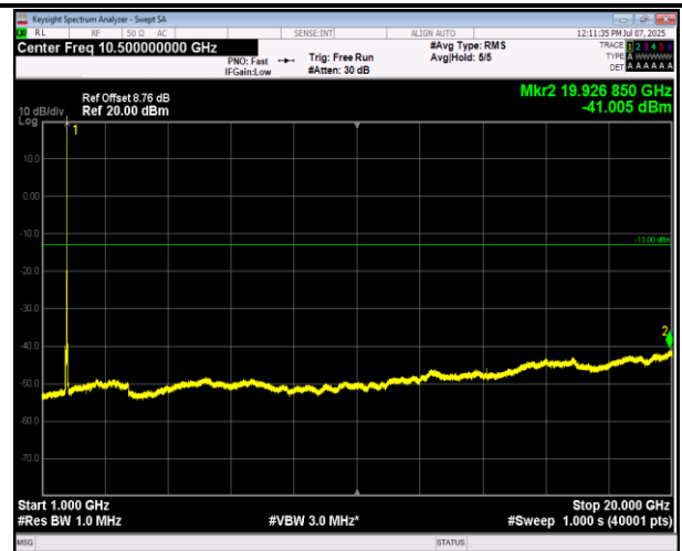
66-66-20MHz-5MHz-16QAM-16QAM-132397-132514-100R B#0-25RB#0-1000~20000MHz-PASS
