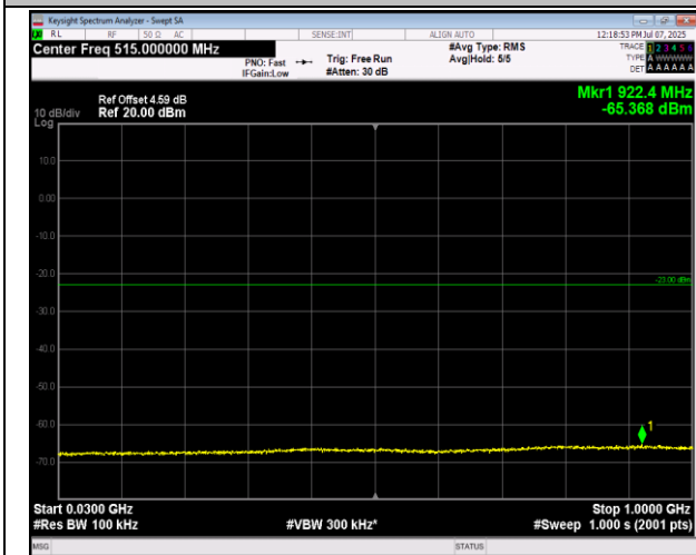
66-66-20MHz-5MHz-16QAM-16QAM-132522-132639-1R B#0-ORB#0-30~1000MHz-PASS
