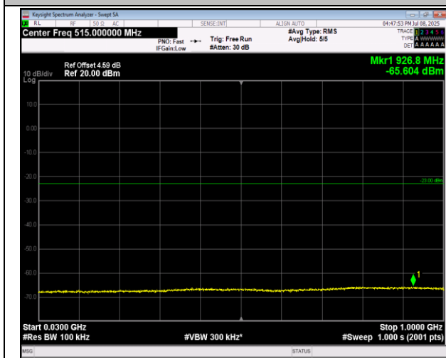
66-66-20MHz-20MHz-16QAM-16QAM-132072-132270-1 00RB#0-100RB#0-30~1000MHz-PASS
