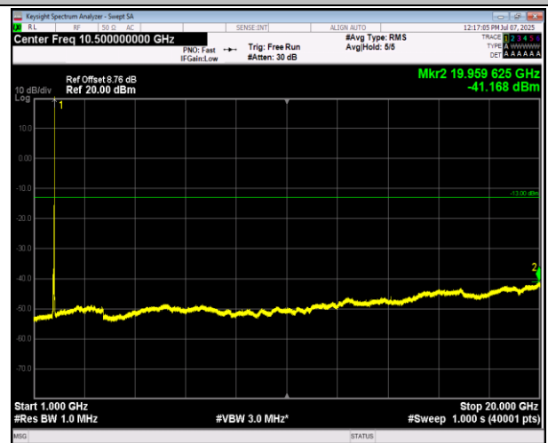
66-66-20MHz-5MHz-16QAM-16QAM-132522-132639-100R B#0-25RB#0-1000~20000MHz-PASS
