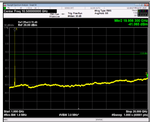
66-66-20MHz-5MHz-16QAM-16QAM-132522-132639-1RB #99-ORB#0-1000~20000MHz-PASS
