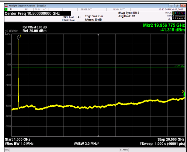
66-66-20MHz-5MHz-16QAM-16QAM-132397-132514-1RB #99-ORB#0-1000~20000MHz-PASS
