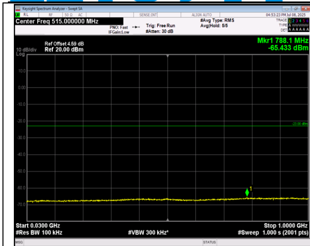
66-66-20MHz-20MHz-16QAM-16QAM-132323-132521-100RB#0-100RB#0-30~1000MHz-PASS
