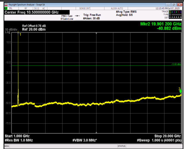
66-66-20MHz-5MHz-16QAM-16QAM-132522-132639-1RB #0-1RB#24-1000~20000MHz-PASS
