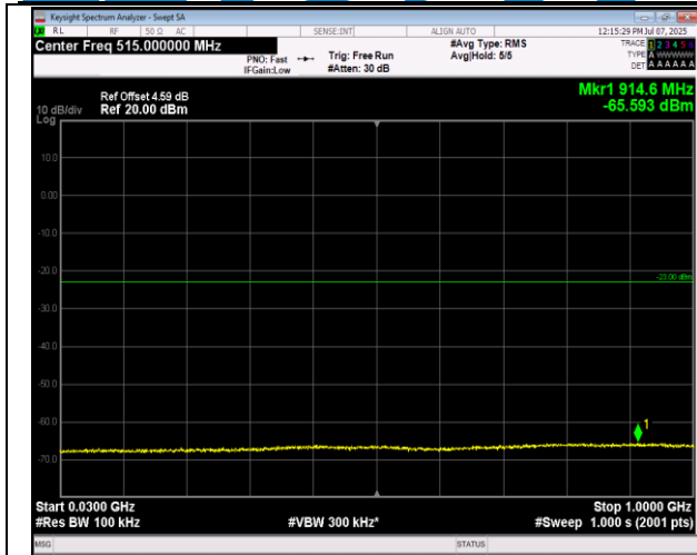
66-66-20MHz-5MHz-16QAM-16QAM-132522-132639-1R B#0-1RB#24-30~1000MHz-PASS
