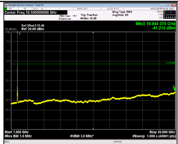
66-66-20MHz-20MHz-16QAM-16QAM-132323-132521-100RB#0-100RB#0-1000~20000MHz-PASS
