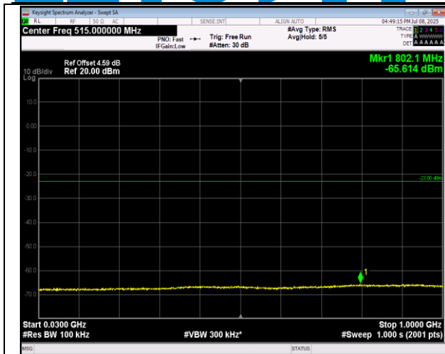
66-66-20MHz-20MHz-16QAM-16QAM-132072-132270-1 RB#99-ORB#0-30~1000MHz-PASS
