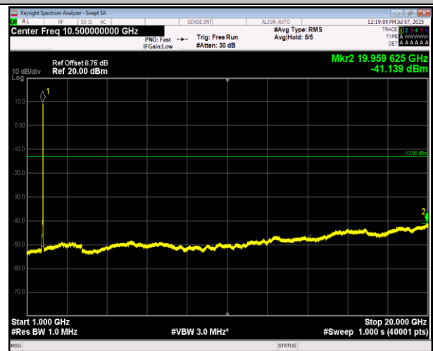
66-66-20MHz-5MHz-16QAM-16QAM-132522-132639-1RB #0-ORB#0-1000~20000MHz-PASS
