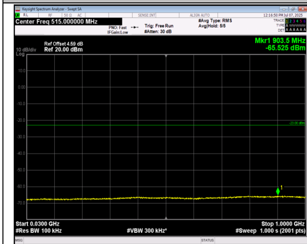
66-66-20MHz-5MHz-16QAM-16QAM-132522-132639-10 ORB#0-25RB#0-30~1000MHz-PASS
