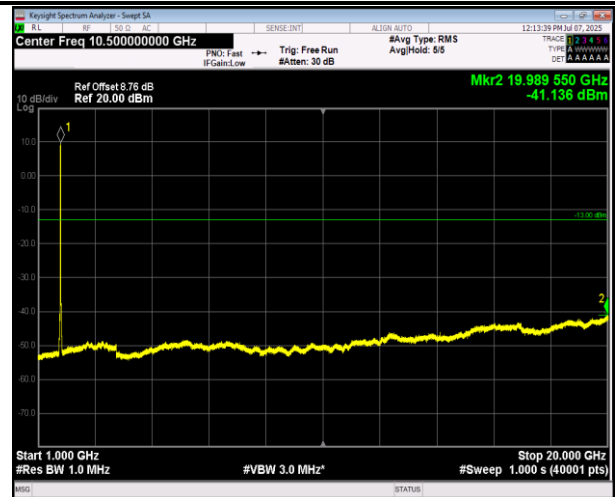
66-66-20MHz-5MHz-16QAM-16QAM-132397-132514-1RB #0-ORB#0-1000~20000MHz-PASS
