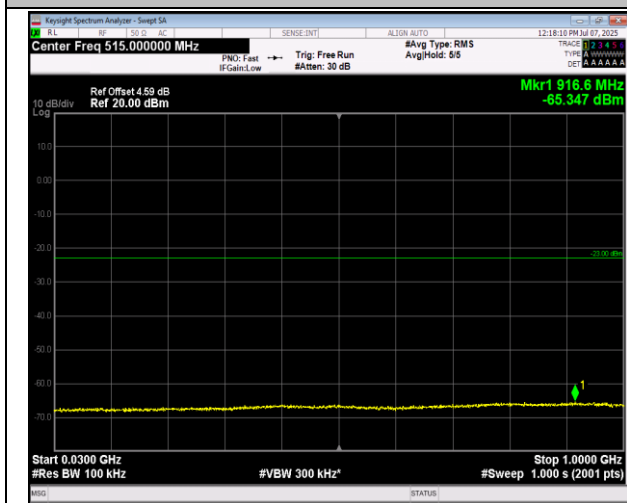
66-66-20MHz-5MHz-16QAM-16QAM-132522-132639-1R B#99-ORB#0-30~1000MHz-PASS
