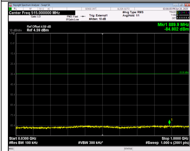
41(2555-2655)-41(2555-2655)-15MHz-15MHz-QPSK-QP SK-40315-40465-1RB#74-ORB#0-30~1000MHz-PASS
