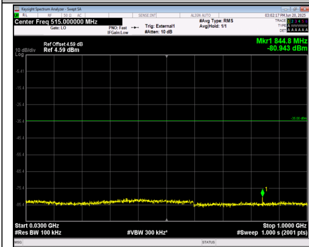
41(2555-2655)-41(2555-2655)-15MHz-15MHz-QPSK-QP SK-40315-40465-1RB#0-1RB#74-30~1000MHz-PASS
