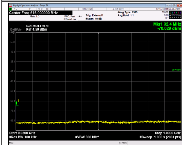
41(2555-2655)-41(2555-2655)-15MHz-10MHz-16QAM-16 QAM-40691-40811-1RB#74-ORB#0-30~1000MHz-PASS
