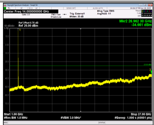
38-38-20MHz-20MHz-16QAM-16QAM-37952-38150-1RB# 99-0RB#0-1000~27000MHz-PASS
