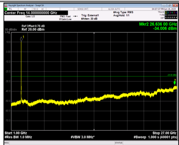
38-38-20MHz-20MHz-16QAM-16QAM-37952-38150-1RB# 0-0RB#0-1000~27000MHz-PASS
