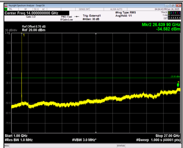
38-38-20MHz-20MHz-16QAM-16QAM-37952-38150-100R B#0-100RB#0-1000~27000MHz-PASS
