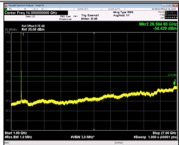
38-38-20MHz-20MHz-16QAM-16QAM-37901-38099-1RB# 99-ORB#0-1000~27000MHz-PASS
