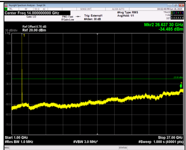
38-38-20MHz-20MHz-16QAM-16QAM-37952-38150-1RB# 0-1RB#99-1000~27000MHz-PASS
