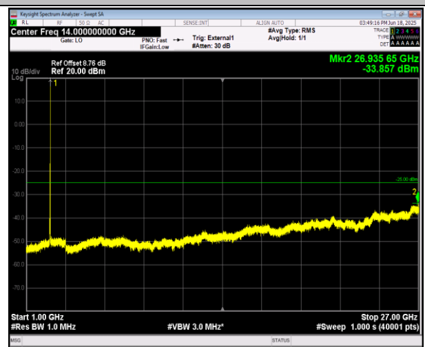
38-38-20MHz-20MHz-16QAM-16QAM-37850-38048-100R B#0-100RB#0-1000~27000MHz-PASS
