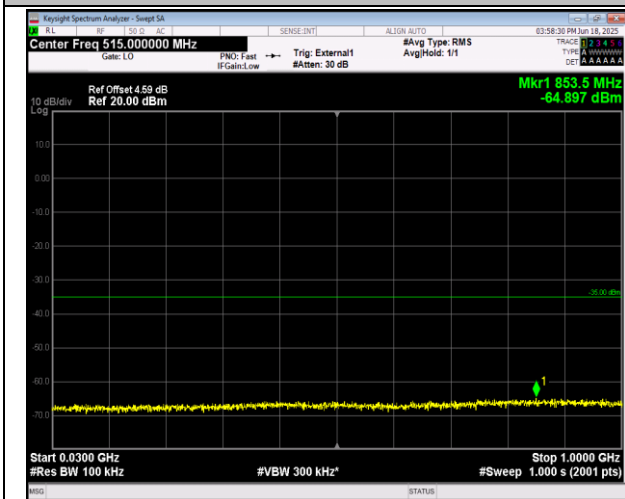
38-38-20MHz-20MHz-16QAM-16QAM-37901-38099-1RB #99-ORB#0-30~1000MHz-PASS
