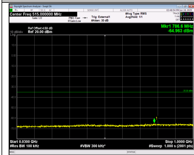
38-38-20MHz-20MHz-16QAM-16QAM-37850-38048-100 RB#0-100RB#0-30~1000MHz-PASS
