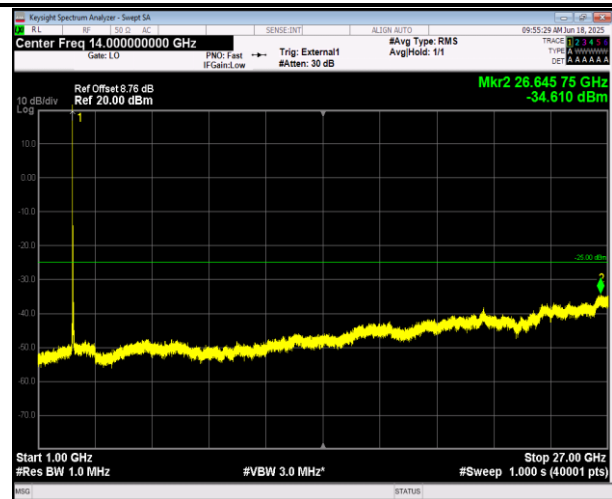
38-38-15MHz-15MHz-QPSK-QPSK-37925-38075-1RB#0-1RB#74-1000~27000MHz-PASS
