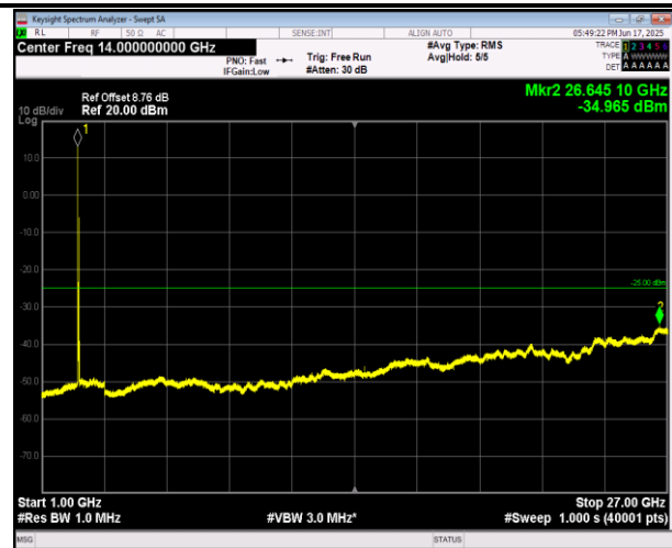
7-7-20MHz-20MHz-16QAM-16QAM-20850-21048-1RB#99- 0RB#0-1000~27000MHz-PASS
