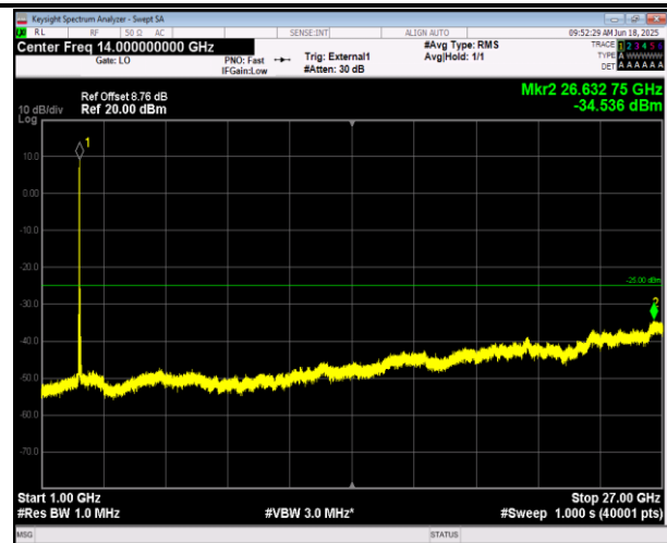
38-38-15MHz-15MHz-16QAM-16QAM-37825-37975-1RB# 74-ORB#0-1000~27000MHz-PASS
