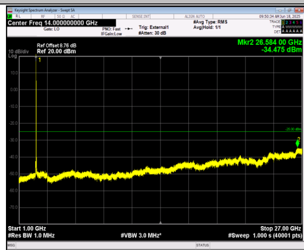
38-38-15MHz-15MHz-16QAM-16QAM-37825-37975-75RB #0-75RB#0-1000~27000MHz-PASS
