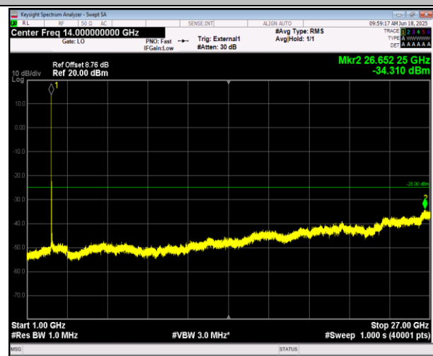
38-38-15MHz-15MHz-QPSK-QPSK-37925-38075-1RB#74-0RB#0-1000~27000MHz-PASS
