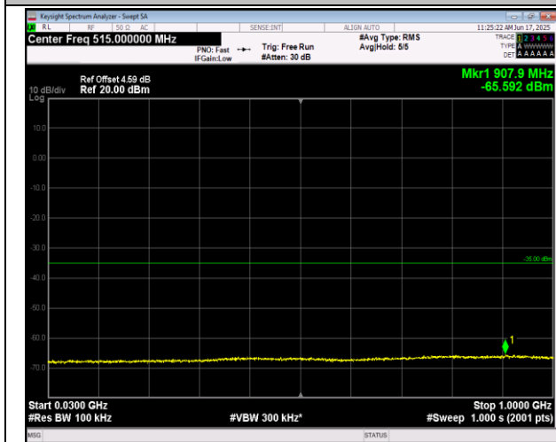
7-7-20MHz-10MHz-16QAM-16QAM-21251-21395-1RB#0-0 -ORB#0-30~1000MHz-PASS
