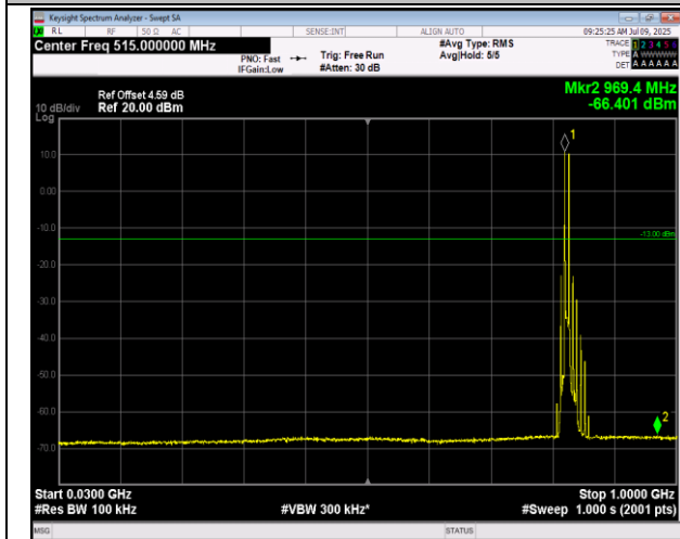
5-5-5MHz-3MHz-QPSK-QPSK-20425-20464-1RB#24-0R B#0-30~1000MHz-PASS
