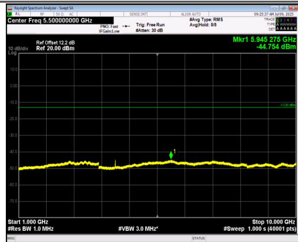
5-5-5MHz-3MHz-QPSK-QPSK-20425-20464-1RB#24-0RB# 0-1000~10000MHz-PASS
