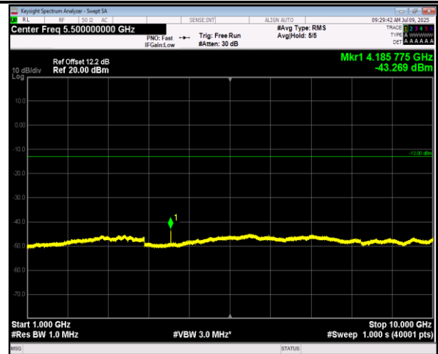
5-5-5MHz-3MHz-16QAM-16QAM-20510-20549-25RB#0-15RB#0-1000~10000MHz-PASS
