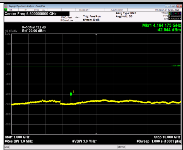
5-5-5MHz-3MHz-QPSK-QPSK-20510-20549-1RB#24-0RB# 0-1000~10000MHz-PASS
