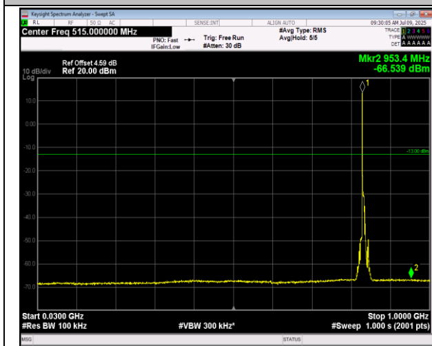
5-5-5MHz-3MHz-QPSK-QPSK-20510-20549-1RB#24-0R B#0-30~1000MHz-PASS
