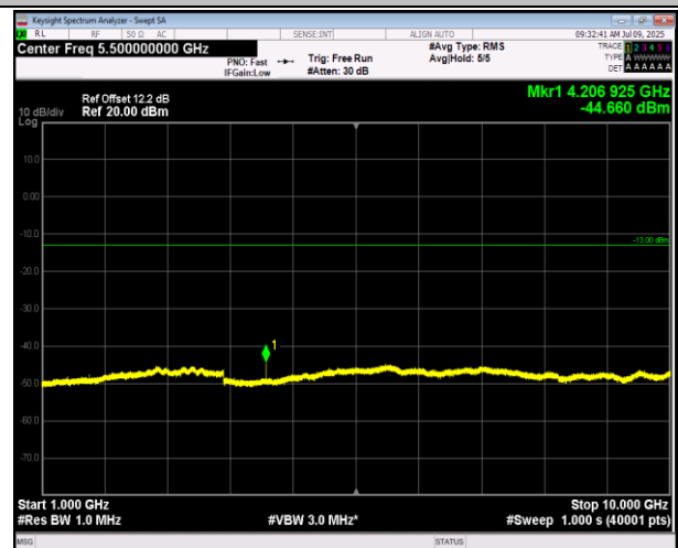
5-5-5MHz-3MHz-QPSK-QPSK-20595-20634-1RB#0-1RB#15-1000~10000MHz-PASS
