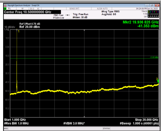
2-2-20MHz-20MHz-16QAM-16QAM-18700-18898-100RB# 0-100RB#0-1000~20000MHz-PASS
