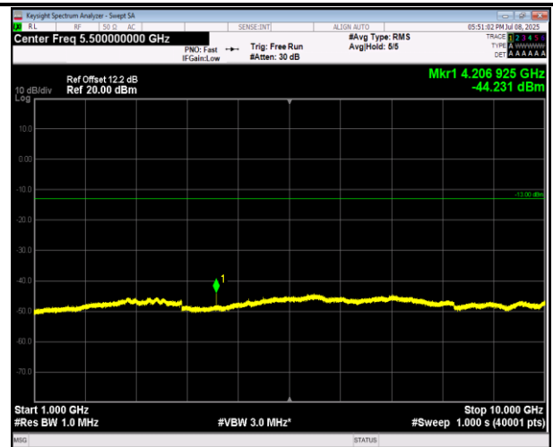
5-5-3MHz-5MHz-QPSK-QPSK-20586-20625-1RB#14-0RB# 0-1000~10000MHz-PASS
