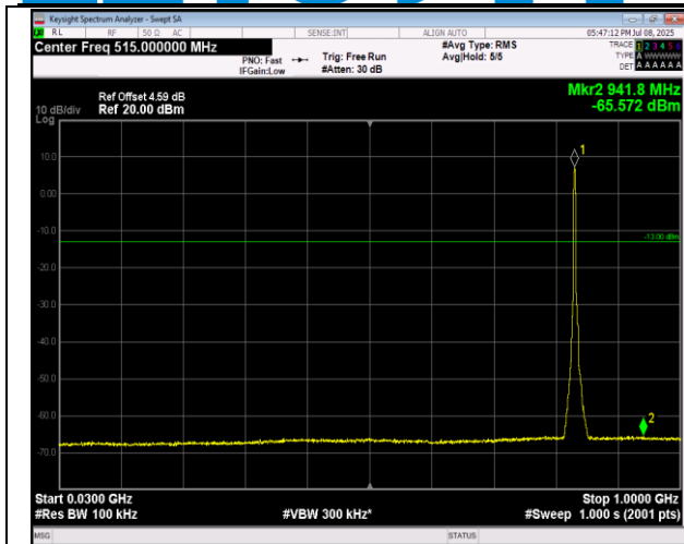
5-5-3MHz-5MHz-16QAM-16QAM-20501-20540-1RB#0-0 RB#0-30~1000MHz-PASS
