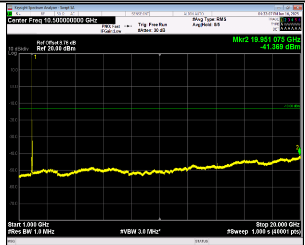
2-2-20MHz-20MHz-16QAM-16QAM-18902-19100-1RB#0-1 RB#99-1000~20000MHz-PASS
