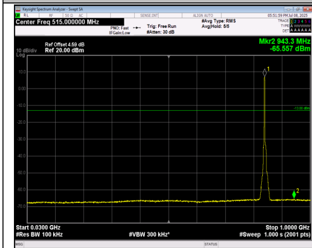
5-5-3MHz-5MHz-16QAM-16QAM-20586-20625-1RB#0-0 RB#0-30~1000MHz-PASS
