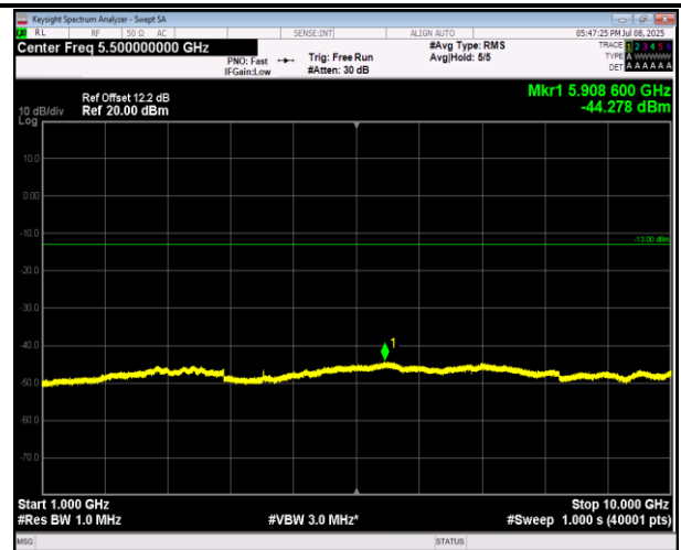
5-5-3MHz-5MHz-16QAM-16QAM-20501-20540-1RB#0-0R B#0-1000~10000MHz-PASS
