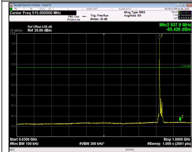
5-5-3MHz-5MHz-16QAM-16QAM-20416-20455-1RB#0-1 RB#24-30~1000MHz-PASS
