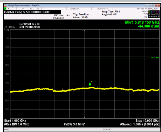
5-5-3MHz-5MHz-QPSK-QPSK-20586-20625-1RB#0-0RB#0-1000~10000MHz-PASS
