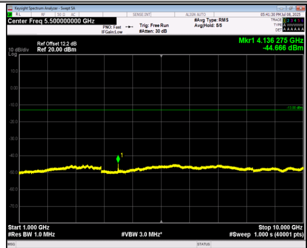
5-5-3MHz-5MHz-QPSK-QPSK-20416-20455-1RB#14-0RB# 0-1000~10000MHz-PASS
