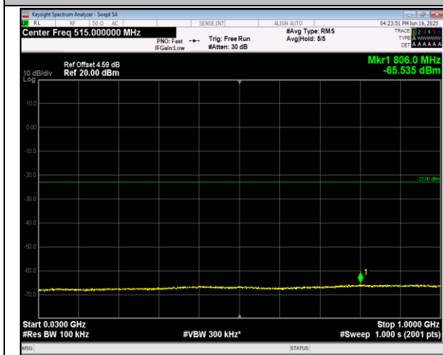
2-2-20MHz-20MHz-16QAM-16QAM-18700-18898-100RB #0-100RB#0-30~1000MHz-PASS
