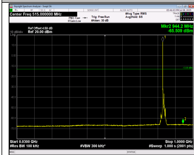
5-5-3MHz-5MHz-QPSK-QPSK-20501-20540-1RB#14-0R B#0-30~1000MHz-PASS
