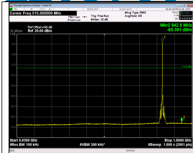
5-5-3MHz-5MHz-16QAM-16QAM-20501-20540-15RB#0-25RB#0-30~1000MHz-PASS
