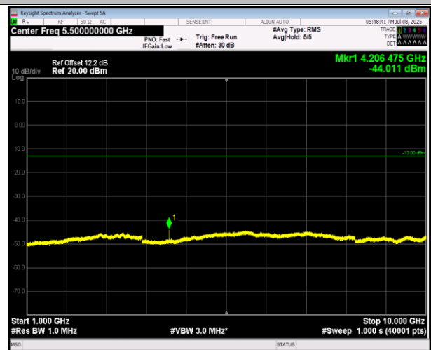
5-5-3MHz-5MHz-QPSK-QPSK-20586-20625-1RB#0-1RB#24-1000~10000MHz-PASS
