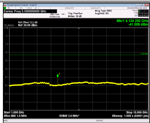
5-5-3MHz-5MHz-16QAM-16QAM-20416-20455-15RB#0-25RB#0-1000~10000MHz-PASS
