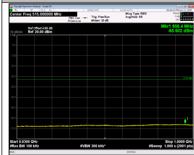
2-2-5MHz-20MHz-QPSK-QPSK-18983-19100-25RB#0-10 ORB#0-30~1000MHz-PASS
