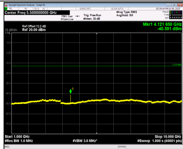
5-5-3MHz-5MHz-16QAM-16QAM-20416-20455-1RB#0-1R B#24-1000~10000MHz-PASS
