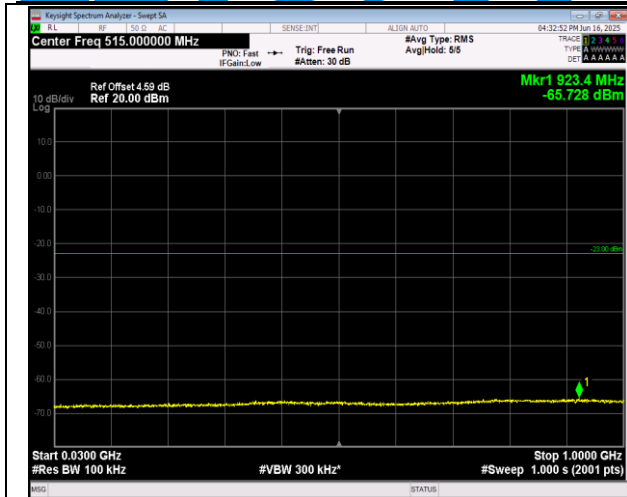
2-2-20MHz-20MHz-16QAM-16QAM-18902-19100-1RB#0 -1RB#99-30~1000MHz-PASS
