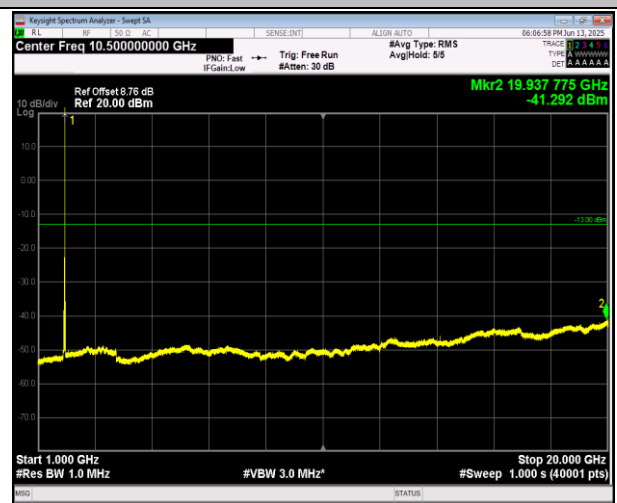
2-2-5MHz-20MHz-QPSK-QPSK-18983-19100-25RB#0-100 RB#0-1000~20000MHz-PASS
