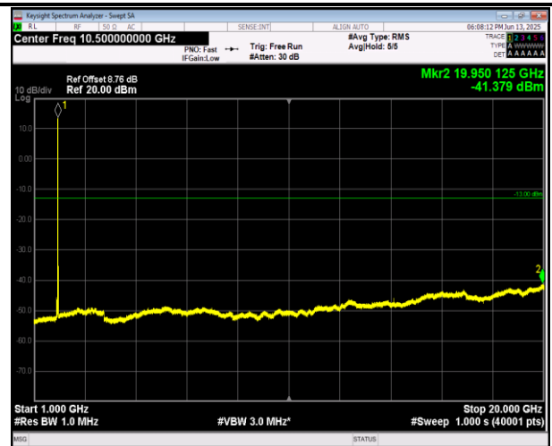
2-2-5MHz-20MHz-QPSK-QPSK-18983-19100-1RB#24-0RB #0-1000~20000MHz-PASS
