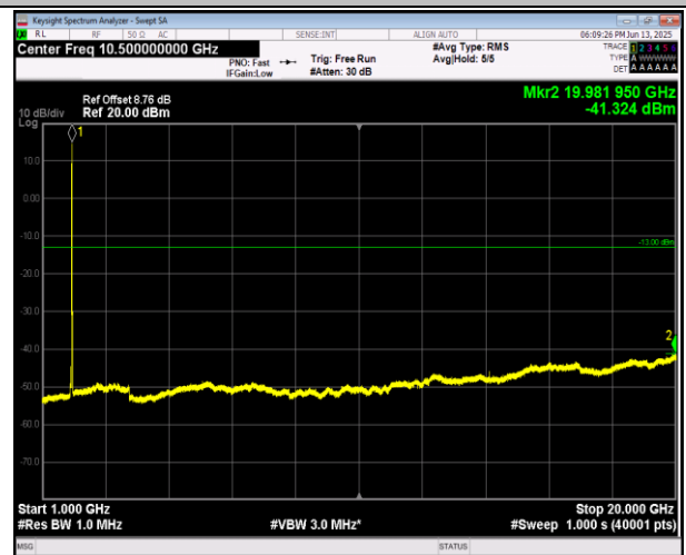
2-2-5MHz-20MHz-16QAM-16QAM-18983-19100-1RB#0-0R B#0-1000~20000MHz-PASS
