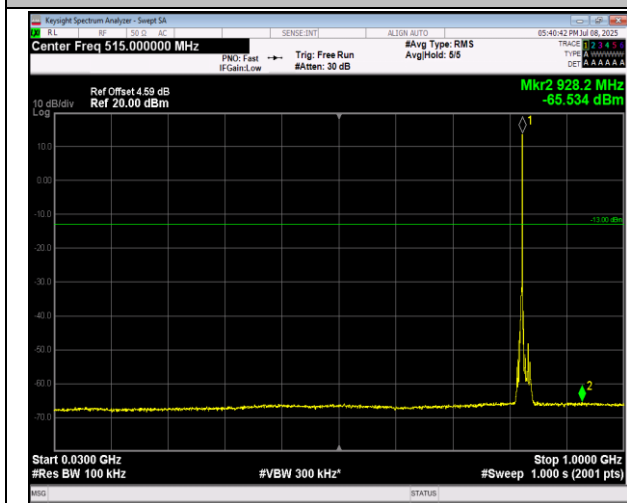
5-5-3MHz-5MHz-16QAM-16QAM-20416-20455-15RB#0-25RB#0-30~1000MHz-PASS
