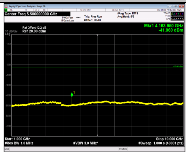
5-5-3MHz-5MHz-16QAM-16QAM-20501-20540-1RB#0-1R B#24-1000~10000MHz-PASS
