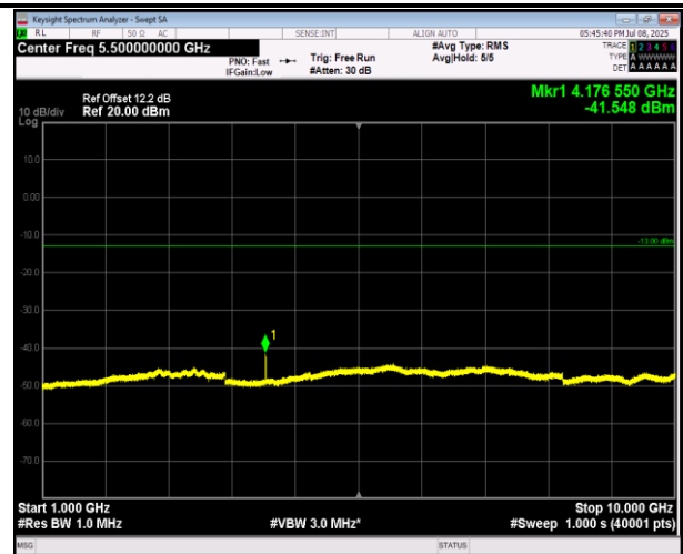
5-5-3MHz-5MHz-16QAM-16QAM-20501-20540-15RB#0-25RB#0-1000~10000MHz-PASS
