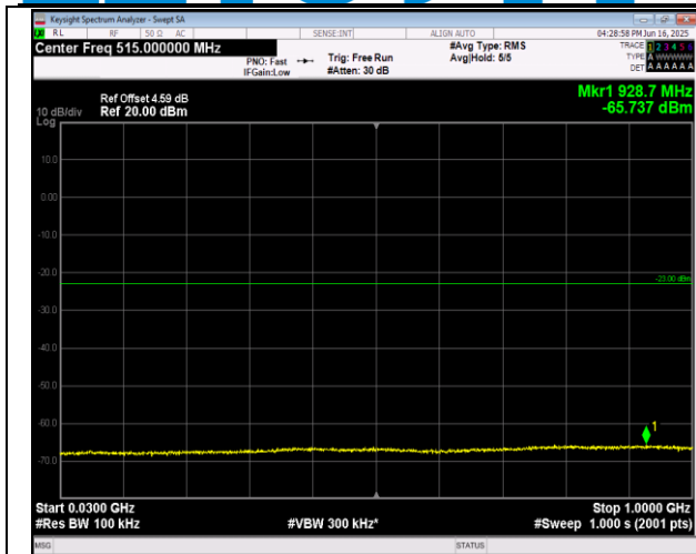
2-2-20MHz-20MHz-16QAM-16QAM-18801-18999-100RB #0-100RB#0-30~1000MHz-PASS
