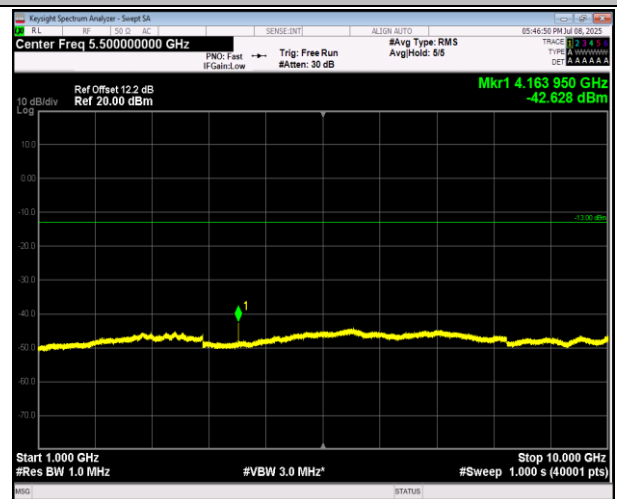
5-5-3MHz-5MHz-16QAM-16QAM-20501-20540-1RB#14-0R B#0-1000~10000MHz-PASS
