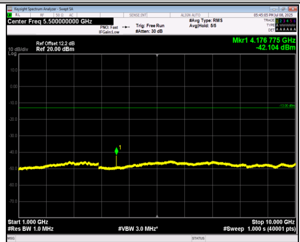
5-5-3MHz-5MHz-QPSK-QPSK-20501-20540-15RB#0-25RB #0-1000~10000MHz-PASS
