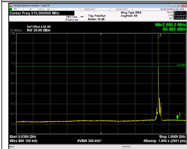
5-5-3MHz-5MHz-QPSK-QPSK-20586-20625-1RB#0-1RB#24-30~1000MHz-PASS
