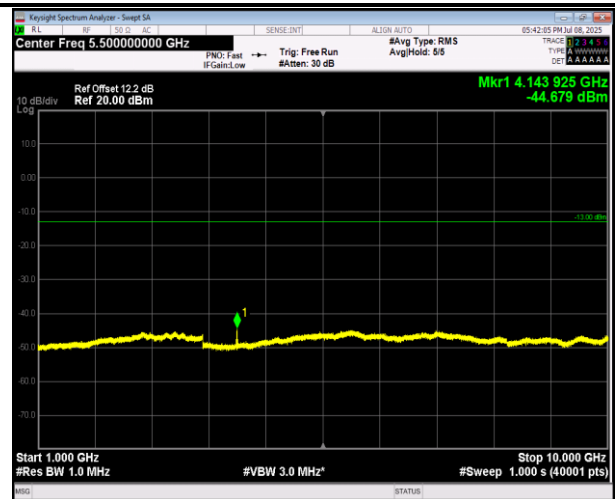
5-5-3MHz-5MHz-16QAM-16QAM-20416-20455-1RB#14-0RB#0-1000~10000MHz-PASS
