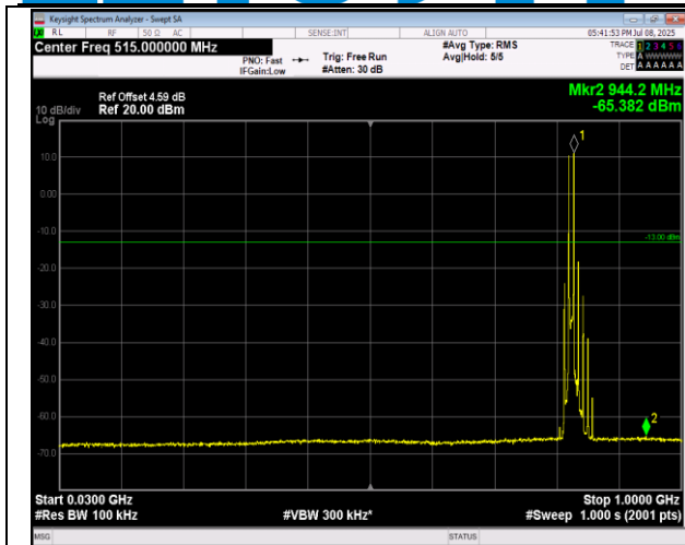
5-5-3MHz-5MHz-16QAM-16QAM-20416-20455-1RB#14-0RB#0-30~1000MHz-PASS
