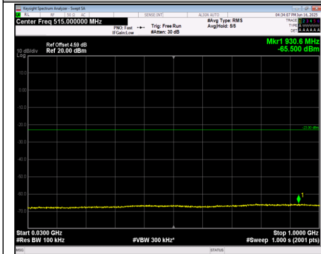
2-2-20MHz-20MHz-16QAM-16QAM-18902-19100-100RB #0-100RB#0-30~1000MHz-PASS
