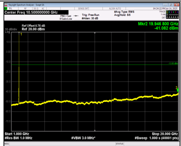
2-2-20MHz-20MHz-16QAM-16QAM-18902-19100-100RB# 0-100RB#0-1000~20000MHz-PASS
