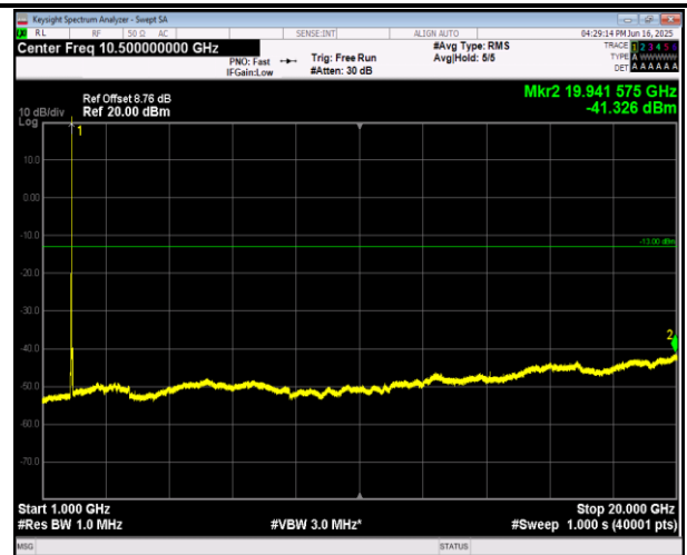
2-2-20MHz-20MHz-16QAM-16QAM-18801-18999-100RB# 0-100RB#0-1000~20000MHz-PASS
