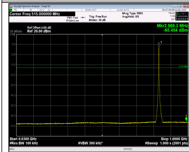
5-5-3MHz-5MHz-QPSK-QPSK-20586-20625-1RB#0-0RB#0-30~1000MHz-PASS
