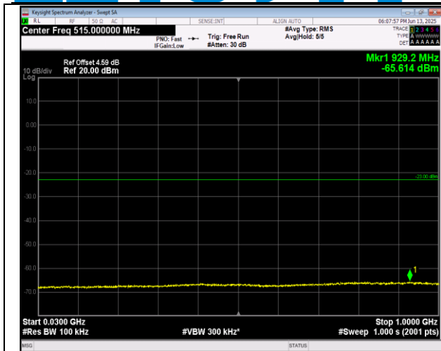
2-2-5MHz-20MHz-QPSK-QPSK-18983-19100-1RB#24-0 RB#0-30~1000MHz-PASS
