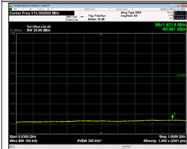
2-2-5MHz-20MHz-16QAM-16QAM-18983-19100-1RB#0- ORB#0-30~1000MHz-PASS
