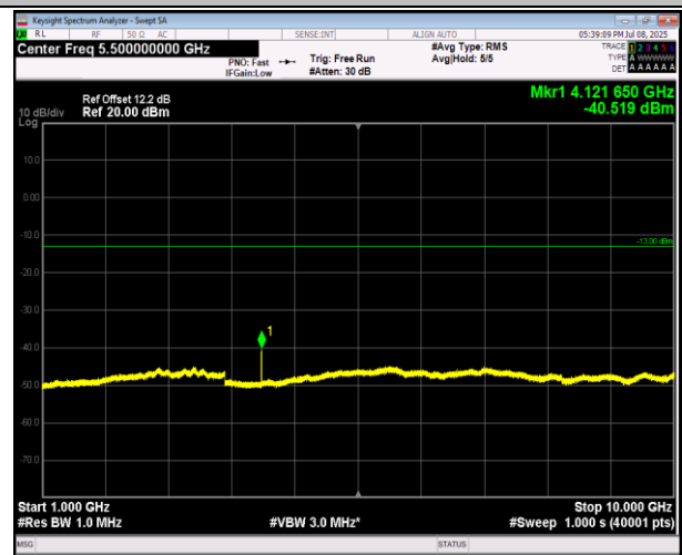
5-5-3MHz-5MHz-QPSK-QPSK-20416-20455-1RB#0-1RB#2 4-1000~10000MHz-PASS
