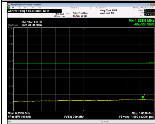
2-2-20MHz-20MHz-16QAM-16QAM-18902-19100-1RB#9 9-0RB#0-30~1000MHz-PASS
