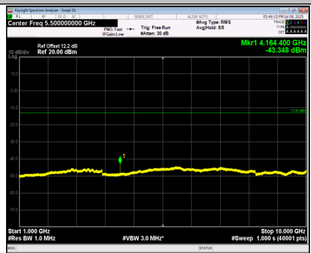
5-5-3MHz-5MHz-QPSK-QPSK-20501-20540-1RB#14-0RB# 0-1000~10000MHz-PASS
