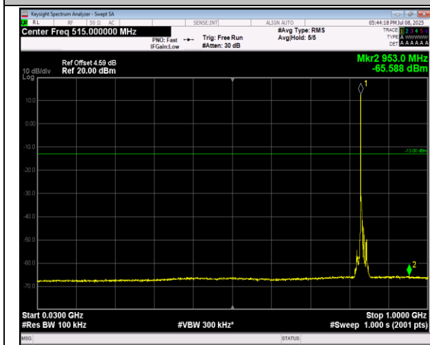
5-5-3MHz-5MHz-16QAM-16QAM-20501-20540-1RB#0-1 RB#24-30~1000MHz-PASS
