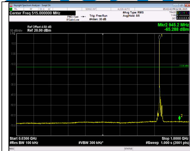
5-5-3MHz-5MHz-QPSK-QPSK-20501-20540-1RB#0-1RB #24-30~1000MHz-PASS
