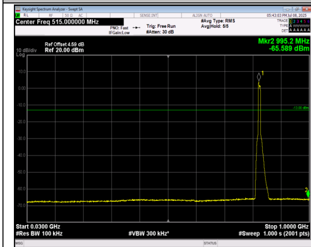
5-5-3MHz-5MHz-QPSK-QPSK-20501-20540-1RB#0-0RB#0-30~1000MHz-PASS
