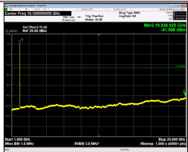
2-2-20MHz-20MHz-16QAM-16QAM-18902-19100-1RB#0-0 RB#0-1000~20000MHz-PASS
