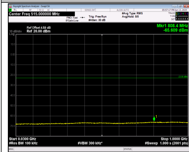
2-2-5MHz-20MHz-16QAM-16QAM-18633-18750-25RB#0 -100RB#0-30~1000MHz-PASS
