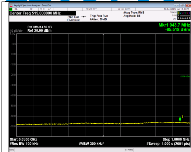
2-2-5MHz-20MHz-16QAM-16QAM-18808-18925-1RB#0- ORB#0-30~1000MHz-PASS
