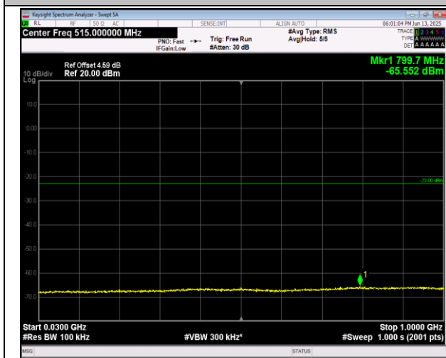
2-2-5MHz-20MHz-16QAM-16QAM-18808-18925-1RB#0- 1RB#99-30~1000MHz-PASS
