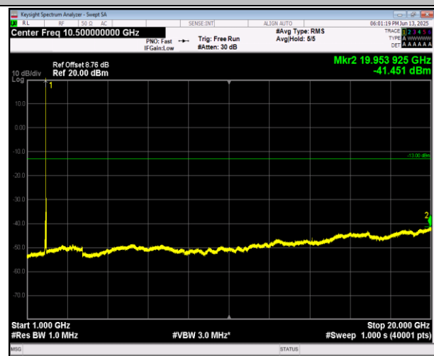
2-2-5MHz-20MHz-16QAM-16QAM-18808-18925-1RB#0-1R B#99-1000~20000MHz-PASS
