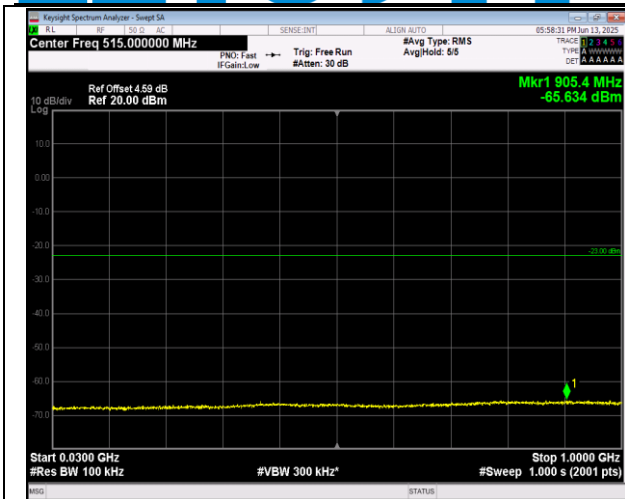
2-2-5MHz-20MHz-16QAM-16QAM-18633-18750-1RB#24 -0RB#0-30~1000MHz-PASS
