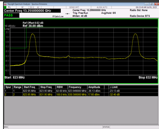
5-5-5MHz-3MHz-QPSK@QPSK-QPSK@QPSK-20425-204 64-25RB#0@25RB#0-15RB#0@15RB#0-PASS
