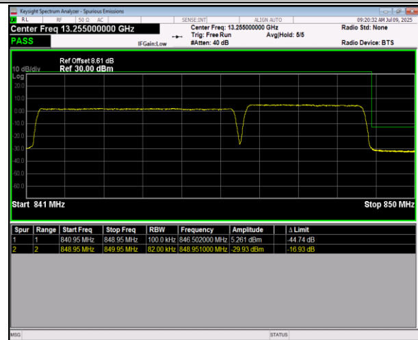
5-5-5MHz-3MHz-16QAM@16QAM-16QAM@16QAM-2059 5-20634-1RB#0@25RB#0-1RB#15@15RB#0-PASS
