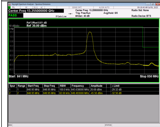
5-5-5MHz-3MHz-16QAM@16QAM-16QAM@16QAM-205 95-20634- 1RB#0@25RB#0-0RB#0@15RB#0-PASS
