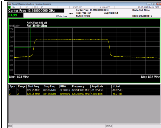
5-5-5MHz-3MHz-QPSK@QPSK-QPSK@QPSK-20425-20 464-1RB#24@25RB#0-0RB#0@15RB#0-PASS
