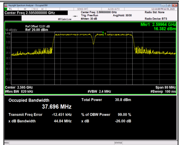
38-38-20MHz-20MHz-16QAM-16QAM-37952-38150-100RB B#0-100RB#0-PASS
