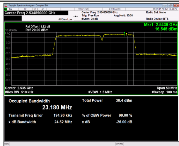
7-7-15MHz-10MHz-16QAM-16QAM-21277-21397-75RB#0-50 50RB#0-PASS
