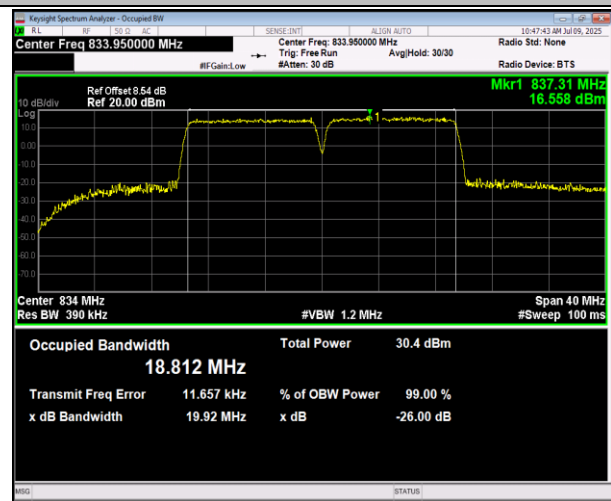
5-5-10MHz-10MHz-16QAM-16QAM-20476-20575-50RB#0-5 50RB#0-PASS
