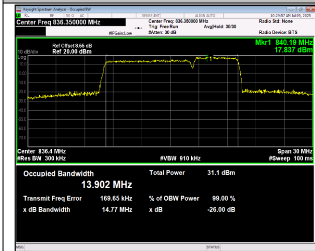
5-5-10MHz-5MHz-QPSK-QPSK-20550-20622-50RB#0-25 RB#0-PASS
