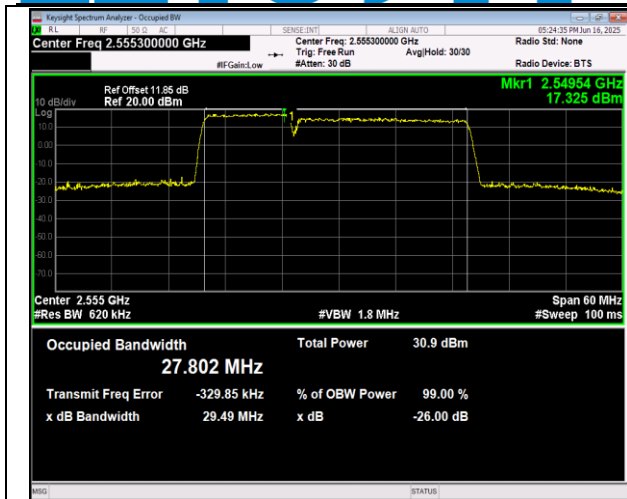
7-7-15MHz-10MHz-QPSK-QPSK-20825-20945-75RB#0-5 ORB#0-PASS
