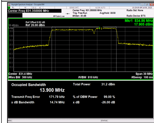
5-5-10MHz-5MHz-QPSK-QPSK-20500-20572-50RB#0-25 RB#0-PASS
