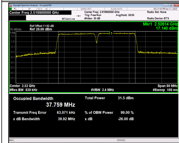
7-7-20MHz-20MHz-QPSK-QPSK-21001-21199-100RB#0-100RB#0-PASS
