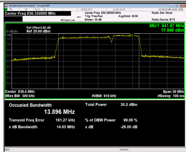
5-5-10MHz-5MHz-16QAM-16QAM-20550-20622-50RB#0-2 5RB#0-PASS
