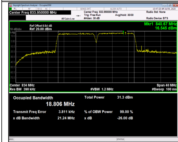
5-5-10MHz-10MHz-QPSK-QPSK-20476-20575-50RB#0-5 ORB#0-PASS
