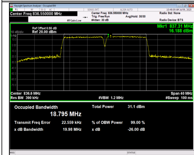
5-5-10MHz-10MHz-QPSK-QPSK-20501-20600-50RB#0-5 ORB#0-PASS
