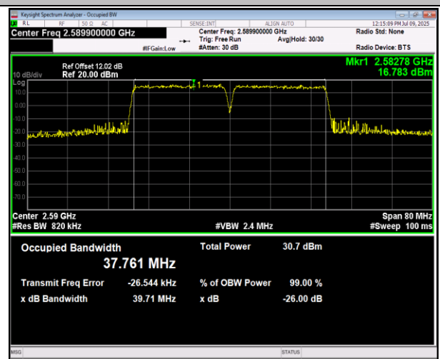
38-38-20MHz-20MHz-16QAM-16QAM-37901-38099-100RB B#0-100RB#0-PASS
