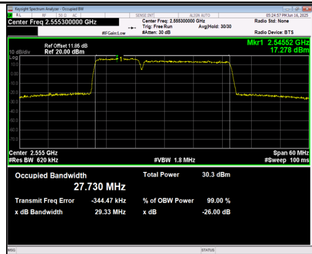
7-7-15MHz-10MHz-16QAM-16QAM-20825-20945-75RB#0-50 50RB#0-PASS
