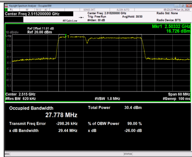
7-7-10MHz-20MHz-16QAM-16QAM-21006-21150-50RB#0- 100RB#0-PASS
