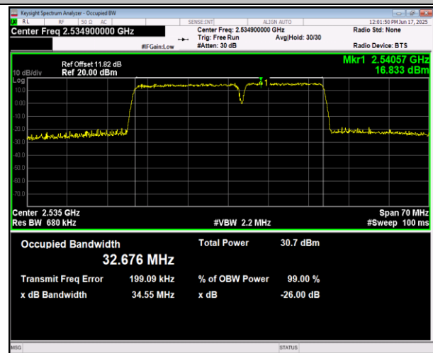
7-7-20MHz-15MHz-16QAM-16QAM-21201-21372-100RB#0-75RB#0-PASS
