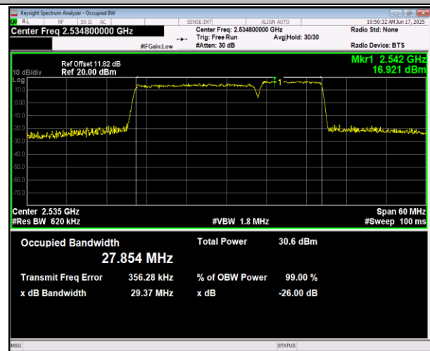
7-7-20MHz-10MHz-16QAM-16QAM-21251-21395-100RB#0-50RB#0-PASS
