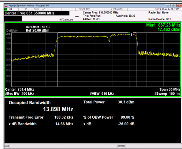
5-5-10MHz-5MHz-16QAM-16QAM-20500-20572-50RB#0-2 5RB#0-PASS
