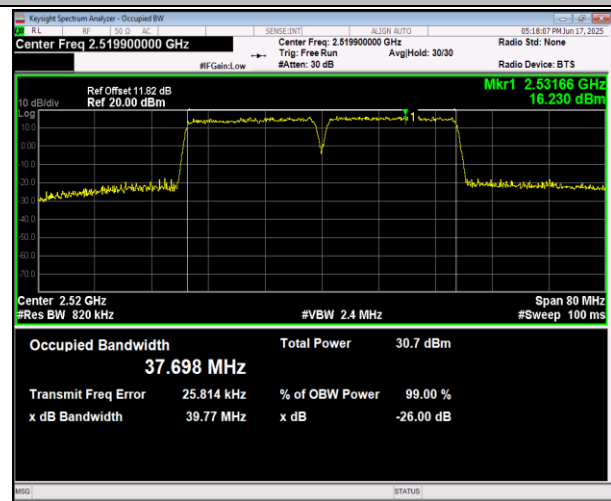
7-7-20MHz-20MHz-16QAM-16QAM-21001-21199-100RB#0-100RB#0-PASS
