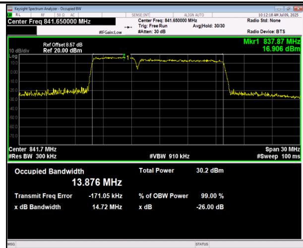
5-5-10MHz-5MHz-16QAM-16QAM-20450-20522-50RB#0-2 5RB#0-PASS
