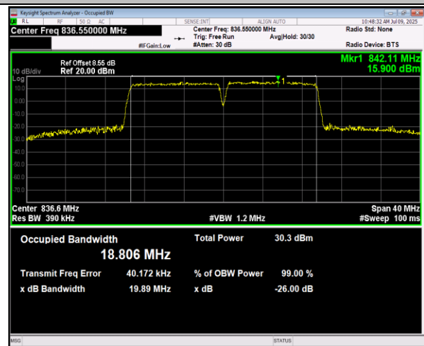
5-5-10MHz-10MHz-16QAM-16QAM-20501-20600-50RB#0-5 50RB#0-PASS
