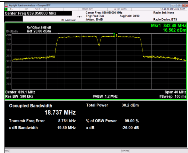
7-7-10MHz-20MHz-16QAM-16QAM-20805-20949-50RB#0- 100RB#0-PASS
