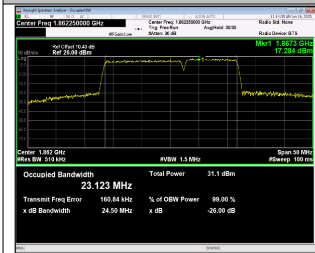
2-2-15MHz-10MHz-QPSK-QPSK-18851-18971-75RB#0-5 ORB#0-PASS
