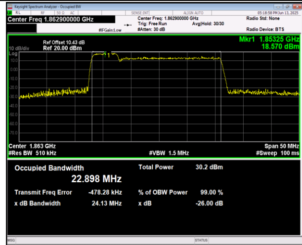
2-2-5MHz-20MHz-16QAM-16QAM-18808-18925-25RB#0-1 00RB#0-PASS
