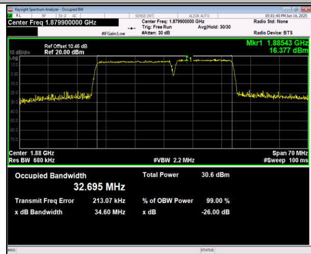
2-2-20MHz-15MHz-16QAM-16QAM-18951-19122-100RB#0-75RB#0-PASS
