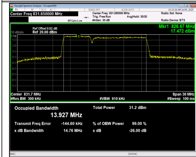
5-5-5MHz-10MHz-QPSK-QPSK-20478-20550-25RB#0-50 RB#0-PASS
