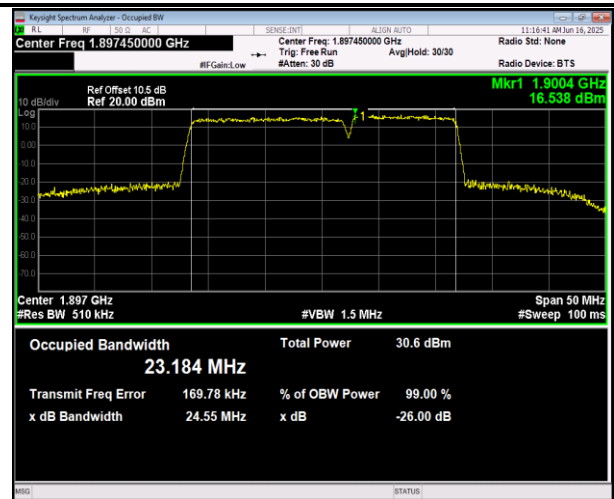
2-2-15MHz-15MHz-16QAM-16QAM-18675-18825-75RB#0-7 75RB#0-PASS
