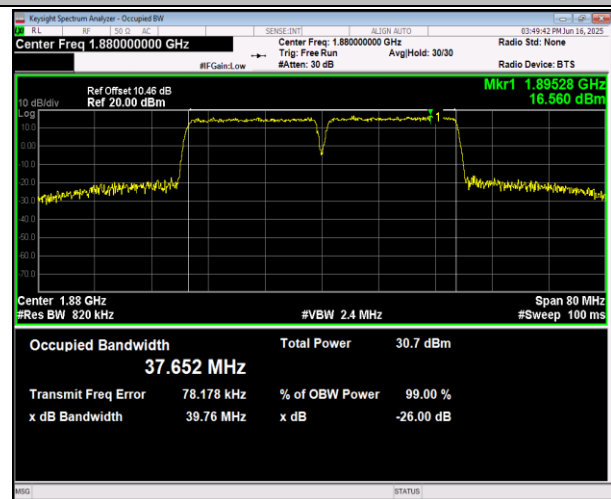
2-2-20MHz-20MHz-16QAM-16QAM-18902-19100-100RB#0-100RB#0-PASS
