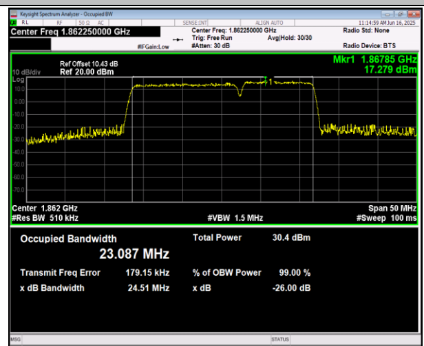
2-2-15MHz-10MHz-16QAM-16QAM-18851-18971-75RB#0- 50RB#0-PASS
