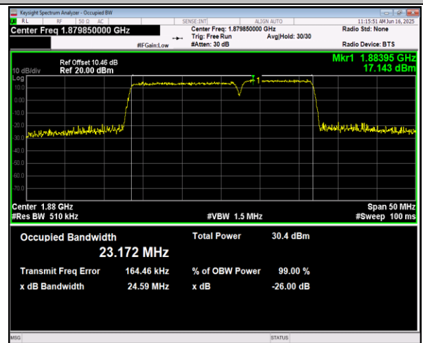
2-2-15MHz-10MHz-16QAM-16QAM-19027-19147-75RB#0- 50RB#0-PASS
