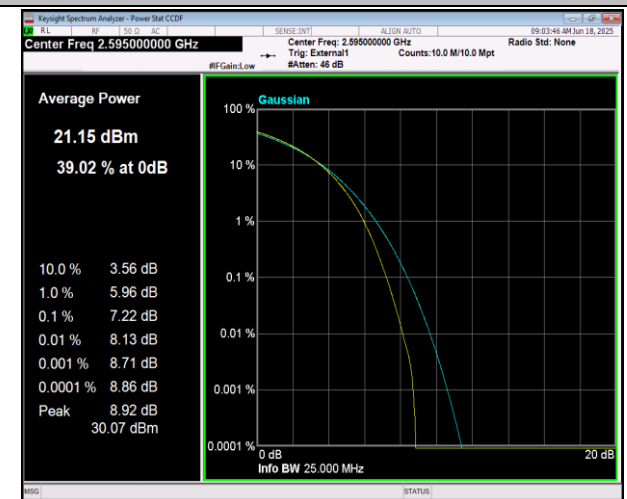
38-38-15MHz-15MHz-16QAM-16QAM-38025-38175-75RB #0-75RB#0-PASS
