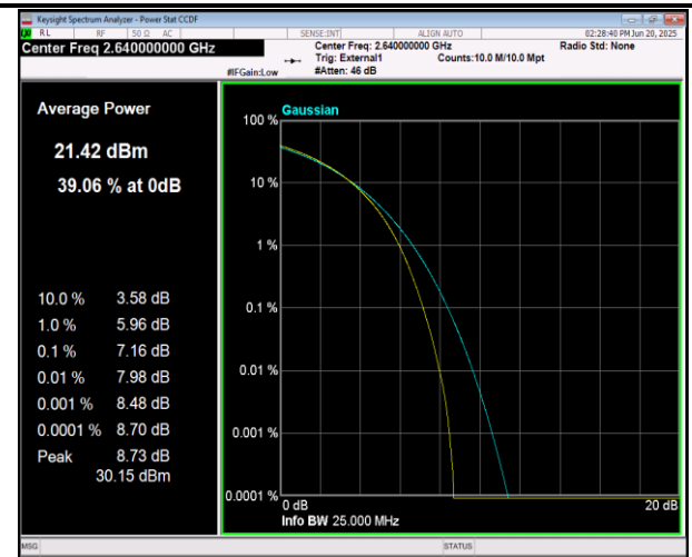
41(2555-2655)-41(2555-2655)-15MHz-20MHz-16QAM-16 QAM-40318-40489-75RB#0-100RB#0-PASS
