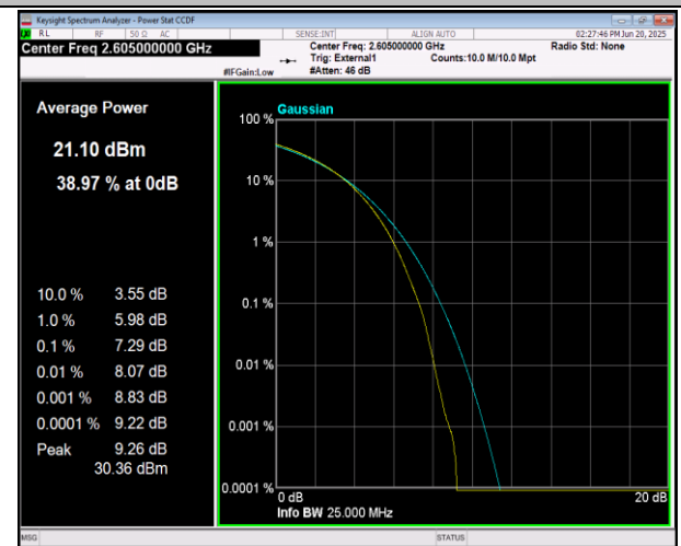
41(2555-2655)-41(2555-2655)-15MHz-15MHz-16QAM-16 QAM-41015-41165-75RB#0-75RB#0-PASS
