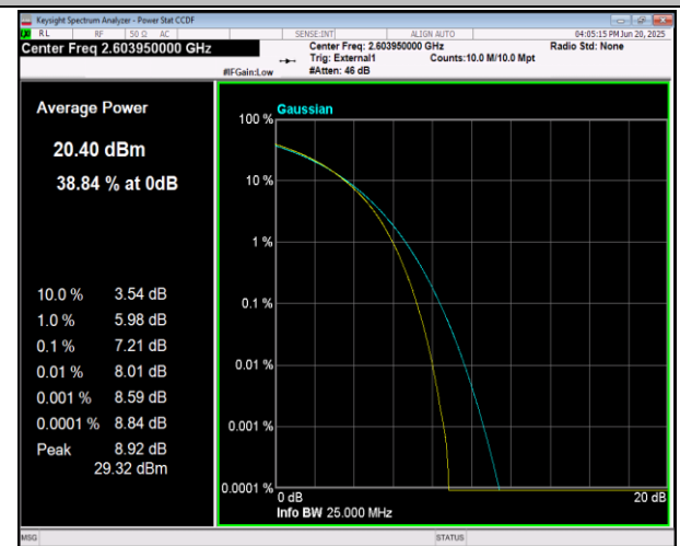
41(2555-2655)-41(2555-2655)-15MHz-20MHz-16QAM-16 QAM-40969-41140-75RB#0-100RB#0-PASS
