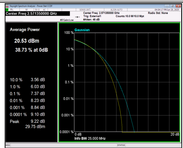
41(2555-2655)-41(2555-2655)-15MHz-20MHz-16QAM-16 QAM-40644-40815-75RB#0-100RB#0-PASS
