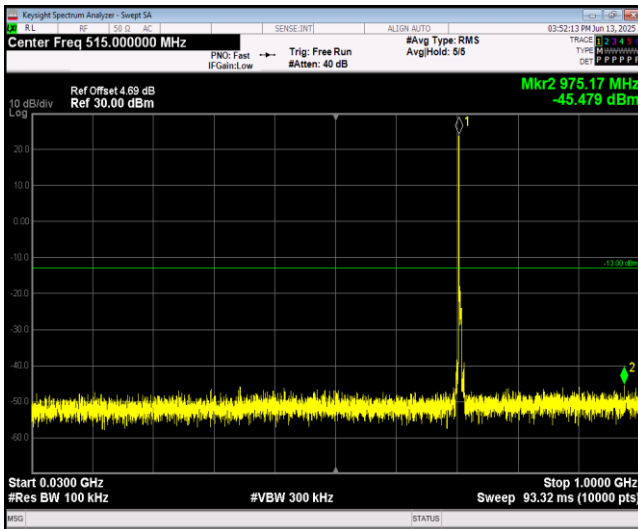
Band17-5MHz-64QAM-23755-1RB#0-Range1:30~1000MHz
