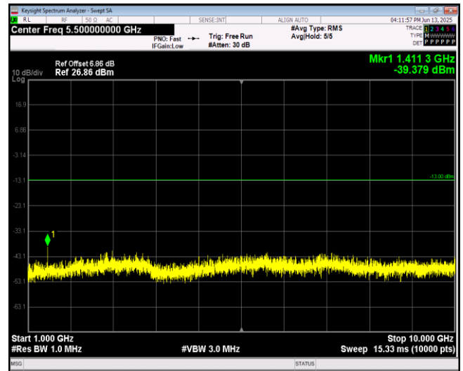
Band17-10MHz-QPSK-23800-1RB#0-Range2:1000~10000MHz
