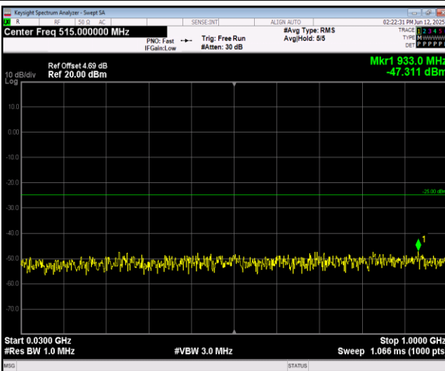
Band38-5MHz-16QAM-38000-1RB#0-Range1:30~10 00MHz
