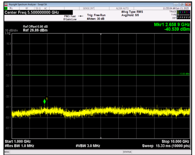
Band5-10MHz-64QAM-20450-1RB#0-Range2:1000~10000MHz
