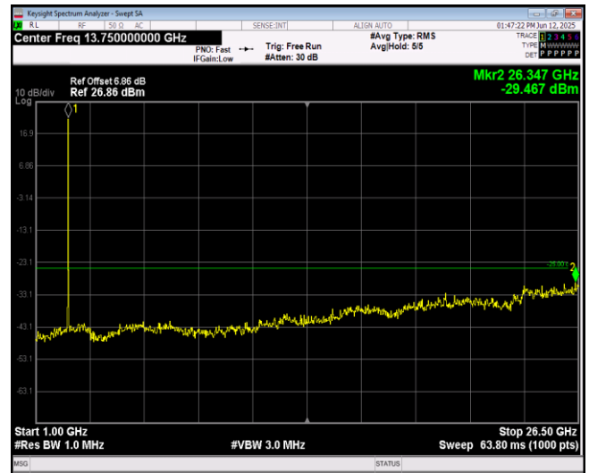
Band7-20MHz-64QAM-21350-1RB#0-Range2:1000~26500MHz
