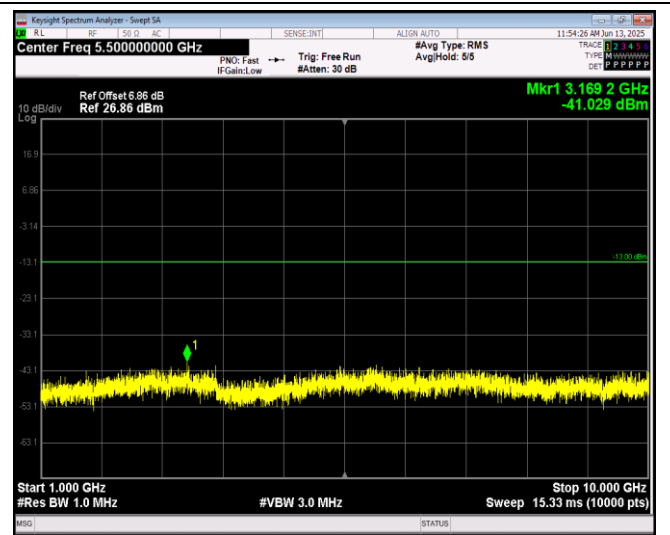
Band5-10MHz-64QAM-20600-1RB#0-Range2:1000~10000MHz
