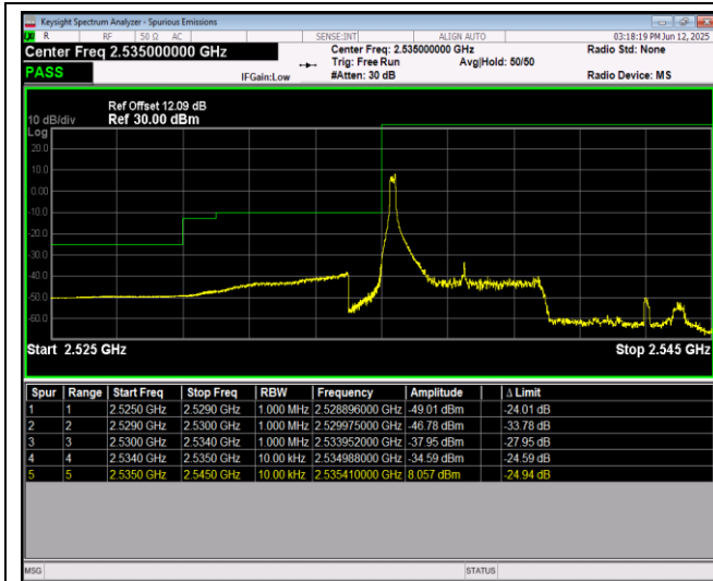
Band41-5MHz-64QAM-40065-25RB#0
