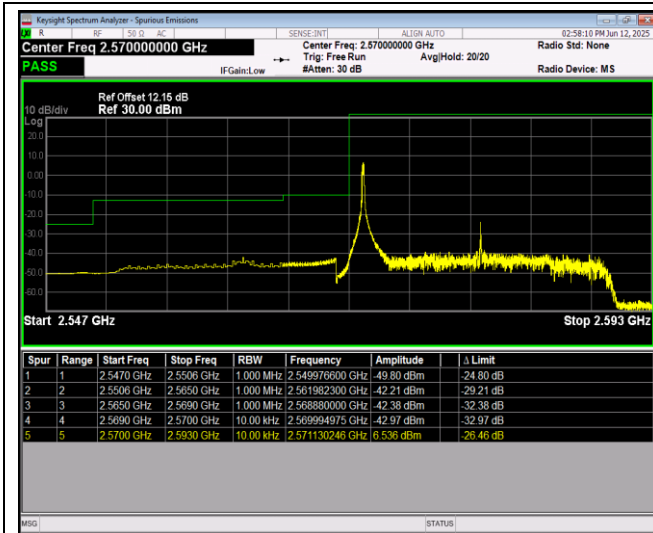
Band38-20MHz-64QAM-37850-100RB#0
