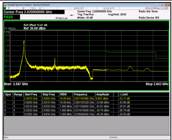
Band38-20MHz-64QAM-38150-100RB#0
