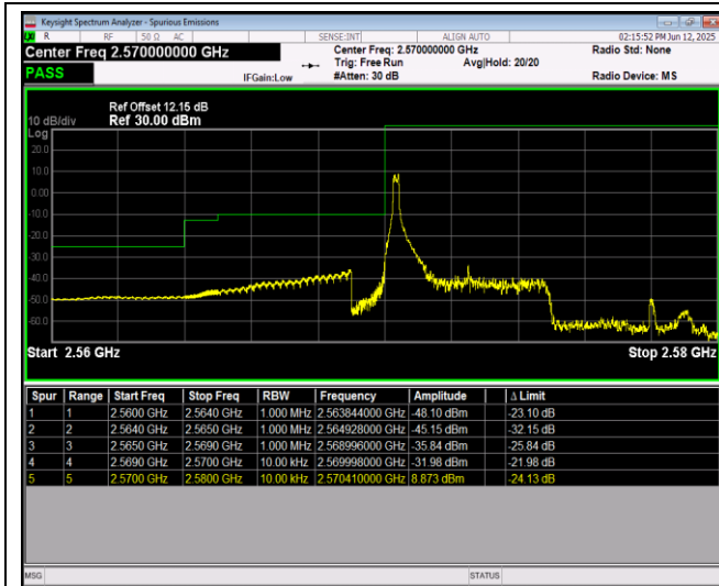
Band38-5MHz-QPSK-37775-25RB#0
