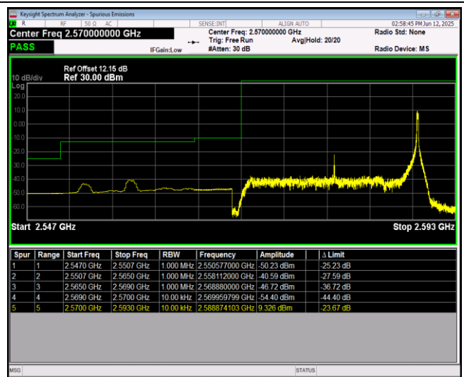
Band38-20MHz-16QAM-38150-1RB#0
