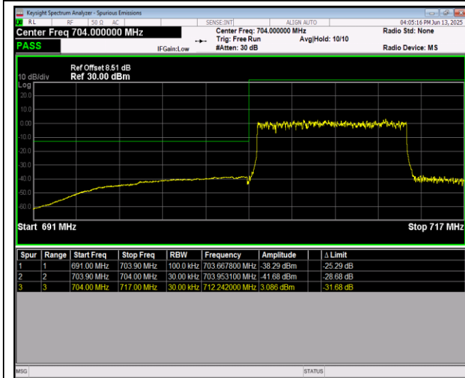
Band17-10MHz-QPSK-23800-1RB#49
