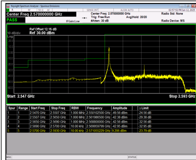
Band38-20MHz-16QAM-37850-100RB#0
