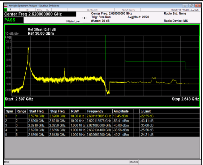
Band38-20MHz-16QAM-38150-100RB#0
