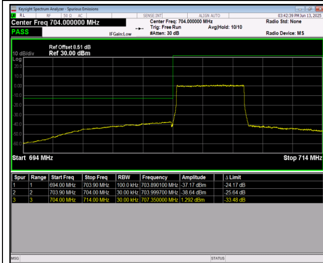
Band17-5MHz-QPSK-23825-1RB#24
