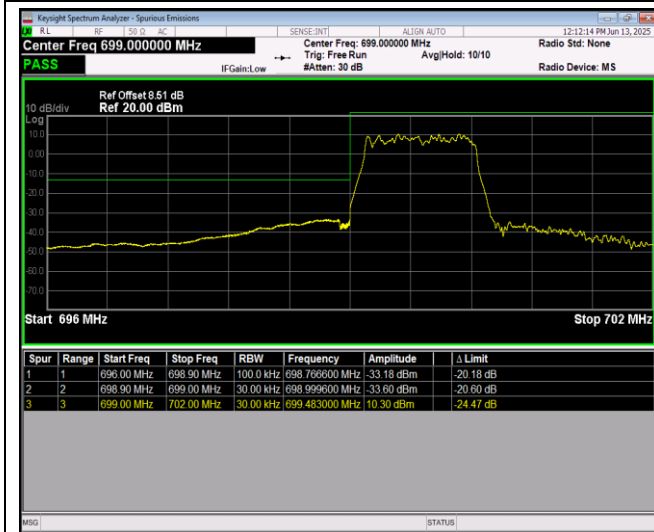
Band12-1.4MHz-16QAM-23173-1RB#5
