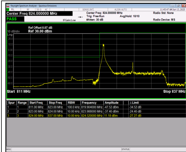
Band5-10MHz-64QAM-20450-50RB#0
