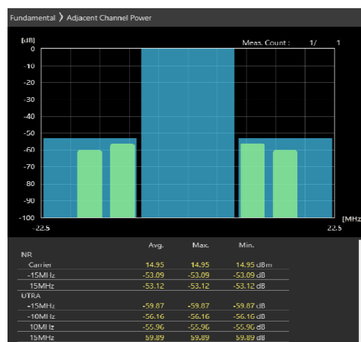
15MHz_30kHz_3692.5MHz-OFDM QPSK_RB36@0 -53.09,-53.12dB
