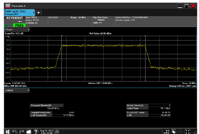
n77_2_15MHz_30kHz_3625MHz_CP-OFDM 256 QAM_RB38@0 13.529MHz
