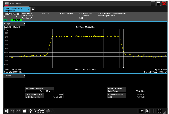
n77_2_15MHz_30kHz_3625MHz_CP-OFDM 16 QAM_RB38@0 13.580MHz
