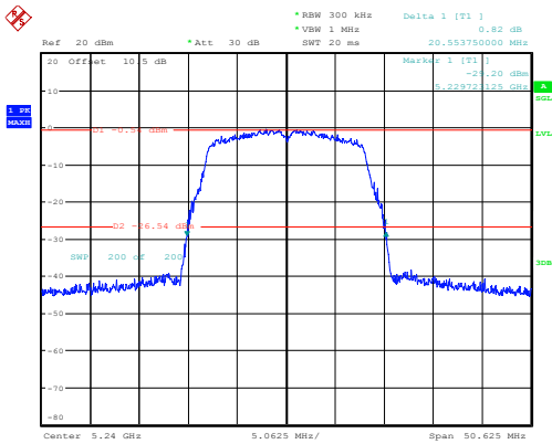
a_5240MHz_Chain 0 20.554MHz
