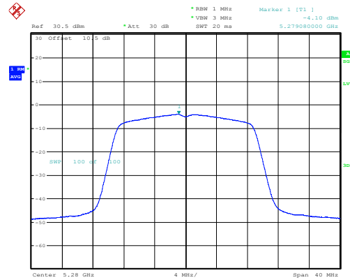
n20_5280MHz_Chain 0 -4.10dBm/MHz
