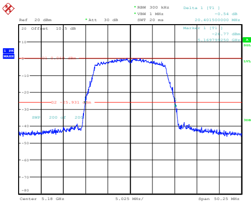
a_5180MHz_Chain 0 20.402MHz
