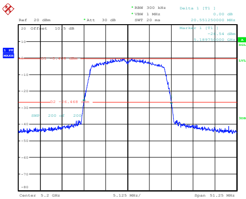
n20_5200MHz_Chain 0 20.551MHz
