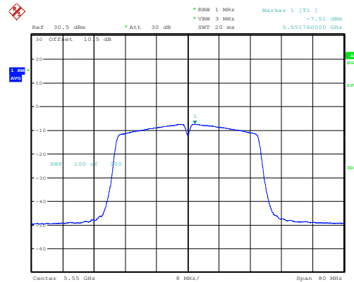
n40_5550MHz_Chain 0 -7.51dBm/MHz
