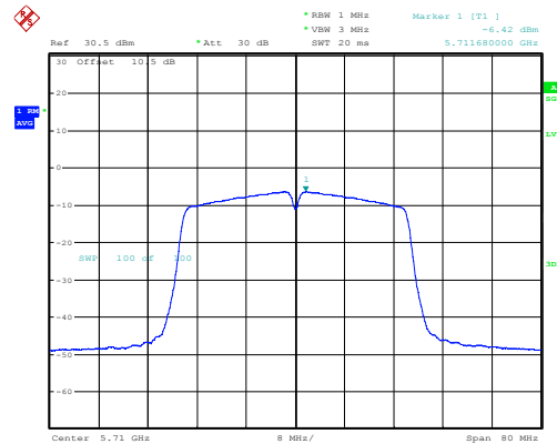
n40_5710MHz_Chain 0 -6.42dBm/MHz
