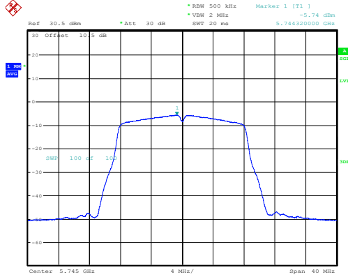
a_5745MHz_Chain 0 -5.74dBm/MHz
