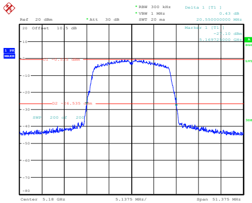
n20_5180MHz_Chain 0 20.550MHz
