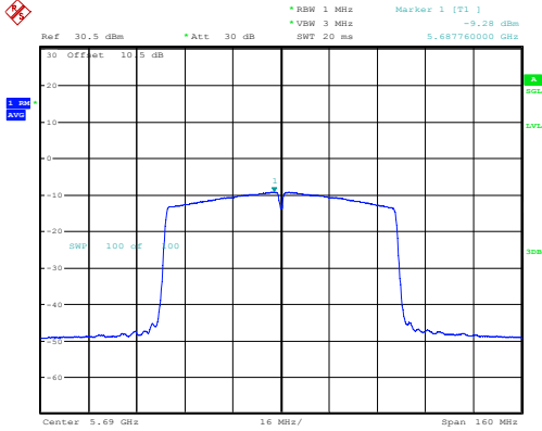
ac80_5690MHz_Chain 0 -9.28dBm/MHz
