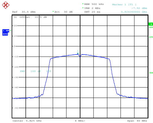
n20_5825MHz_Chain 0 -7.92dBm/MHz
