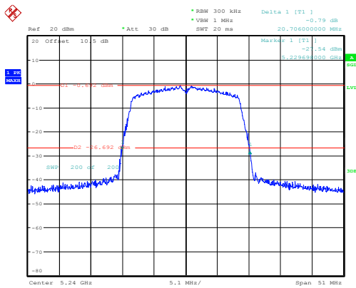
n20_5240MHz_Chain 0 20.706MHz
