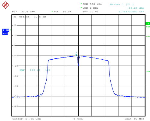
n40_5795MHz_Chain 0 -10.29dBm/MHz
