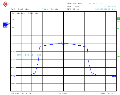
n40_5755MHz_Chain 0 -9.41dBm/MHz
