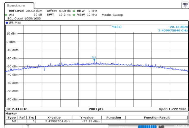
Middle -23.15dBm/3kHz
