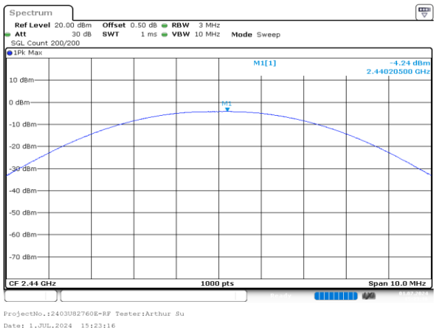
Middle -4.24dBm
