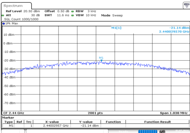
Middle -21.14dBm/3kHz
