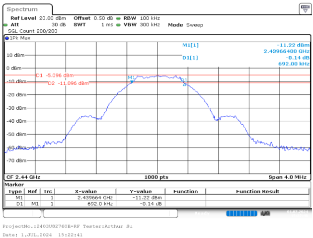
Middle 0.692MHz
