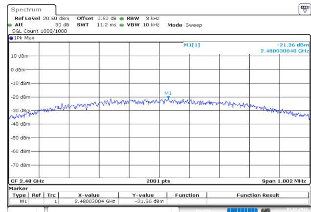
High -21.36dBm/3kHz
