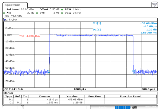
8DPSK_Hopping_3DH3 1.659ms
