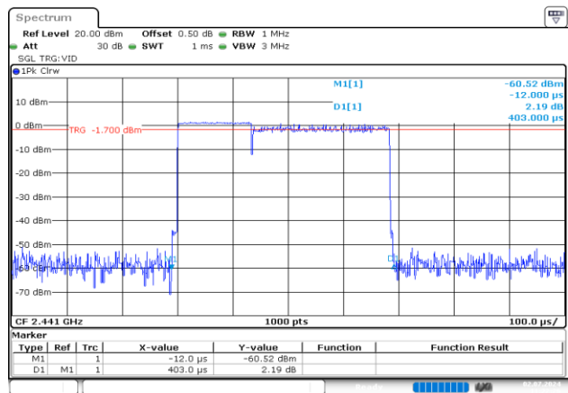
8DPSK_Hopping_3DH1 0.403ms
