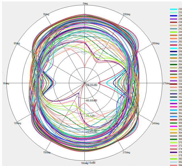
LTE B7/B38/B40/B41/B42 NR n7/n38/n40/n41/n77/n78 Theta=90deg
