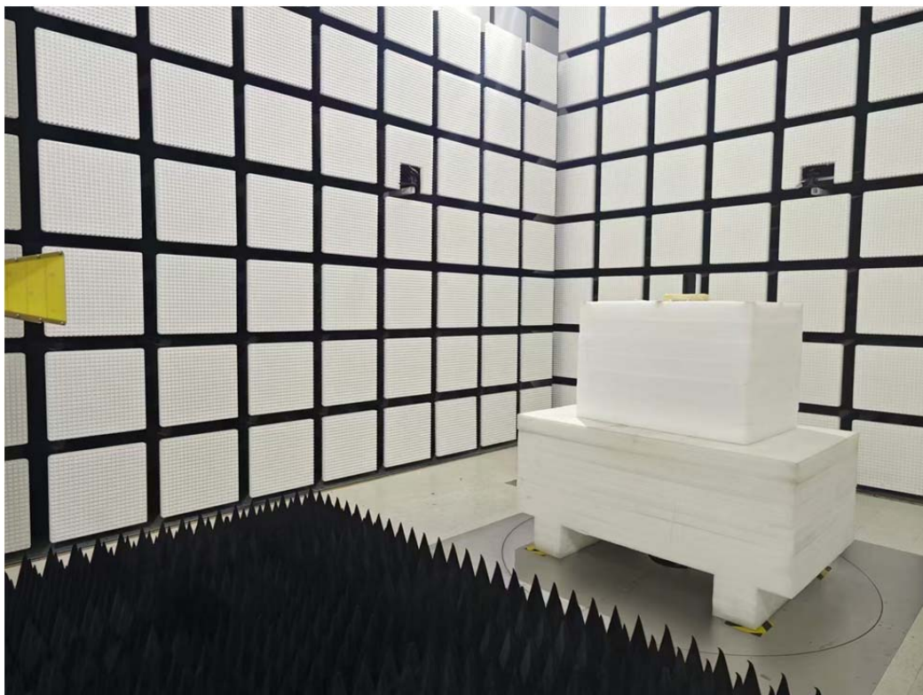
Radiated Emission Above 1GHz View 1-18G
