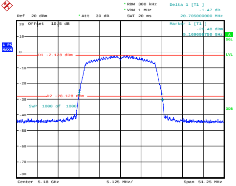
n20_5180MHz 20.705MHz
