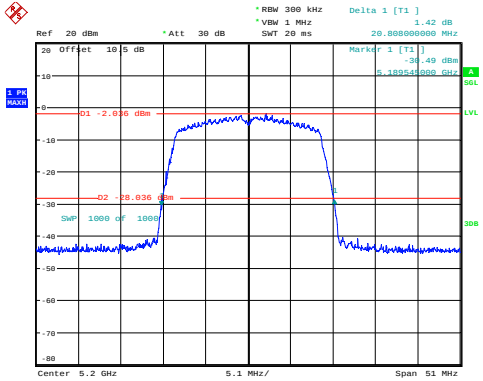
n20_5200MHz 20.808MHz
