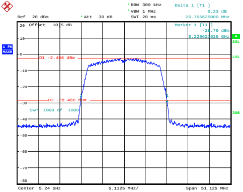
n20_5240MHz 20.706MHz
