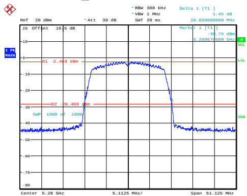
n20_5280MHz 20.859MHz
