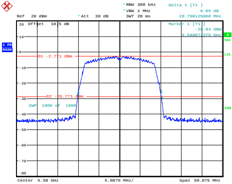
n20_5580MHz 20.706MHz
