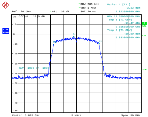
n20_5825MHz 17.650MHz
