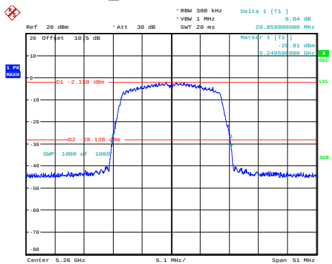
n20_5260MHz 20.859MHz
