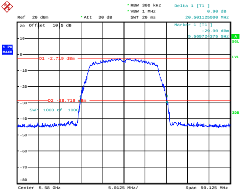
a_5580MHz 20.501MHz
