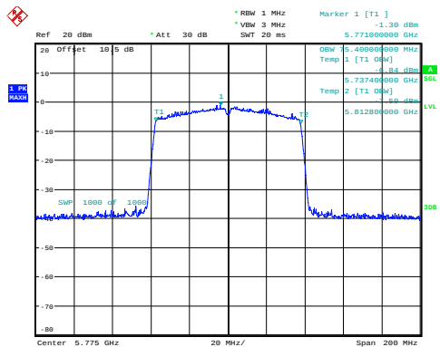
ac80_5775MHz 75.400MHz
