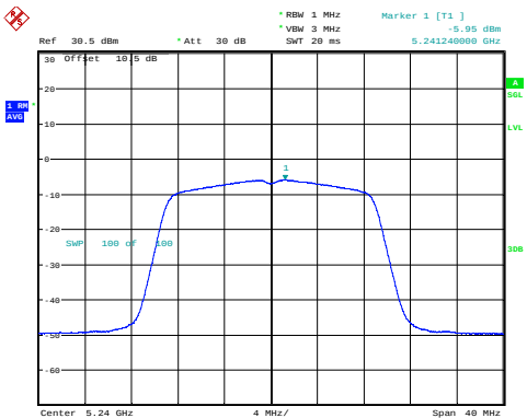
n20_5240MHz -5.95dBm/MHz
