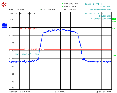
n20_5320MHz 20.859MHz
