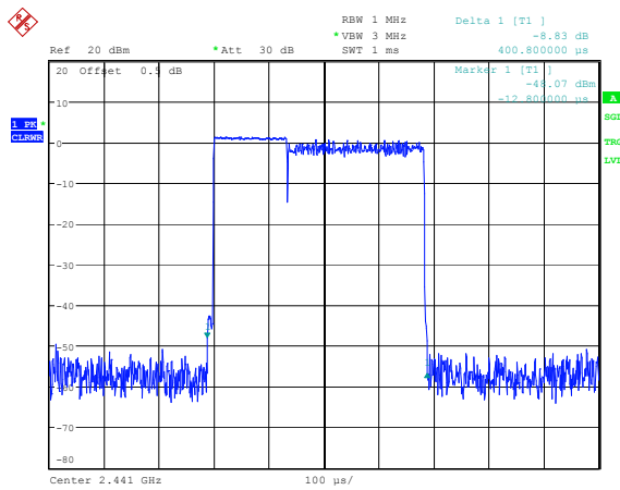
8DPSK_Hopping_3DH1 0.401ms
