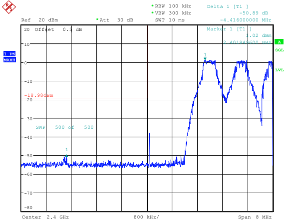
GFSK_Hopping_Lower 50.89dB
