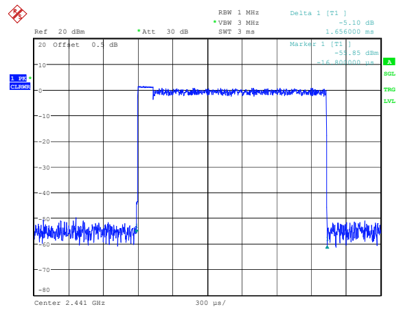
8DPSK_Hopping_3DH3 1.656ms
