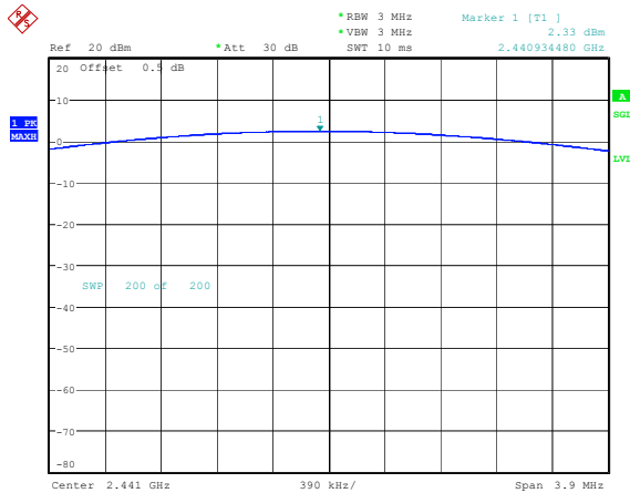
GFSK_Middle 2.33dBm
