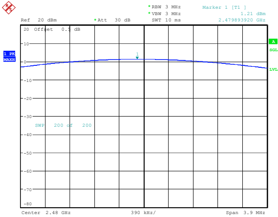
GFSK_High 1.21dBm
