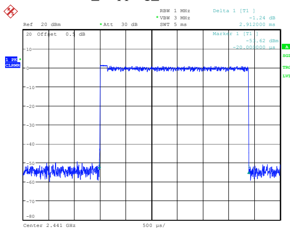
8DPSK_Hopping_3DH5 2.912ms
