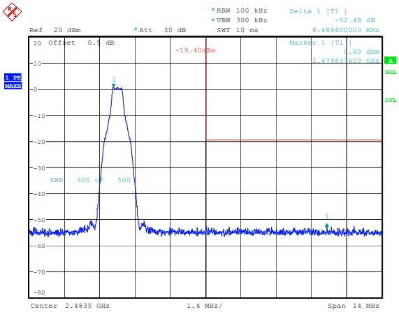
GFSK_High 52.48dB
