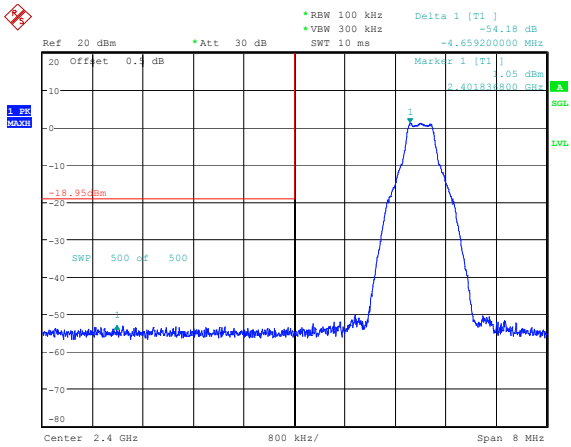
GFSK_Low 54.18dB
