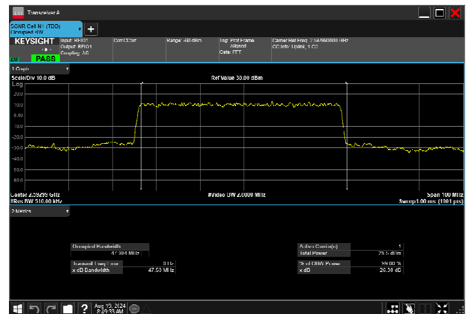
n41_50MHz_30kHz_2592.99MHz_DFT-s-OFDM 16 QAM_RB128@0 47.051MHz
