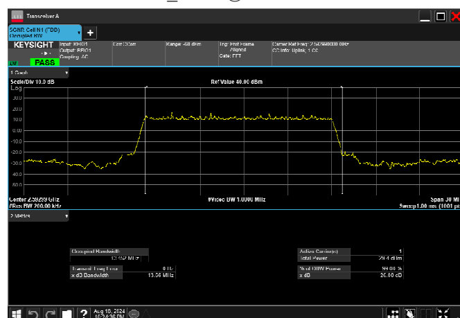
n41_15MHz_30kHz_2592.99MHz_DFT-s-OFDM 16 QAM RB36@0 13.503MHz
