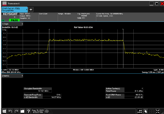
n12_15MHz_15kHz_707.5MHz_CP-OFDM 16 QAM_RB79@0 14.103MHz
