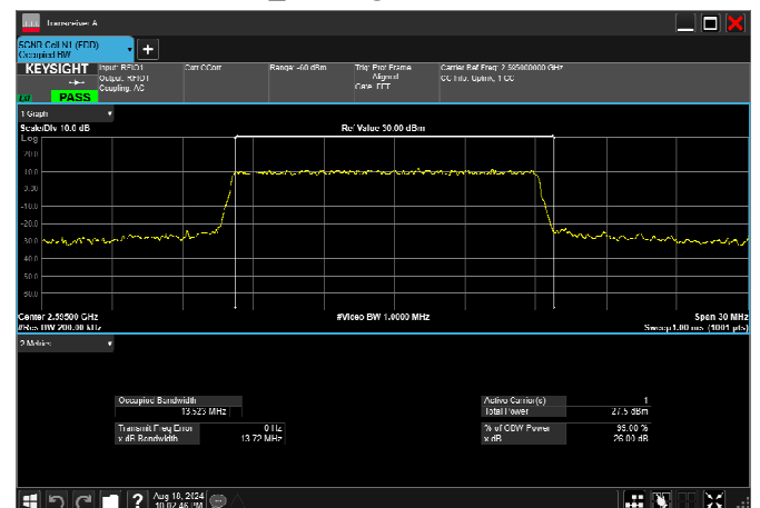
n38_15MHz_30kHz_2595MHz_DFT-s-OFDM 16 QAM_RB36@0 13.523MHz
