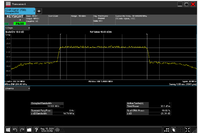
n12_15MHz_15kHz_707.5MHz_CP-OFDM 64 QAM_RB79@0 14.059MHz
