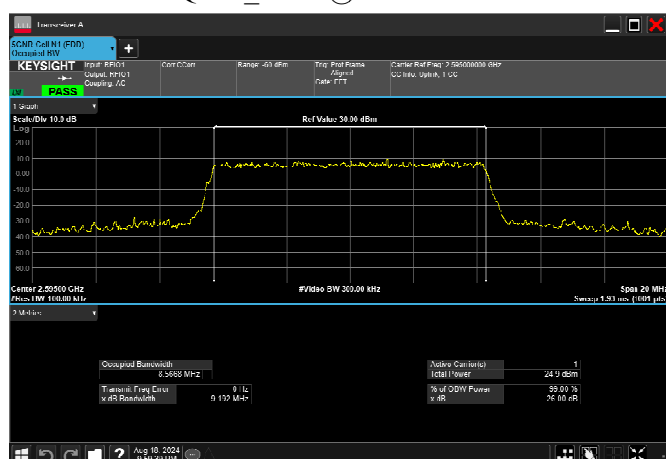
n38_10MHz_30kHz_2595MHz_DFT-s-OFDM 256 QAM_RB24@0 8.567MHz
