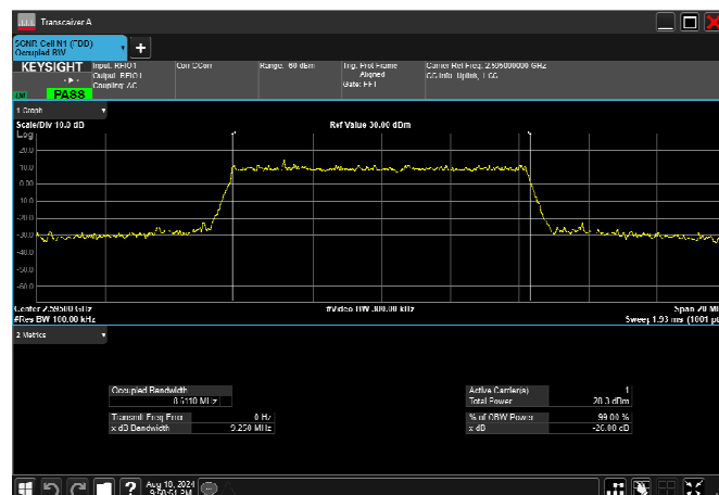
n38_10MHz_30kHz_2595MHz_DFT-s-OFDM 64 QAM_RB24@0 8.604MHz
