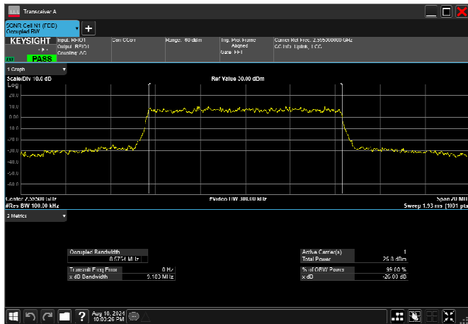
n38_10MHz_30kHz_2595MHz_CP-OFDM 256 QAM_RB24@0 8.611MHz
