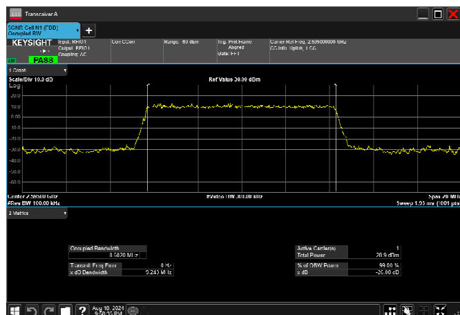
n38_10MHz_30kHz_2595MHz_DFT-s-OFDM 16 QAM_RB24@0 8.574MHz
