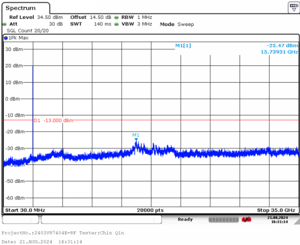
1_10MHz_High_QPSK_1@0
