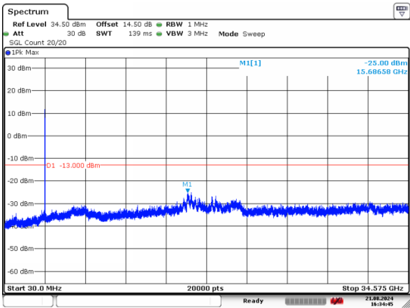
1_15MHz_Low_QPSK_75@0
