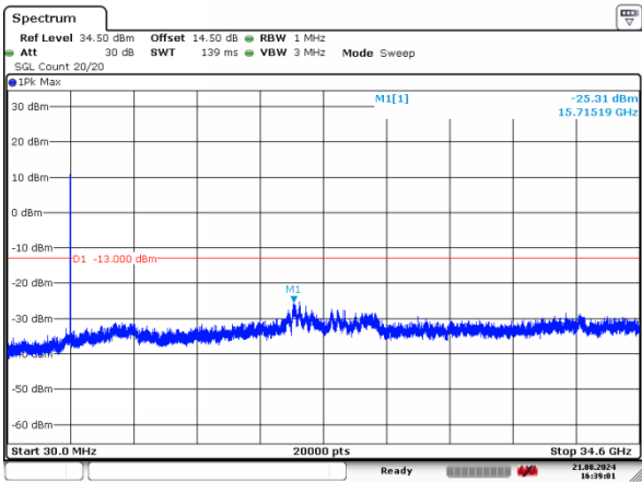
1_20MHz_Low_QPSK_100@0
