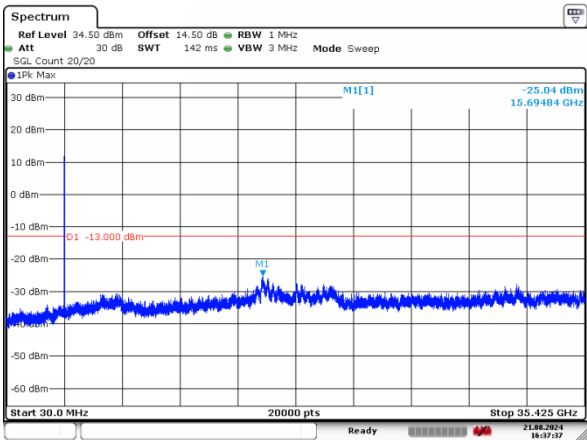
1_15MHz_High_QPSK_75@0
