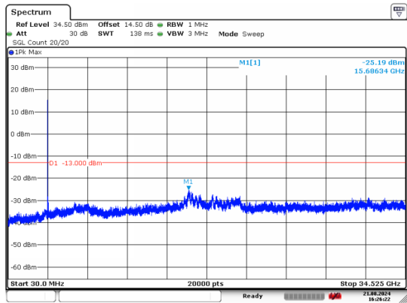
1_5MHz_Low_QPSK_25@0
