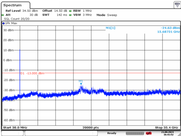
1_20MHz_High_QPSK_100@0
