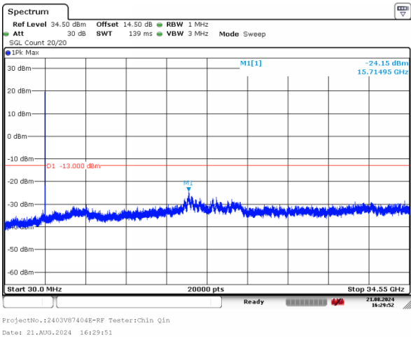
1_10MHz_Middle_QPSK_1@0
