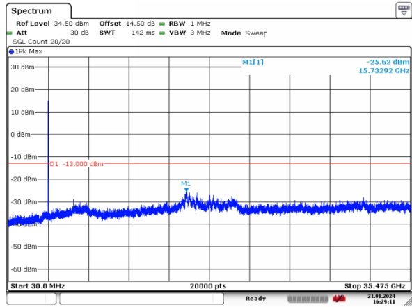
1_5MHz_High_QPSK_25@0
