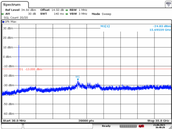
1_20MHz_Middle_QPSK_100@0
