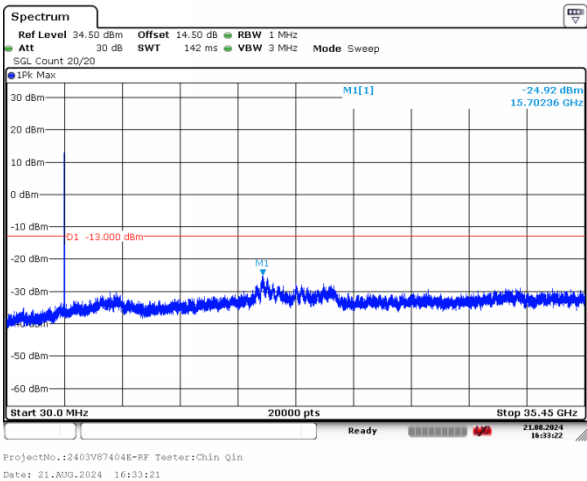
1_10MHz_High_QPSK_50@0
