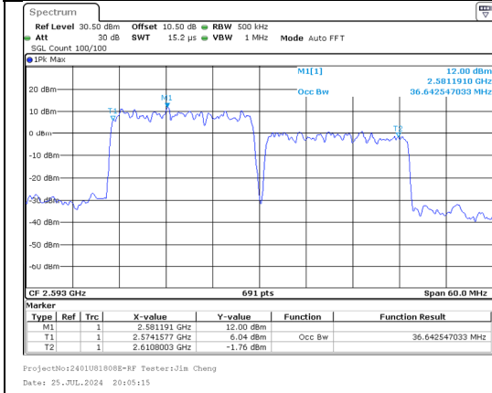
99%OBW Band 41 20MHz/2583.1/Mid QPSK 100@0 Band 41 20MHz/2602.9/Mid QPSK 100@0
