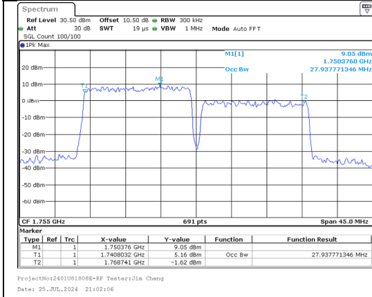
99%OBW Band 66 15MHz/1747.5/Mid 256QAM 75@0 Band 66 15MHz/1762.5/Mid 256QAM 75@0
