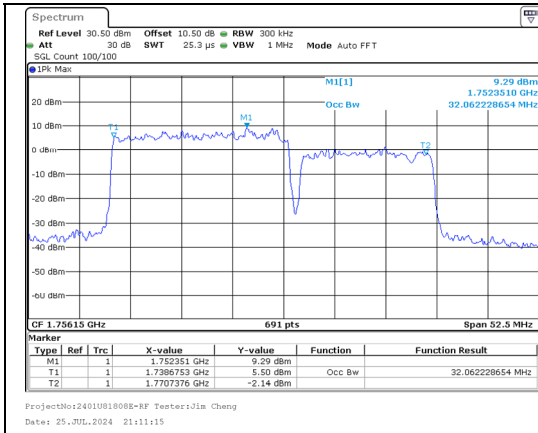
99%OBW Band 66 20MHz/1747.6/Mid 256QAM 100@0 Band 66 15MHz/1764.7/Mid 256QAM 75@0
