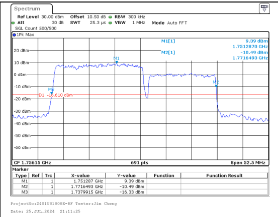
26%OBW Band 66 20MHz/1747.6/Mid 256QAM 100@0 Band 66 15MHz/1764.7/Mid 256QAM 75@0
