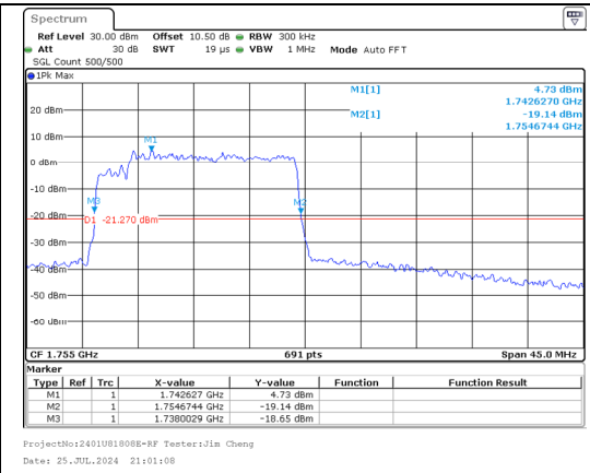
26%OBW Band 66 15MHz/1747.5/Mid 64QAM 75@0 Band 66 15MHz/1762.5/Mid 64QAM 75@0
