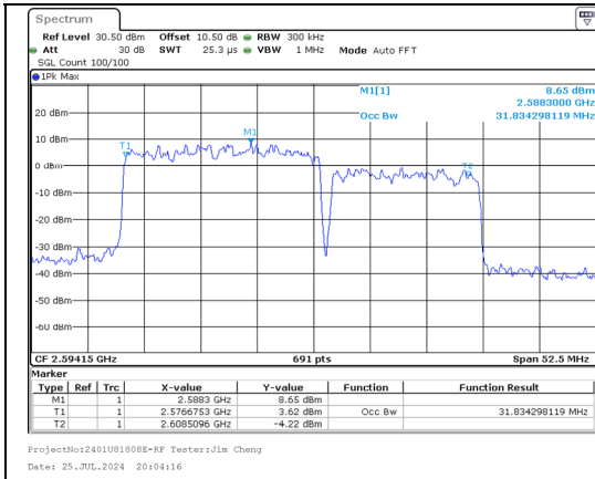
99%OBW Band 41 20MHz/2585.6/Mid 256QAM 100@0 Band 41 15MHz/2602.7/Mid 256QAM 75@0
