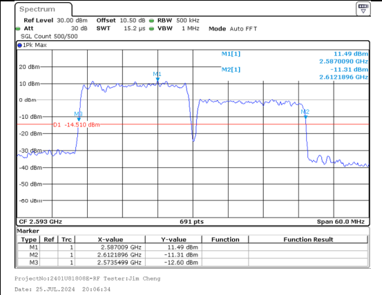
26%OBW Band 41 20MHz/2583.1/Mid 16QAM 100@0 Band 41 20MHz/2602.9/Mid 16QAM 100@0
