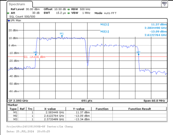
26%OBW Band 41 20MHz/2583.1/Mid QPSK 100@0 Band 41 20MHz/2602.9/Mid QPSK 100@0
