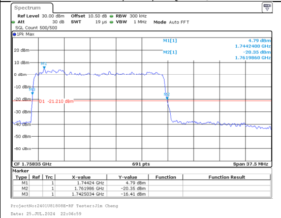
26%OBW Band 66 20MHz/1752.5/Mid 16QAM 100@0 Band 66 5MHz/1764.2/Mid 16QAM 25@0
