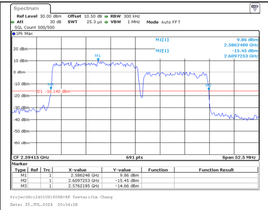
26%OBW Band 41 20MHz/2585.6/Mid 256QAM 100@0 Band 41 15MHz/2602.7/Mid 256QAM 75@0
