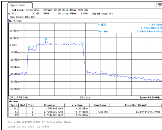
99%OBW Band 66 15MHz/1747.5/Mid 64QAM 75@0 Band 66 15MHz/1762.5/Mid 64QAM 75@0
