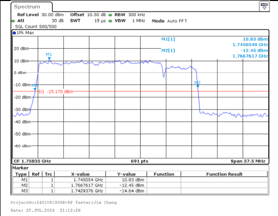
26%OBW Band 66 20MHz/1752.5/Mid QPSK 100@0 Band 66 5MHz/1764.2/Mid QPSK 25@0
