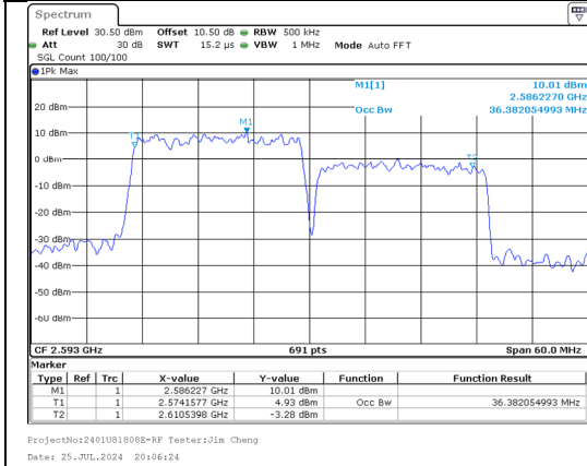
99%OBW Band 41 20MHz/2583.1/Mid 16QAM 100@0 Band 41 20MHz/2602.9/Mid 16QAM 100@0
