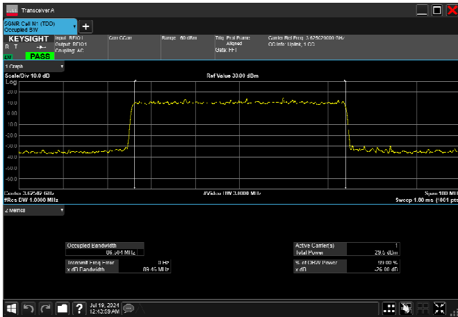
n78_2_90MHz_30kHz_3625MHz_DFT-s-OFDM 16 QAM_RB243@0 86.514MHz
