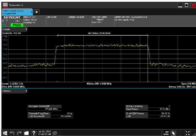
n78_2_80MHz_30kHz_3625MHz_CP-OFDM 64 QAM_RB217@0 77.245MHz
