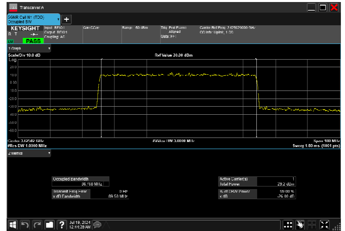
n78_2_90MHz_30kHz_3625MHz_DFT-s-OFDM 64 QAM_RB243@0 86.814MHz
