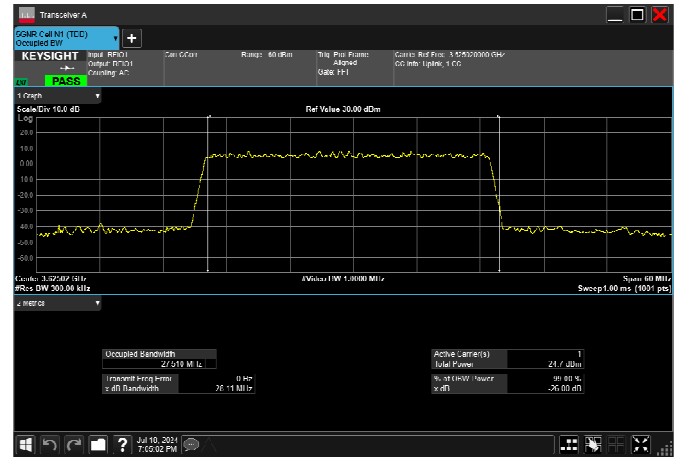
n77_2_30MHz_30kHz_3625MHz_CP-OFDM 16 QAM_RB78@0 27.765MHz
