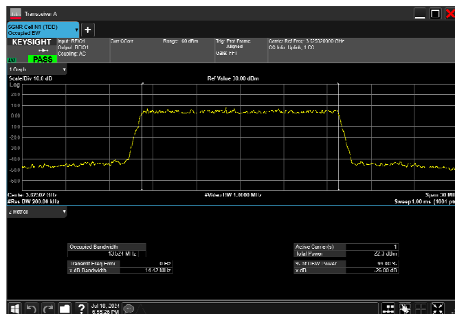
n77_2_15MHz_30kHz_3625MHz_CP-OFDM 256 QAM_RB38@0 13.524MHz
