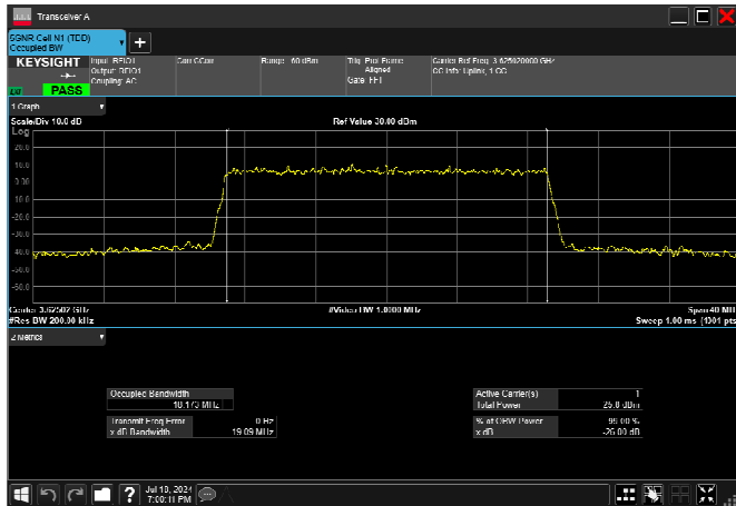
n77_2_20MHz_30kHz_3625MHz_CP-OFDM 256 QAM_RB51@0 18.182MHz
