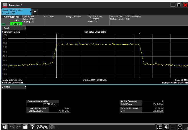
n77_2_30MHz_30kHz_3625MHz_CP-OFDM 64 QAM_RB78@0 27.749MHz
