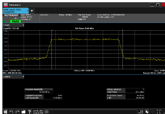
n77_2_15MHz_30kHz_3625MHz_CP-OFDM 16 QAM_RB38@0 13.577MHz
