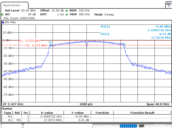
n20_2437MHz_Chain 0
