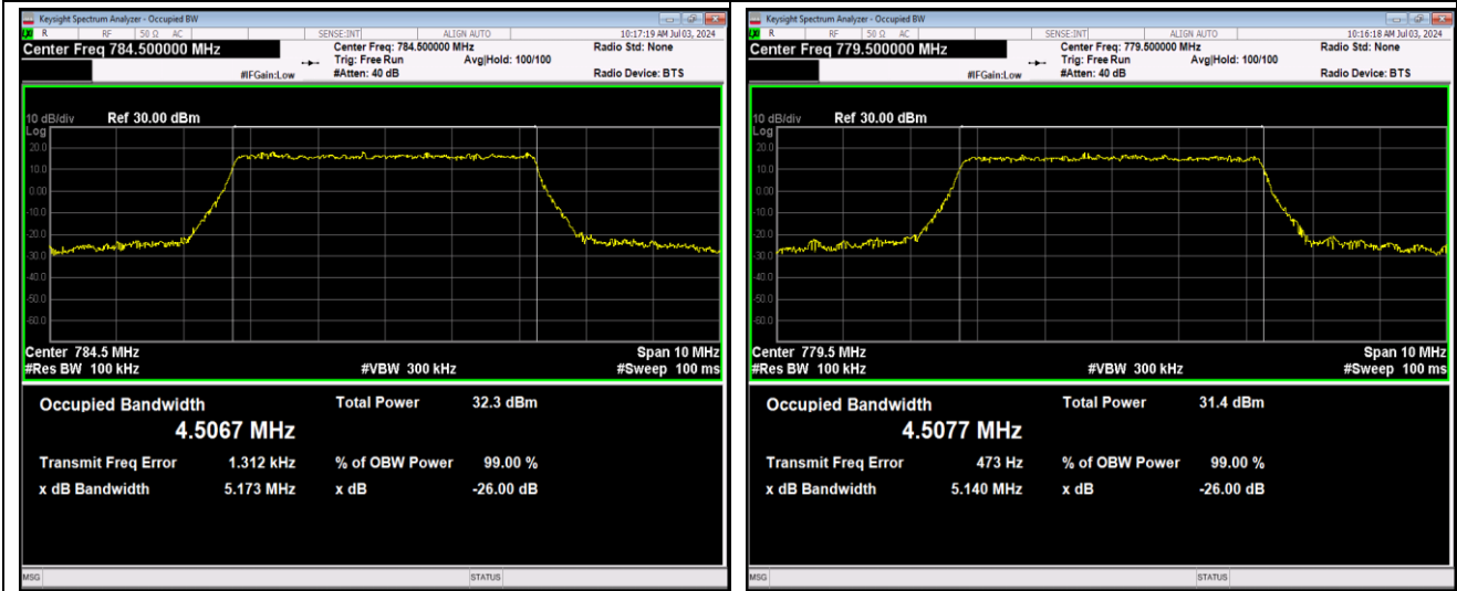
Band13-5MHz-16QAM-23230-25RB#0
