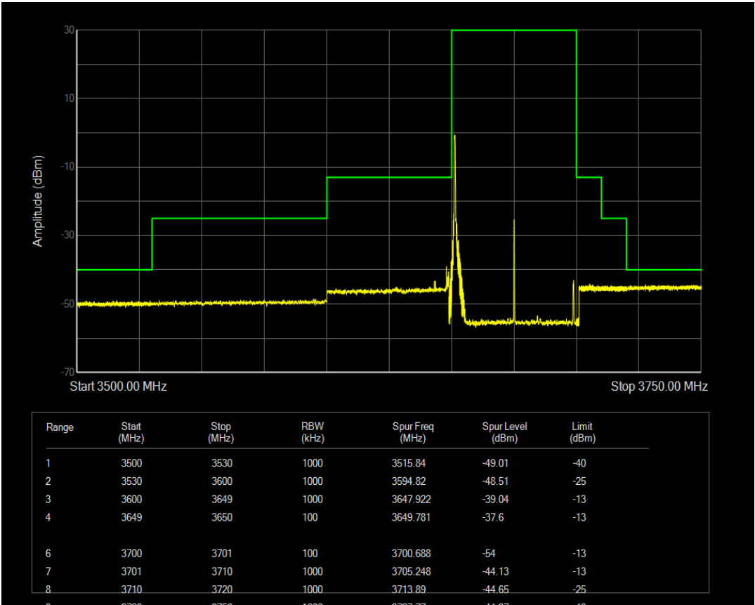
n77(3550-3700) SCS=30kHz CP_QPSK BW=50MHz Channel=645000 RB=1@132
