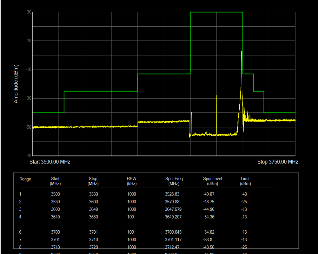
n77(3550-3700) SCS=30kHz CP_QPSK BW=100MHz Channel=640000 RB=1@@
