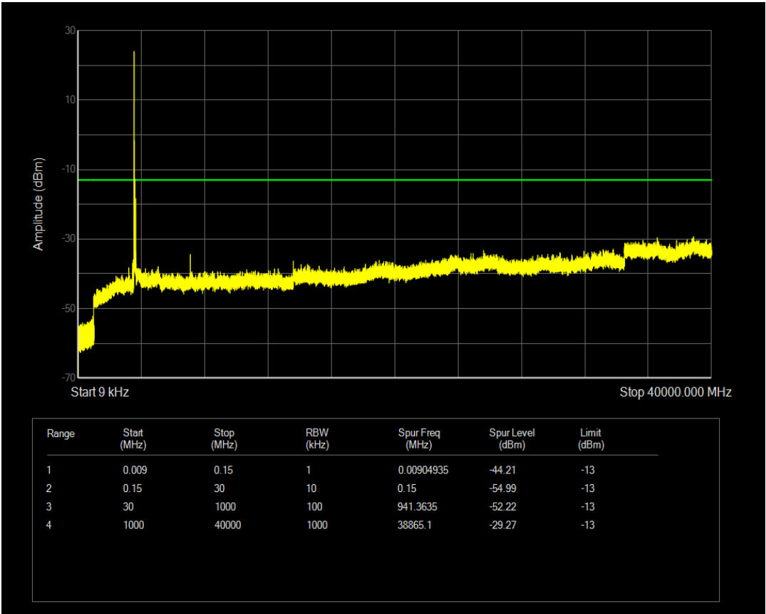
n77(3550-3700) SCS=30kHz CP_QPSK BW=100MHz Channel=643332 RB=1@0
