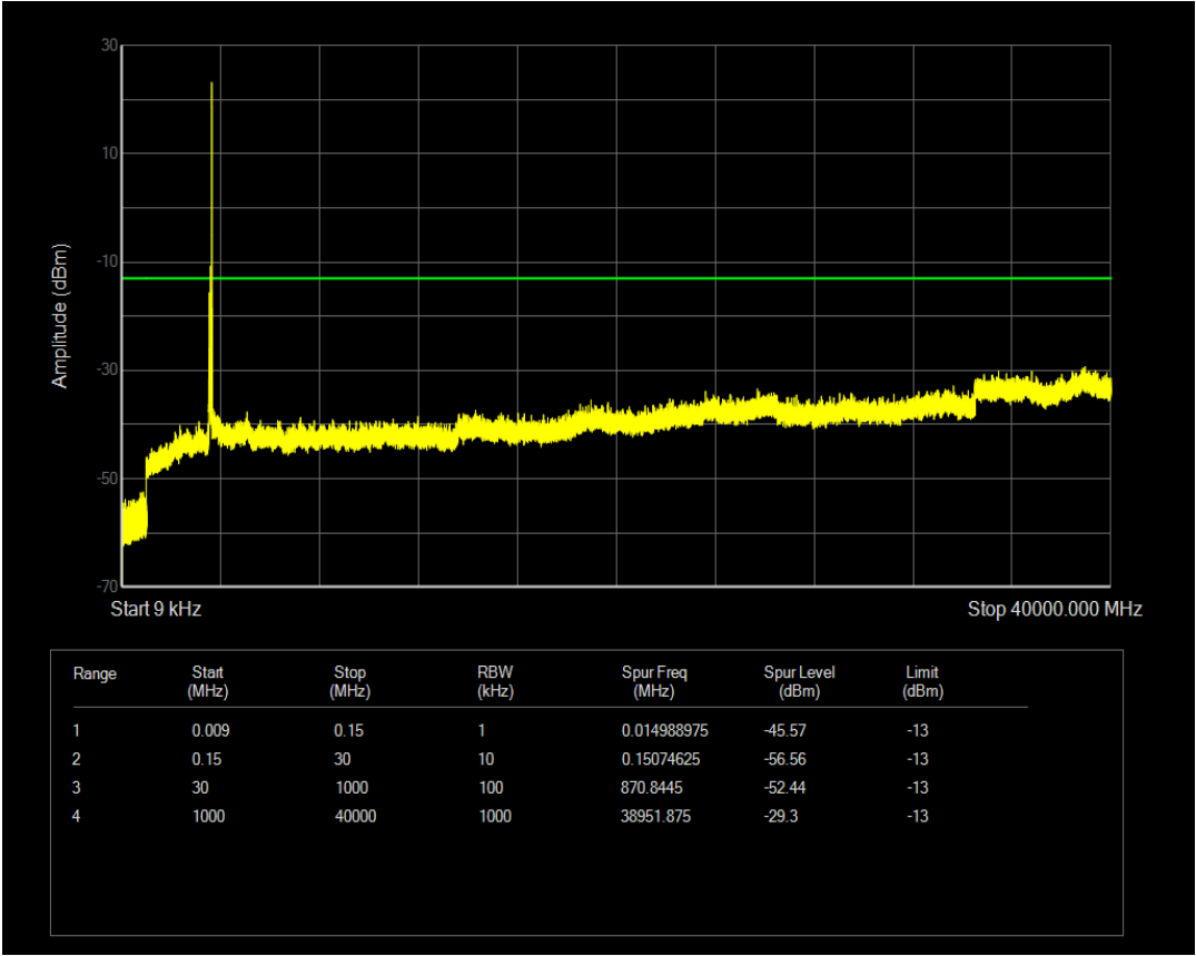
n77(3550-3700) SCS=30kHz CP_QPSK BW=100MHz Channel=640000 RB=1@0
